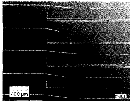
Fig. 2 Micrograph of part of test structure Waveguides between the lenses are used for identification purposes.
