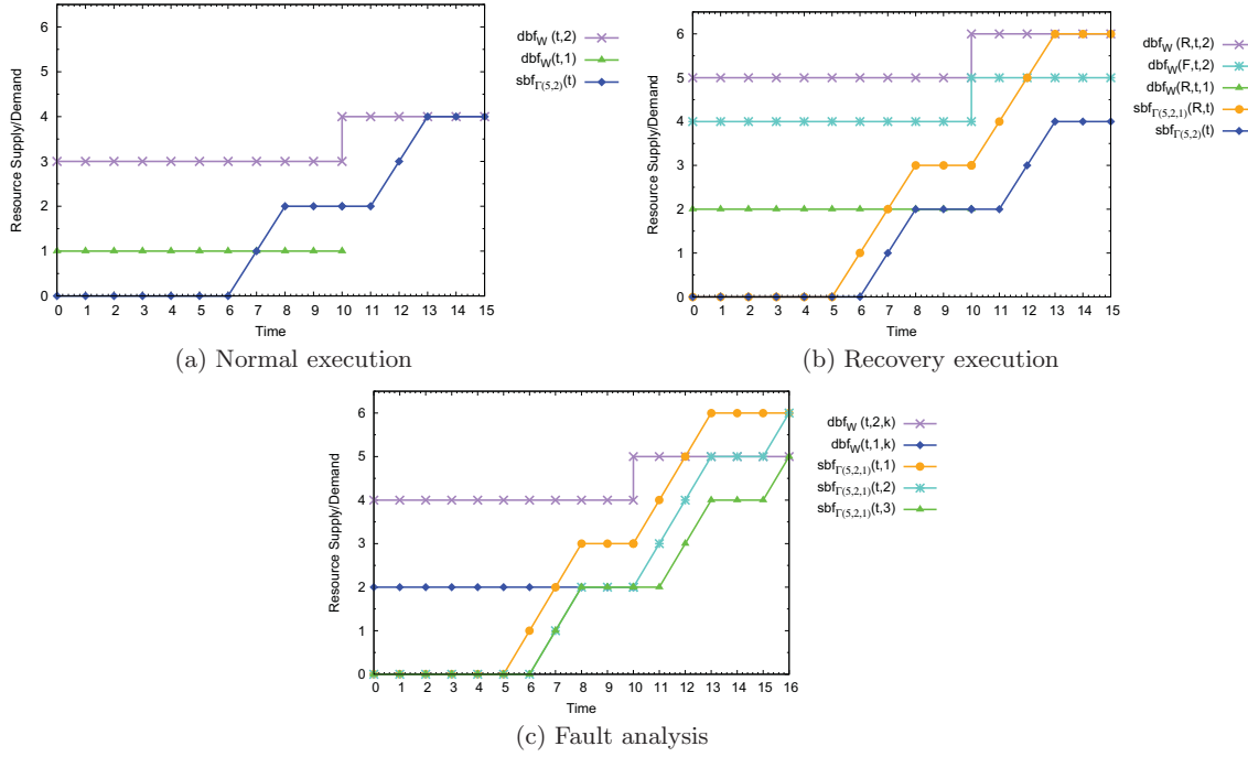
Figure 5: Schedulability analysis of Example 3.2
