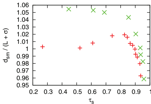
FIG. 4. The smectic layer-to-layer distance, d_{sm} , in the smectic phase as a function of smectic order parameter \tau_s , obtained from compression simulations for L/L_p = 0.31 (red pluses) and L/L_p = 0.09 (green crosses). Here, L_p , L , and L + \sigma are the persistence length, the contour length, and the total length of an isolated particle, respectively, with \sigma being the diameter of our beads. Because the particles compress slightly at high pressures corresponding to large values of the smectic order parameter d_{sm}/(L + \sigma) can be smaller than unity even though in reality d_{sm} is in that case virtually equal to the actual rod length.
