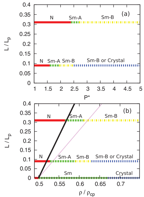
FIG. 1. Phase diagram of our filamentous particles for three values of the length-over-persistence-length ratios LL_p = 0.31, 0.09 , and 0 as a function of (a) reduced pressure, P^* and (b) reduced volume density \rho/\rho_{cp} where \rho_{cp} is the closed packed density for our particles. The red solid line and the green dashed line indicate the range in which the nematic and smectic-A phases are stable, respectively. The blue dotted line shows the region where the smectic-B or crystalline phases are stable and the yellow dotted-dashed line indicates the range in which the smectic-B phase is stable. The black solid line and purple dotted line correspond to theoretical predictions for nematic-smectic-A transition for \beta = 0.0235 and S_2 \approx 0.84 and 0.9 , respectively. See the main text.
