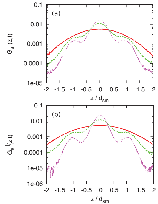
FIG. 9. Self part of the Van Hove function parallel to the director, G_s^{\parallel}(z, t = 1000t^*) , as a function of the scaled distance, z/d_{sm} , for particles (a) with L/L_p = 0.31 at P^* = 2.1 (red solid line), 2.5 (green dashed line), and 2.6 (purple dotted line) and (b) with L/L_p = 0.09 at P^* = 1.3 (red solid line), 1.6 (green dashed line), and 1.8 (purple dotted line). Here, d_{sm} is the layer-to-layer spacing of the smectic phase. For both L/L_p = 0.31 and 0.09, the lowest value of the pressure corresponds to a nematic phase state point in which case d_{sm} is set equal to a single particle length.
