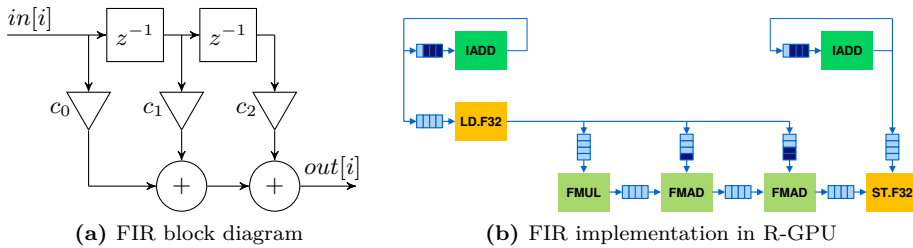
Figure 7.4: Block diagram of a 3-tap FIR filter (a) and an R-GPU implementation (b). Two cores (IADD) are calculating addresses, three cores (FMUL and FMADD) are performing calculations on data and two load-store units (LD and ST) are used.
