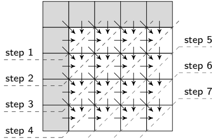
Figure 7.8: Dependencies between matrix elements in the Needleman-Wunsch algorithm. Seven steps are required to calculate this 4 \times 4 matrix.
