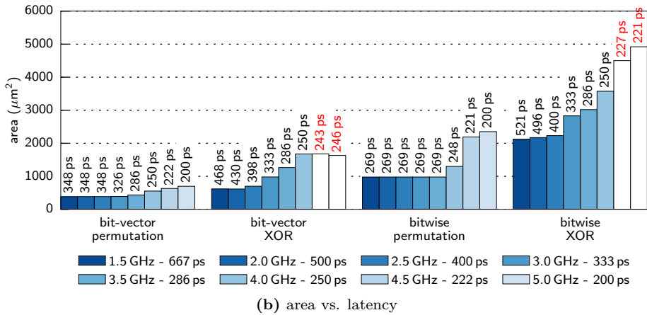
Figure 6.4: Power (a) and area (b) vs. latency results for the four proposed hash functions for a range of target clock frequencies (1.5 GHz – 5.0 GHz)
