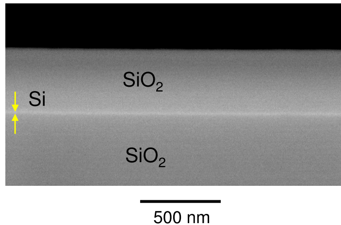
Fig. 5. (a) Side view image, made with a scanning electron microscope, of an a-Si thin film sputtered onto a \text{SiO}_2 substrate and covered by a \text{SiO}_2 layer.
