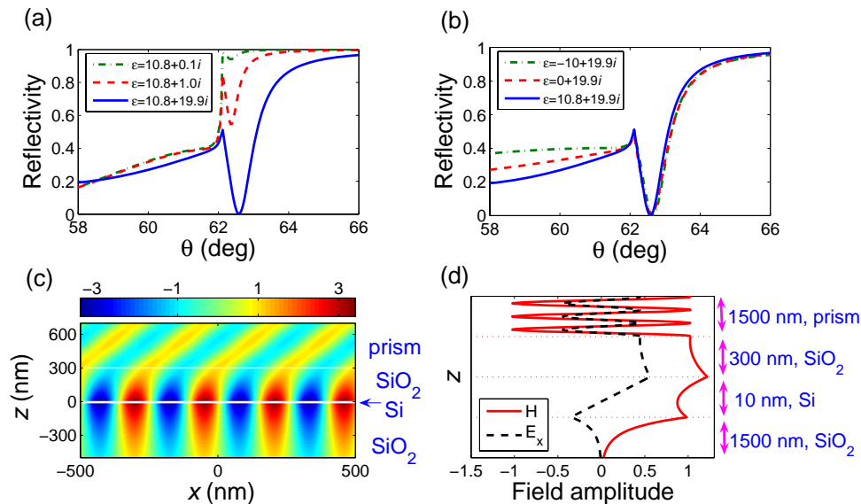
Fig. 8. (a) and (b) display the reflectivity at \lambda_0 = 375 nm of a sample formed by a prism ( n_{\text{prism}} = 1.67 ) on top of a SiO 2 layer with a thickness of 300 nm, an a-Si layer with a thickness of 10 nm and a SiO 2 substrate ( n = 1.48 ). The reflectivity is calculated for different values of the imaginary part (a) and the real part (b) of the permittivity of the thin layer. The full blue curves in (a) and (b) are calculated for \epsilon = 10.8 + 19.9i , i.e., the dielectric constant of a-Si at \lambda_0 = 375 nm. In figure (a) \epsilon = 10.8 + 1.0i (red dashed curve) and \epsilon = 10.8 + 0.1i (green dot-dashed curve). In figure (b) \epsilon = 0 + 19.9i (red dashed curve) and \epsilon = -10 + 19.9i (green dot-dashed curve). (c) Calculation of the magnetic field amplitude for a p -polarized beam ( \lambda_0 = 375 nm) incident at 62.9^\circ onto the sample with the same dimensions as in (a) and (b). Magnetic field amplitude (red full curve) and x -component of the electric field (black dashed curve) at x = 0 are shown in (d). Note that, for clarity, the SiO 2 layer and the silicon film are scaled.
