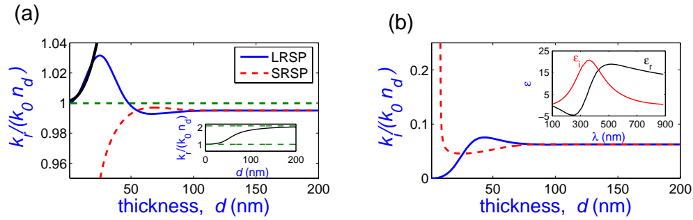
Fig. 2. (a) real k_r and (b) complex k_i components of the wave number of long-range surface polaritons (blue solid curves) and short-range surface polaritons (red dashed curves) in a-Si films at \lambda_0 = 318 nm as a function of the thickness of the film. The film is surrounded by a dielectric with a refractive index n_d = \sqrt{\epsilon_d} = 1.45 . k_r and k_i are normalized to the wave number in the surrounding dielectric. The black curve and the inset in (a) represent the normalized wave number of the TM_0 mode in a non-absorbing thin film surrounded by a medium with n_d = 1.45 . Inset of (b): wavelength dependence of the real (black curve) and imaginary (red curve) components of the permittivity of a-Si.
