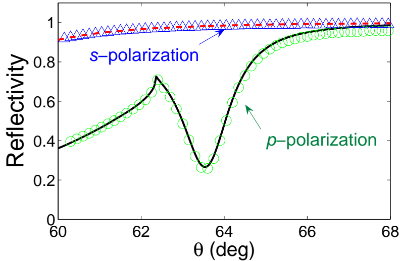
Fig. 7. Experimental (open circles and triangles) and theoretical (curves) reflectivity at \lambda_0 = 375 nm of the system formed by F2 glass, a \text{SiO}_2 layer with a thickness of 345 nm, an a-Si layer with a thickness of 13 nm and a \text{SiO}_2 substrate. The green circles and solid black curve correspond to p -polarized light, while the blue triangles and red dashed curve correspond to s -polarized light.
