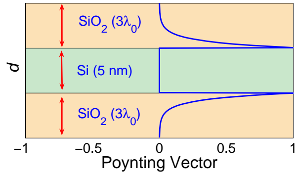
Fig. 4. LRSP's Poynting vector component tangential to an a-Si thin-film. The thickness of the a-Si is d = 5 nm with permittivity \epsilon = 18.5i at \lambda_0 = 318 nm, and the background is \text{SiO}_2 . Note that, for clarity, the scales for the \text{SiO}_2 layer and the a-Si film are different.
