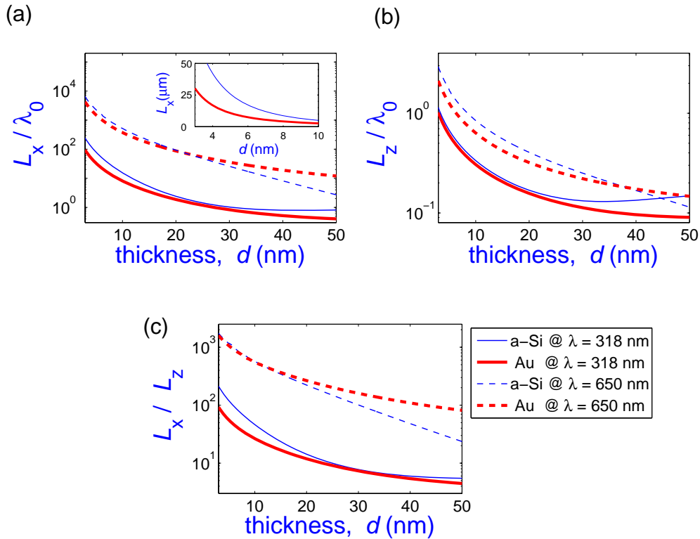
Fig. 3. (a) LRSP propagation length L_x normalized by \lambda_0 in a film of thickness d of gold (thick red curves) and silicon (thin blue curves) surrounded by a dielectric with refractive index n_d = 1.45 . The solid curves correspond to \lambda_0 = 318 nm, while the dashed curves are the calculations for \lambda_0 = 650 nm. The inset represents a close view of L_x at \lambda_0 = 318 nm for small values of d . (b) decay length of the field intensity L_z (normalized by \lambda_0 ) in the dielectric for the same materials and wavelength as in (a). (c) Figure of merit of thin-film guiding structures defined as L_x/L_z for the same materials and wavelengths as in (a).
