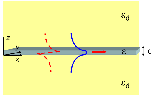
Fig. 1. Schematic representation of the electric field component along the x -direction of a long-range (red dashed curve) and of a short-range (blue solid curve) surface polariton in a thin layer of a material of permittivity \epsilon surrounded by a dielectric of permittivity \epsilon_d .
