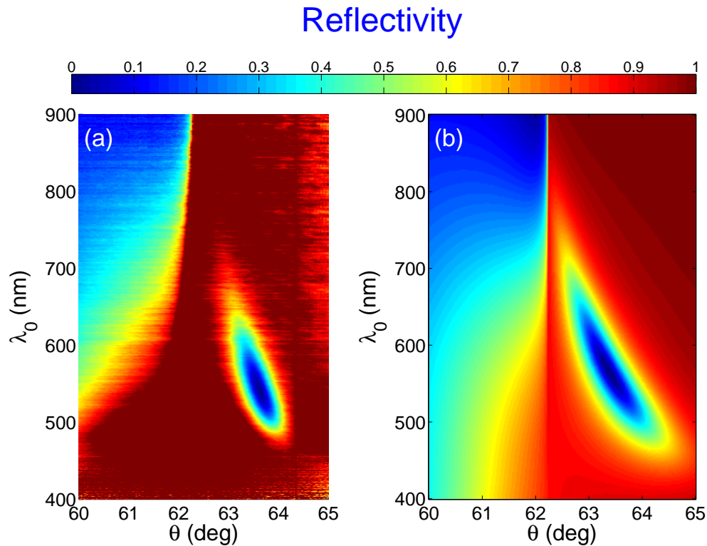
Fig. 6. (a) Measurements and (b) calculations of the reflected spectra of p -polarized light incident at an angle \theta on the system formed by F2 glass, a SiO 2 layer with a thickness of 500 nm, a 20 nm layer of a-Si and a SiO 2 substrate.
