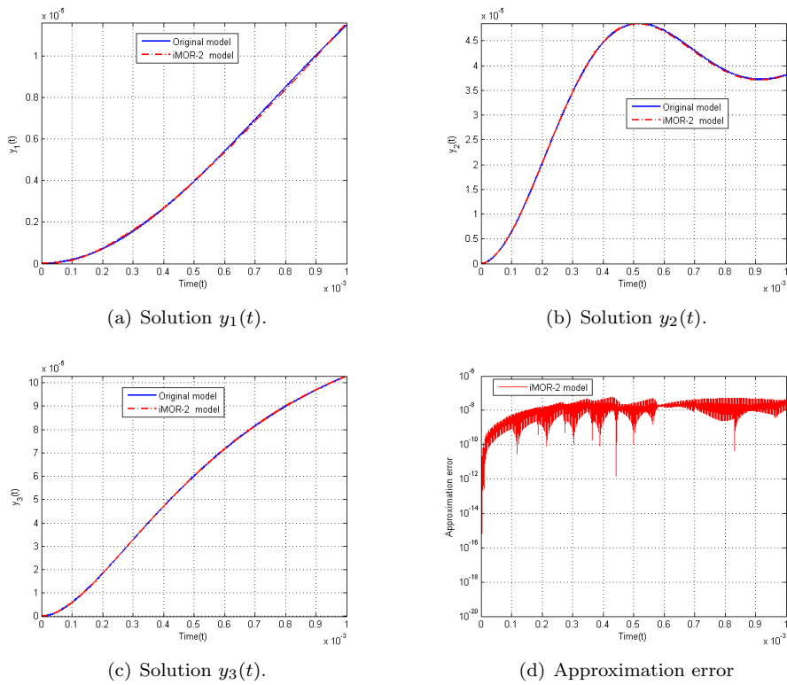
FIG. 4.19. Example 7. Solutions and their approximation error.
