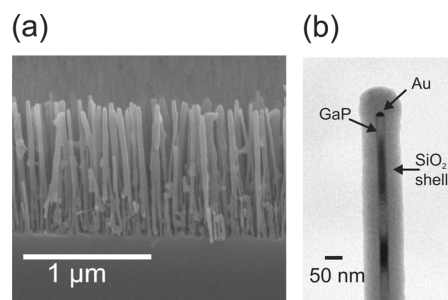
FIG. 1. (a) Cross-sectional SEM image of a sample of GaP nanowires. (b) TEM image of a nanowire covered with a thin shell of SiO 2 .
