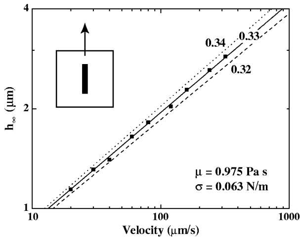
FIG. 3. Dependence of the height of entrained liquid lines on the speed of withdrawal U . The solid line represents a power law relation h_\infty \sim U^\beta with \beta=0.33 . The dashed and dotted lines represent equivalent power law relations with exponents 0.32 and 0.34, respectively.
