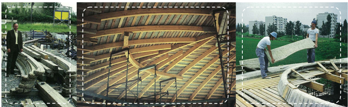
Figure 6: formwork system by Heinz Isler 6
