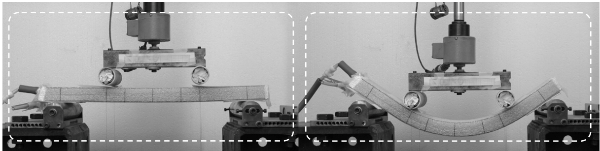
Figure 10: large bending deformations of Vacuumatics
