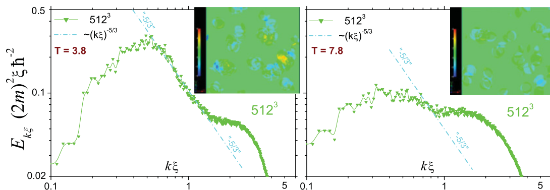
FIG. 1. (Color online) The incompressible energy spectra at time T = 3.8 (left) and T = 7.8 (right). The color insets show vorticity two-dimensional slice maps (see text for the definition). The grid size is 512^3 and \Lambda \simeq 1.5 .
