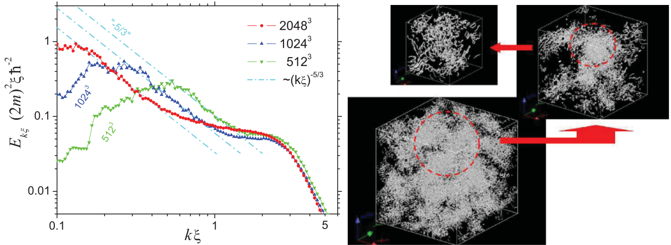
FIG. 2. (Color online) Left: Simulation results of the incompressible energy spectra E(k\xi) normalized by \hbar^2/(4m^2\xi) . Symbols: 2048^3 (—•—), 1024^3 (—▲—), 512^3 (—▼—). \Lambda varies from \Lambda \simeq 1.5 (slightly depending on time) for 512^3 to \Lambda \simeq 2.2 for 2048^3 . Dot-dashed (cyan) line: K41 “ -5/3 ” scaling. Right: A snapshot of vortex lines at the fully developed turbulent state of 2048^3 demonstrates the self-similarity of the bundle-vortex structure (see the dotted circles representing the zoomed regions whose vortex distributions are shown subsequently), typical for fully developed turbulence.
