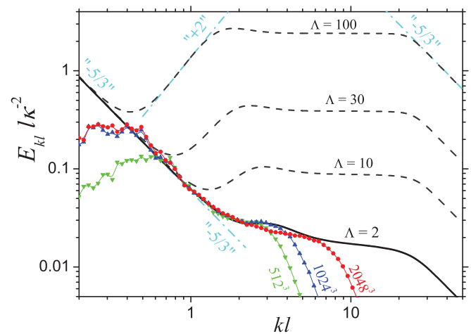
FIG. 3. (Color online) Incompressible energy spectra plotted vs kl\ell and normalized by \kappa^2/\ell . The simulation results (the same symbols) and the LNR model for \Lambda = 10, 30, 100 [dashed (black) curves] are brought together to the theoretical [solid (black)] curve with \Lambda = 2 by superposing the K41 (for both simulations and model) and plateau regions (only for simulations). Dot-dashed (cyan) lines show different scaling asymptotics.
