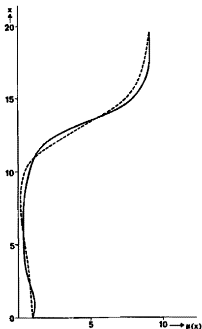
Figure 6.5 Solid line: the square of the refractive index for the 2.4 mode. Dashed line: the approximation by Rower's function.
