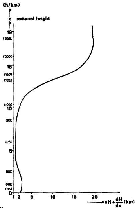
Figure 6.2. \kappa H + \frac{dH}{dx} versus the reduced height for the Mean Reference Atmosphere of CIRA 1972. The real height is given in parentheses.
