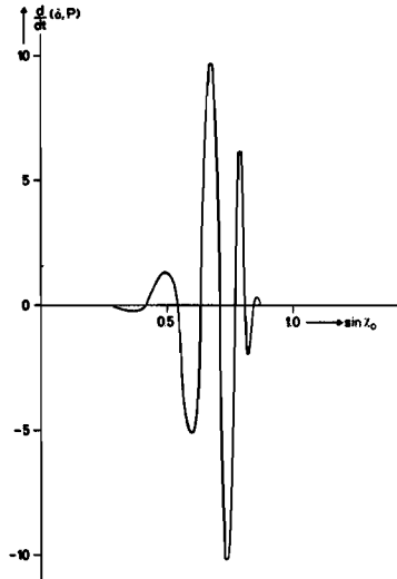
Figure 2.3 The frequency shift of a high-frequency signal as a function of the angle of incidence in the case of a wavelike perturbation in the electron density of the ionosphere.
