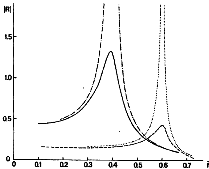
Figure 5.2 Variation of the absolute value of the reflection coefficient |R| , as a function of the ratio \hat{f} between the angular velocity f and the wave frequency \omega . Conventions as in the previous figure.
