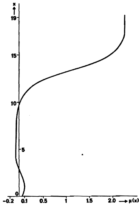
Figure 6.3. The value of the square of the refractive index for the 2.2 mode versus the reduced height.
