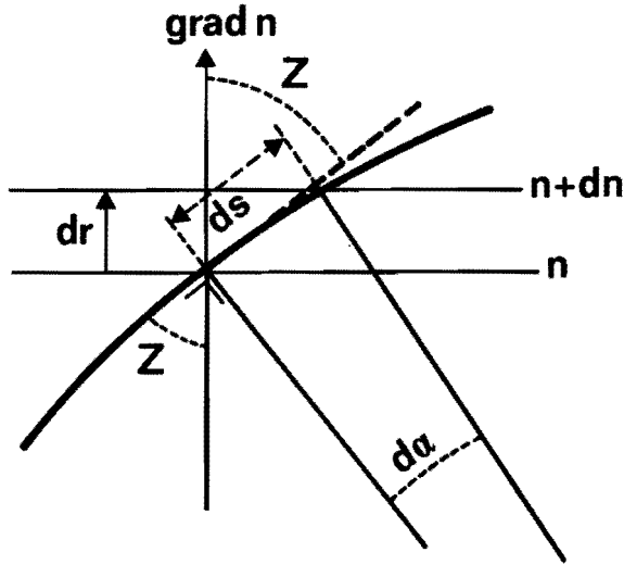
Figure 2.1 The relation between the curvature and the angular refraction of a ray in a medium with a gradient in the refractive index (Snel's law).
