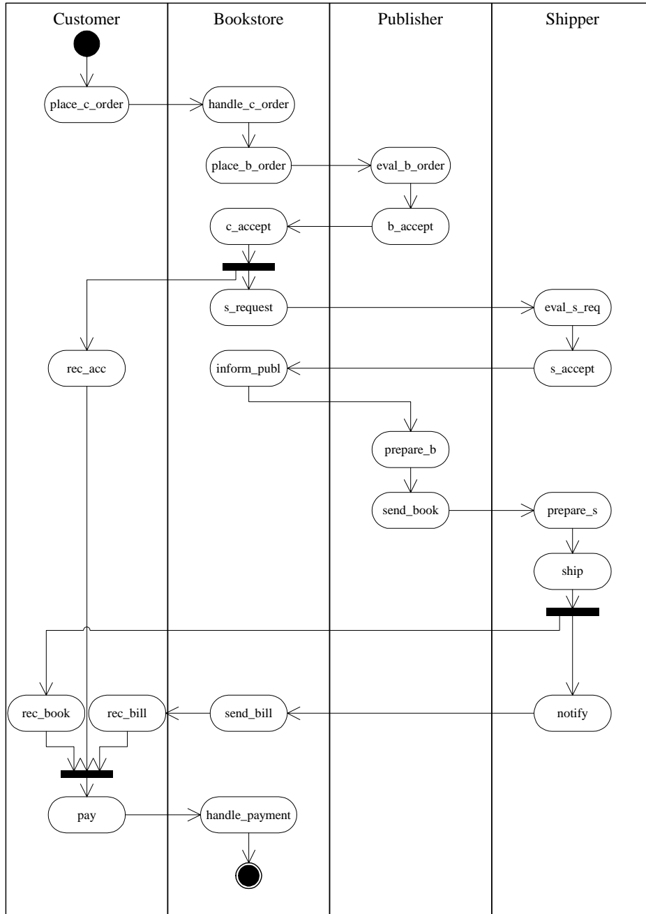
Figure 5. Typical order flow for an electronic bookstore.
