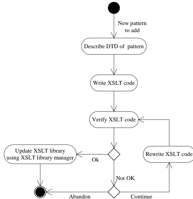
Figure 3. Adding a new template to the library.
