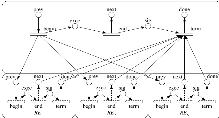
Figure 15. Semantics of parallel_no_sync .
