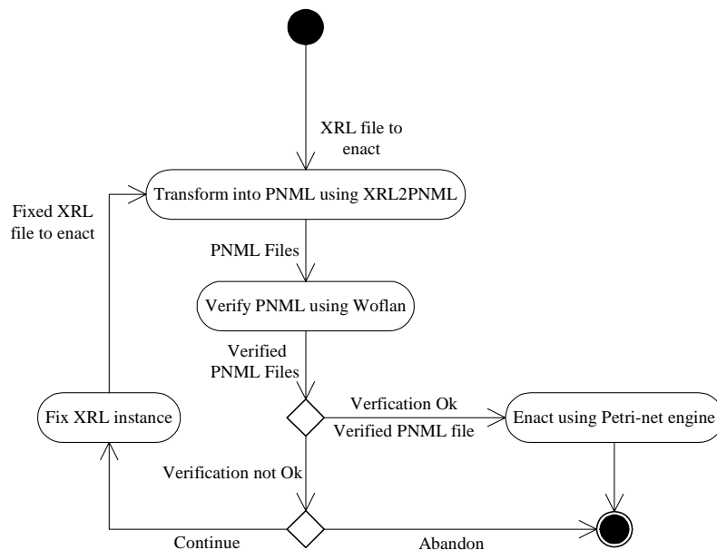
Figure 2. Transformation from XRL to PNML.
