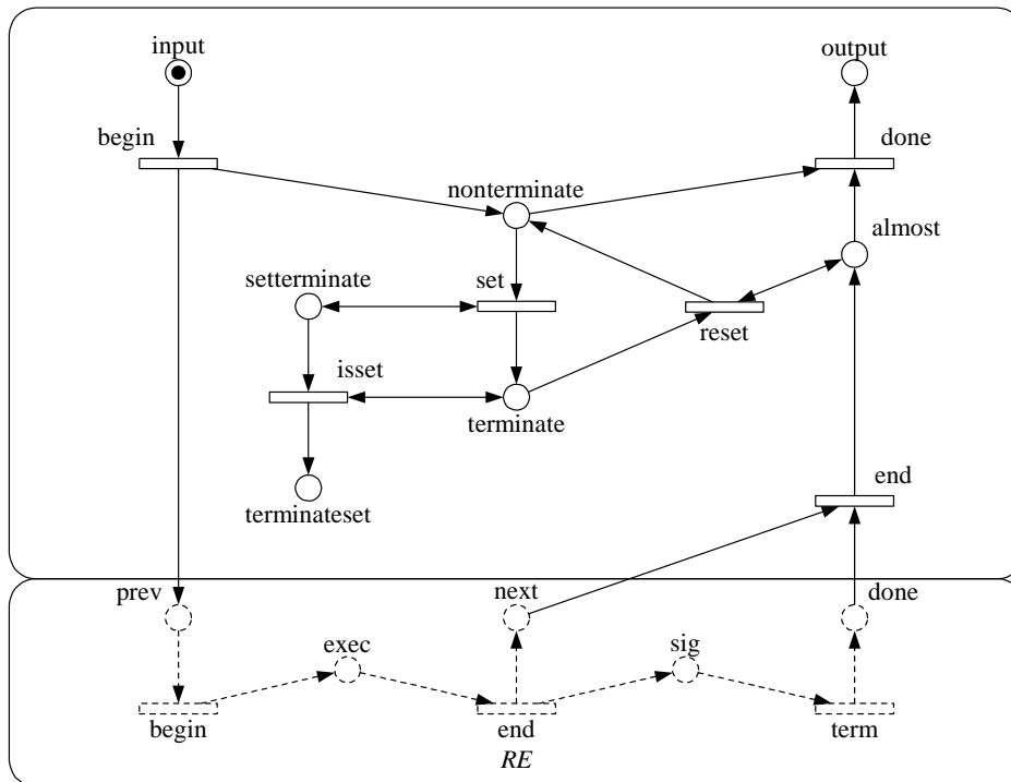
Figure 7. Semantics of route.
