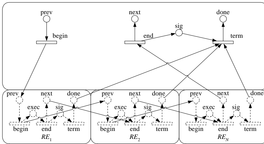
Figure 25. Semantics of fast_sequence .
