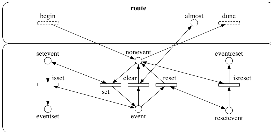
Figure 27. Semantics of event on global level after extending event.
