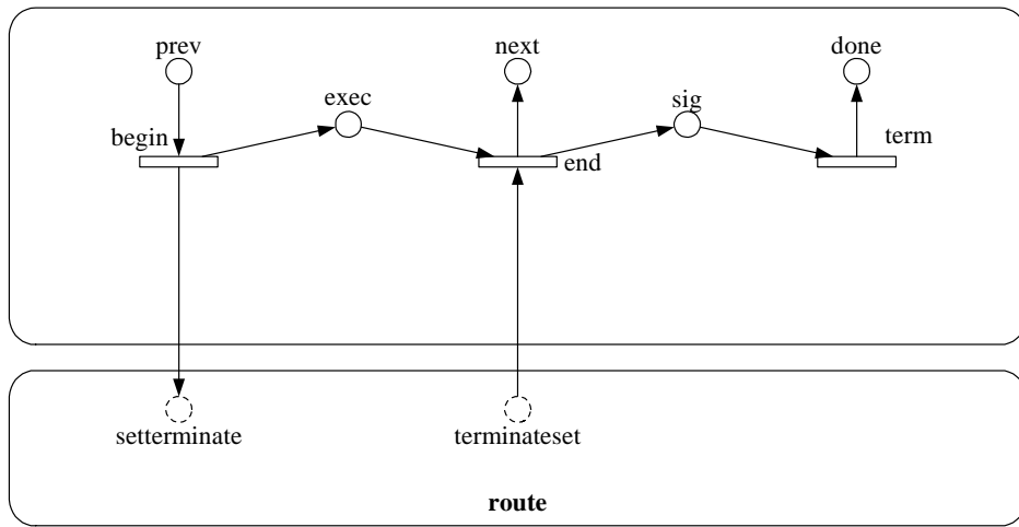
Figure 21. Semantics of terminate.
