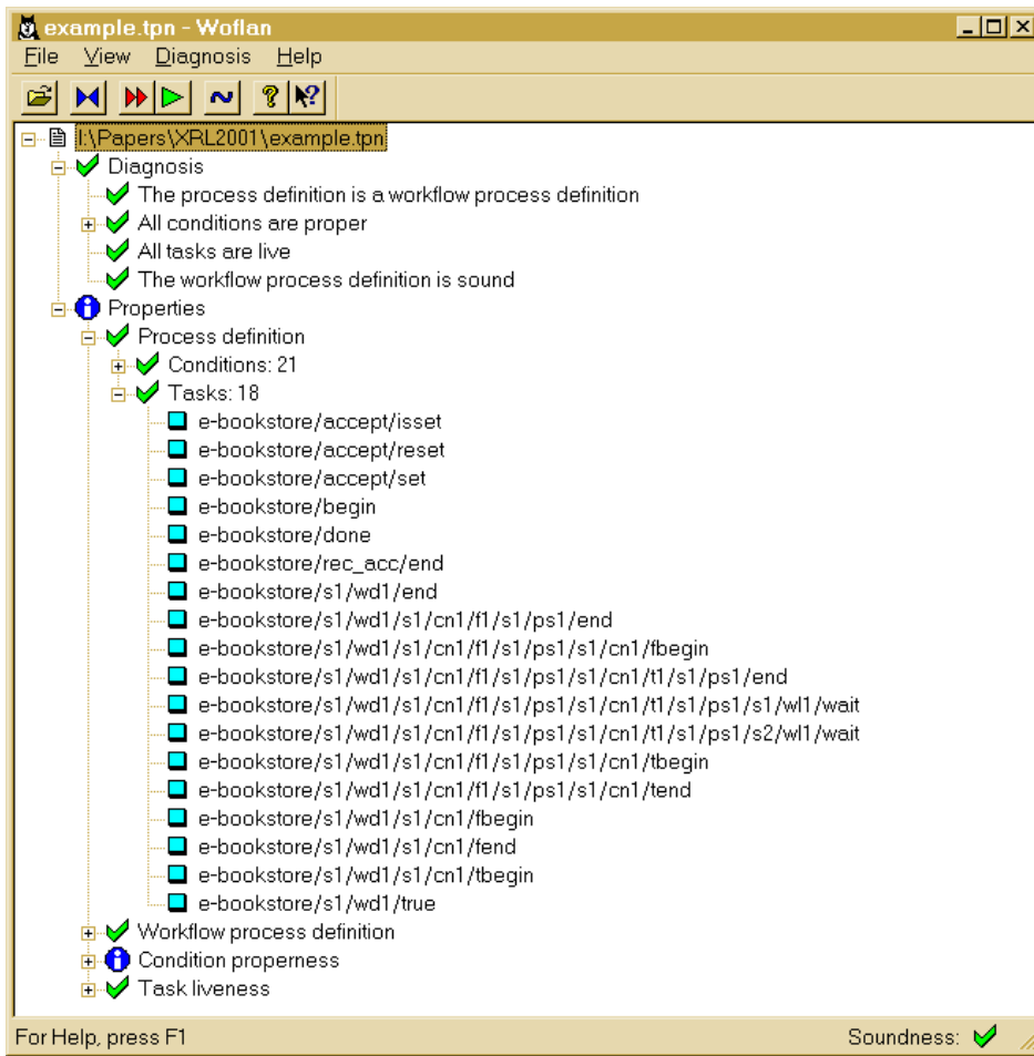
Figure 30. Woflan screendump.
