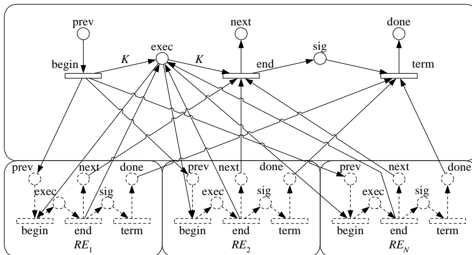
Figure 24. Semantics of restricted_parallel_sync .
