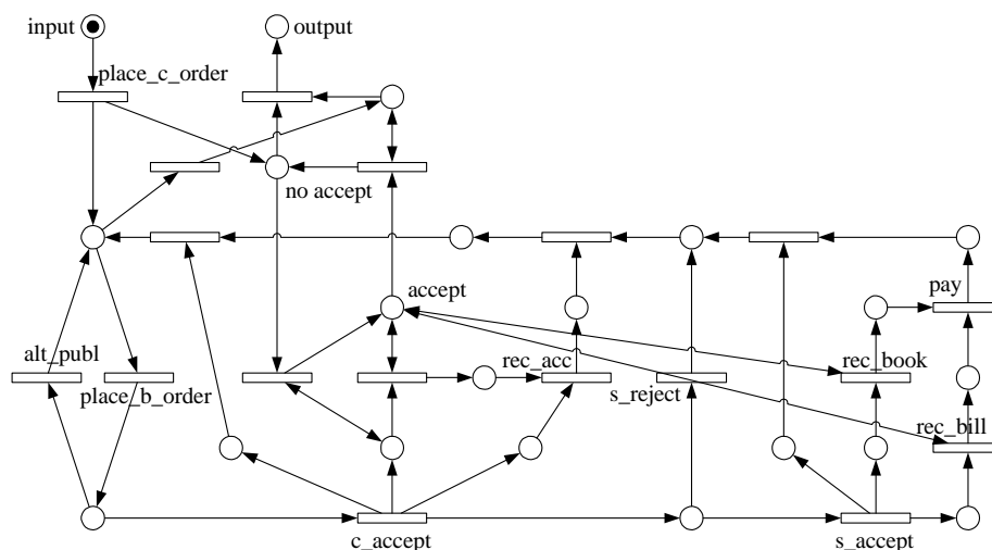
Figure 23. The WF-net corresponding to the example XRL route in Section 3 after both reductions.
