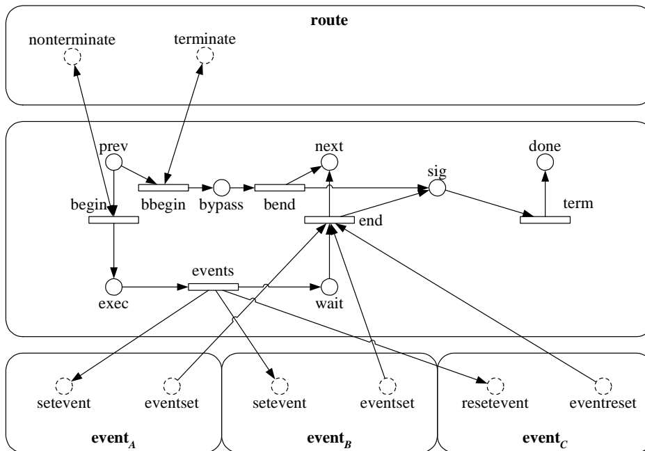
Figure 26. Semantics of task after extending event.
