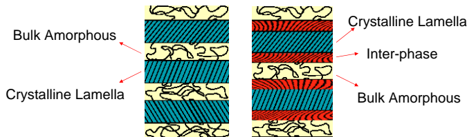
Figure 2: Schematic of the two-phase and three-phase models
