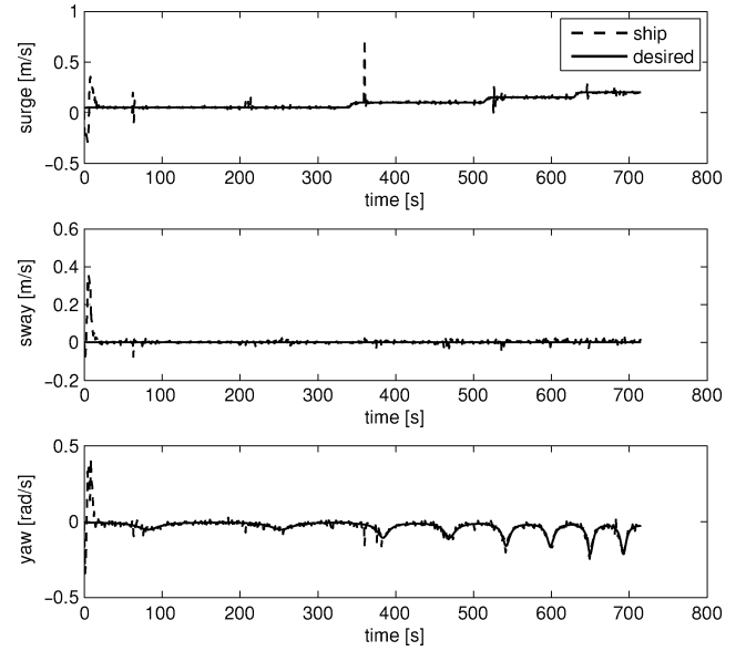
Fig. 4. Desired velocity u_{\text{ref}} , v_{\text{ref}} , and r_{\text{ref}} and ship velocity u , v , and r estimated by the numerical differentiator. The surge velocity increases at t = 345 , t = 520 , and t = 635 .
