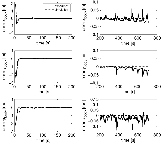
Fig. 3. Position errors of the observer-controller scheme: e_{x\text{body}} , e_{y\text{body}} and e_{\psi} for both simulation (dashed line) and experiment (solid line).
