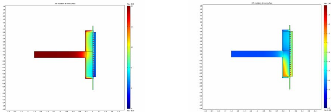
FIG. 8: variant 4, inside surface insulation with XPS
