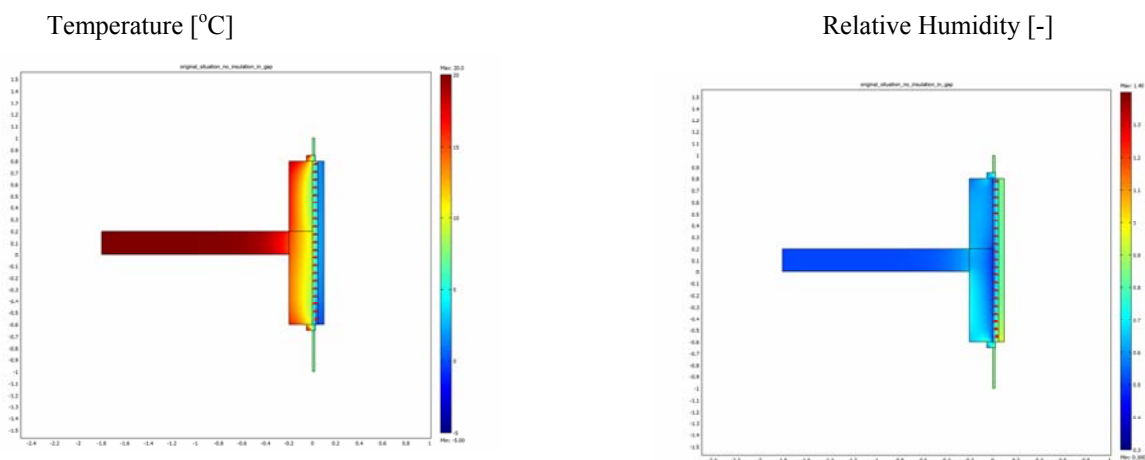
FIG. 5: variant 1, the original non insulated facade
