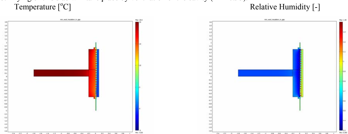
FIG. 6: variant 2, mineral wool in gap
