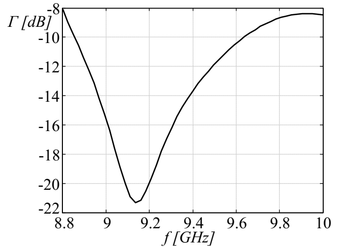
Fig. 3. Measured Input Reflection Coefficient.
