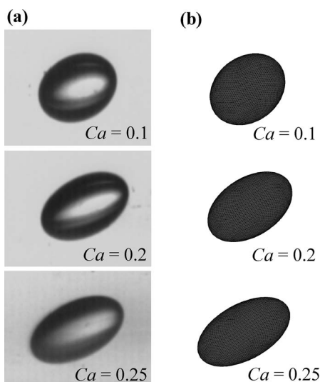
FIG. 3. Steady-state droplet shape in the velocity-velocity gradient plane at Ca=0.1, 0.2, and 0.25 for 2R/d=0.18 : (a) Experimental data and (b) numerical data.
