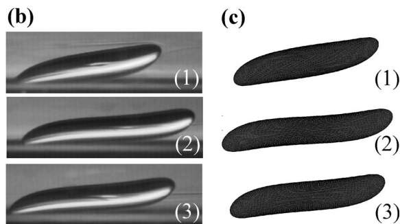
FIG. 11. Startup data at Ca=0.35 for 2R/d=0.88 . (a) Comparison between experimental and numerical droplet dimensions as a function of dimensionless time. (b) Experimental droplet shape and (c) numerical droplet shape at t^*= (1) 18.2, (2) 60.6, and (3) 135.5.
