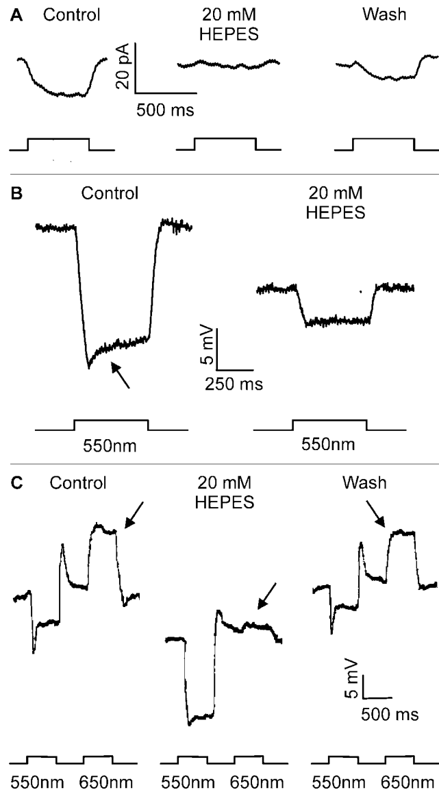
Figure 2. HEPES reduces feedback-mediated responses in the cone/horizontal cell network in the isolated retina of goldfish.
