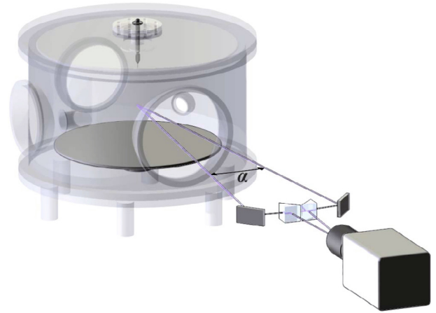
Fig. 2. (Color online) A stainless steel vessel of 50 cm diameter and 30 cm height is used to create a 16 cm gap in a controlled gas composition. The large side window offers the possibility to view the streamer under two angles. Details on the set-up and its pulsed power supply can be found elsewhere [1,14].
