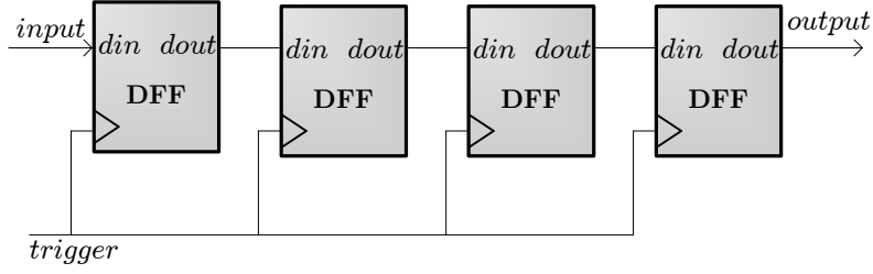
Figure 7: A simple shift register
