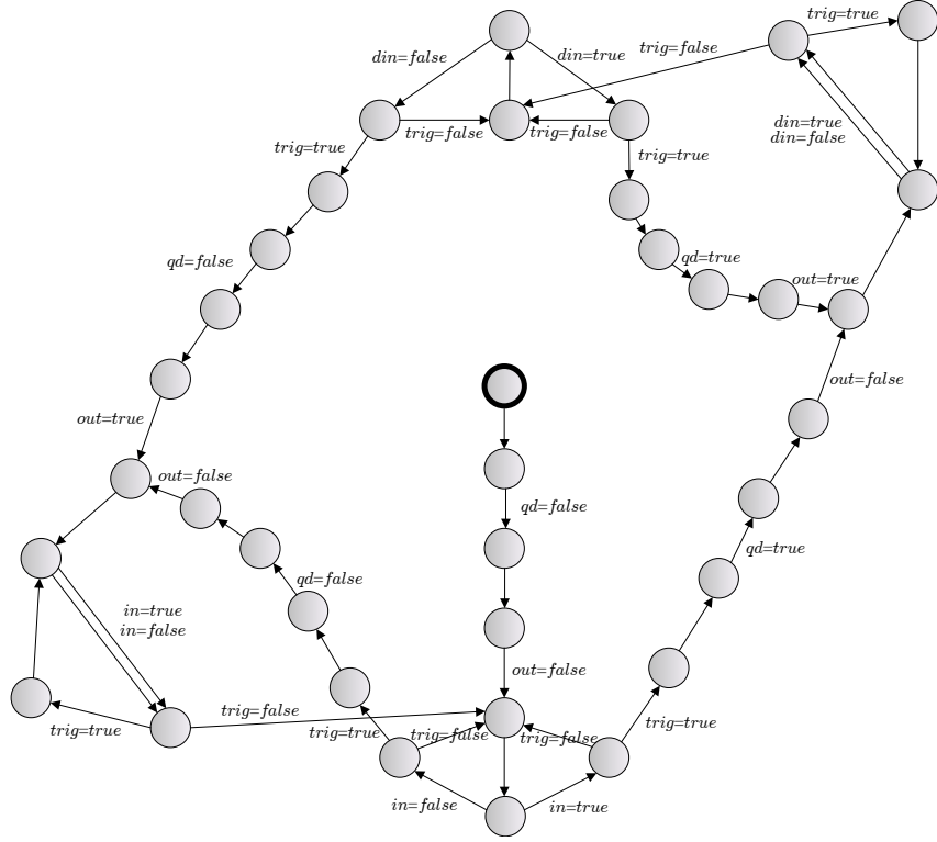
Figure 11: The state space of Figure 9 after tau-confluence reduction
