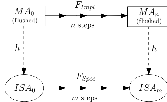
Figure 14: Burch and Dill's Commuting Diagram
