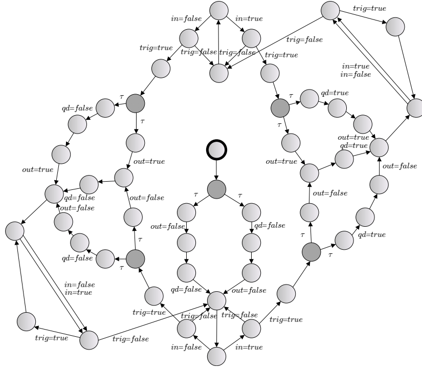
Figure 10: The state space of Figure 9 after branching bisimulation reduction
