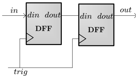
Figure 9: A two bit shift register
