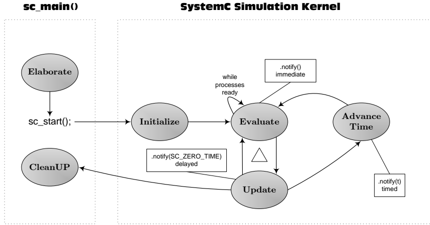
Figure 2: SystemC Simulation kernel ([4])
