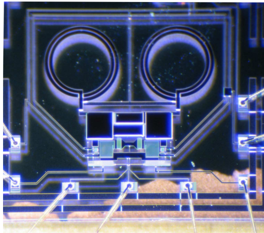
Figure 4.53 2 nd IC prototype silicon implementation
