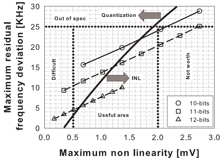
Figure 4.7 Effect of DAC INL on the residual frequency error
