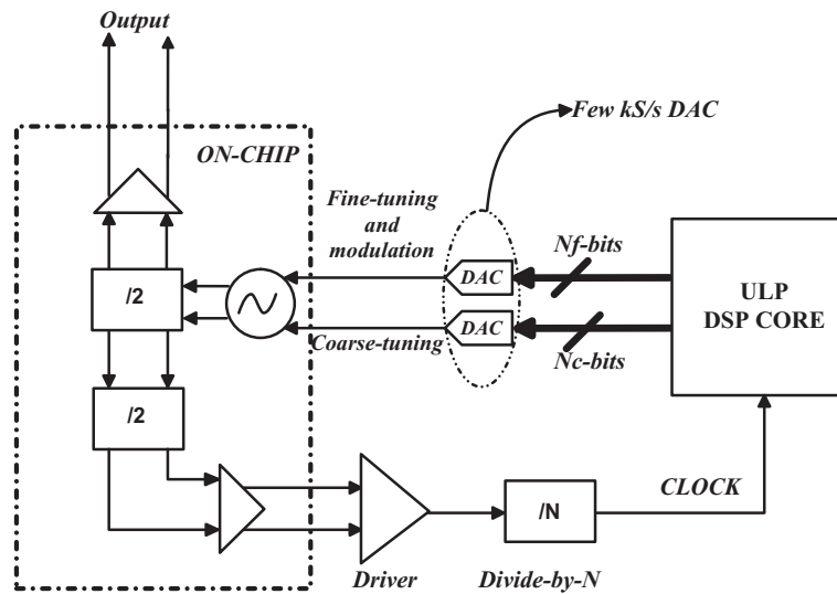
Figure 4.54 Schematic block diagram of the transmitter prototype
