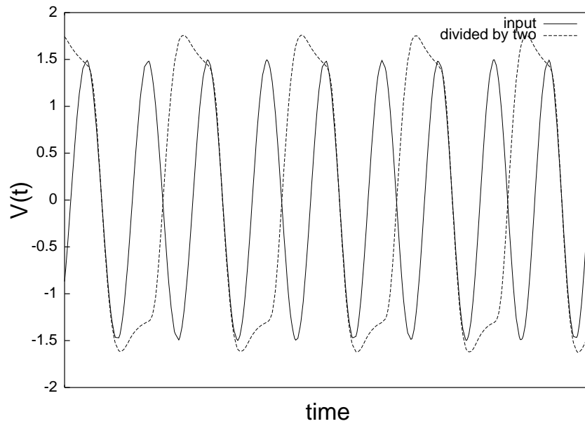
Figure 4.29 Input and output transient waveforms for the TWD
