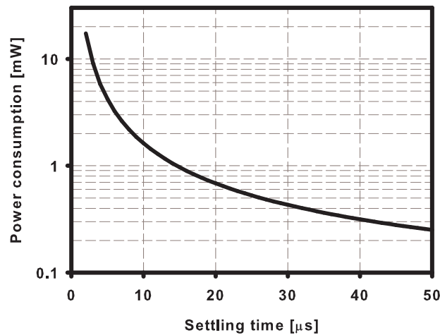
(b) Power consumption of the baseband PLL versus settling time
