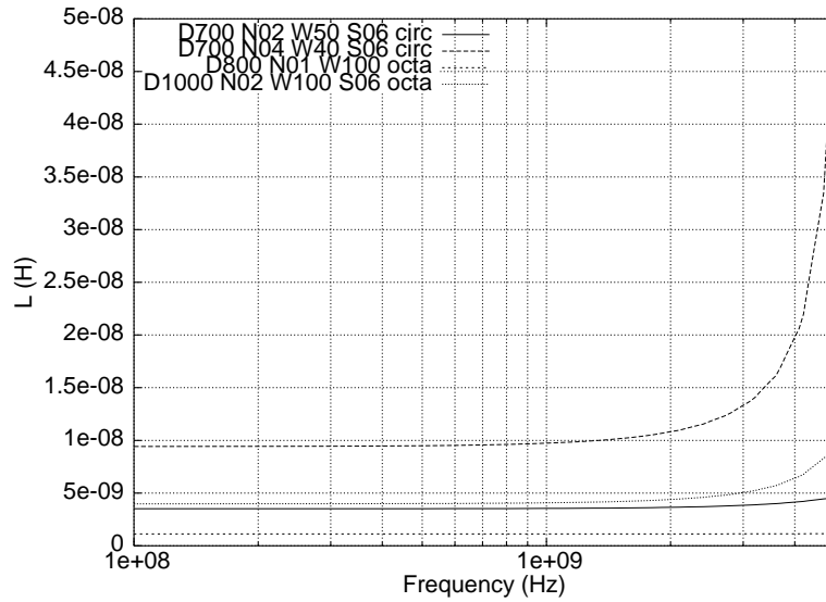
Figure 4.15 Inductance of coils as a function of frequency
