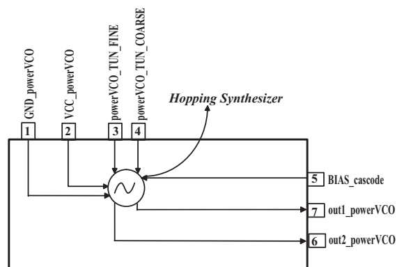
Figure 4.52 Block diagram of the 2 nd IC prototype
