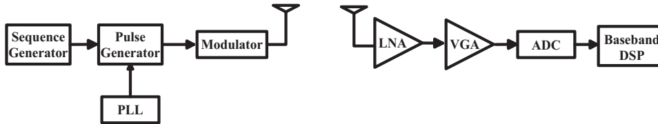
Figure 2.1 The building blocks of an impulse based UWB transceiver
