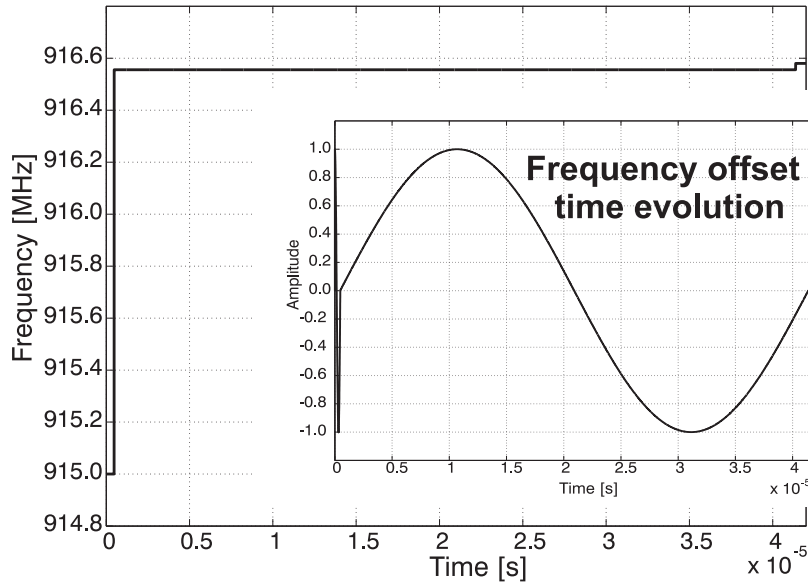
Figure 4.42 Receiver synthesized frequency vs. time
