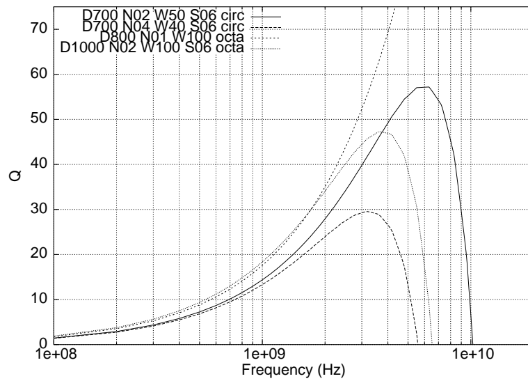
Figure 4.16 Q factor of coils as a function of frequency
