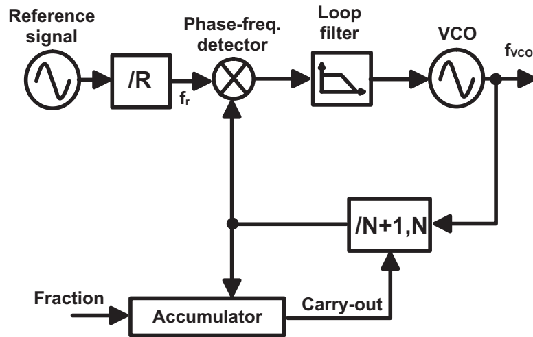
Figure 3.6 Fractional-N PLL block diagram
