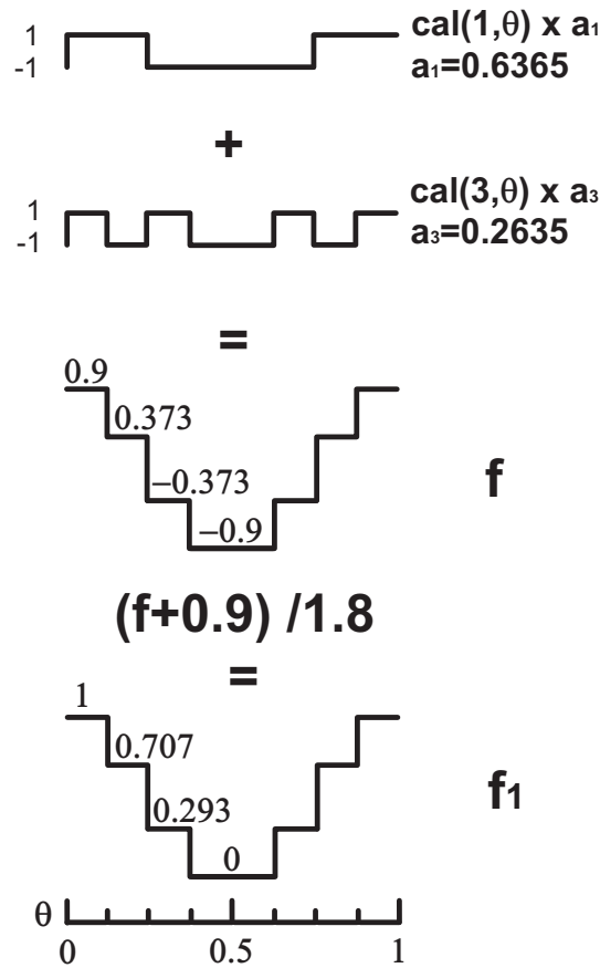
Figure 5.11 Synthesized function for n=3
