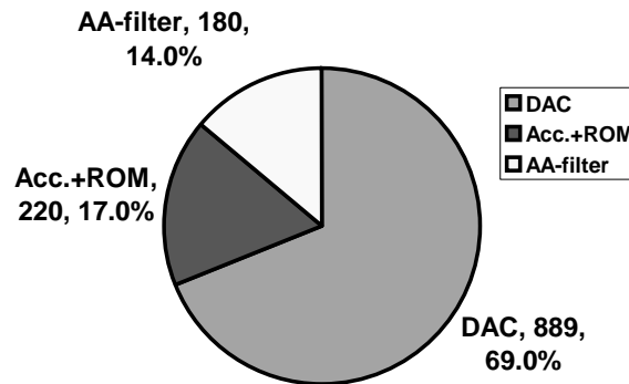
Figure 3.23 Power consumption break-down by block (power in \mu\text{W} )
