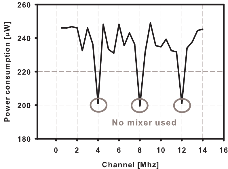
Figure 5.32 Measured power consumption versus the synthesized frequency
