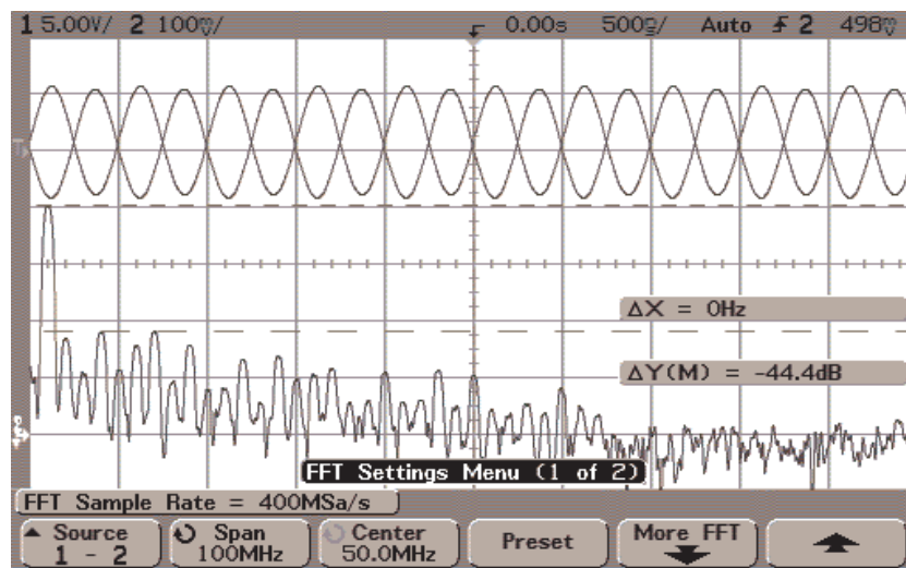
Figure 5.36 Spectrum of the differential signal output for a synthesized frequency of 2 MHz
