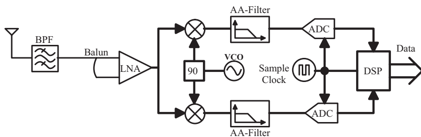
Figure 5.16 Proposed zero-IF receiver architecture
