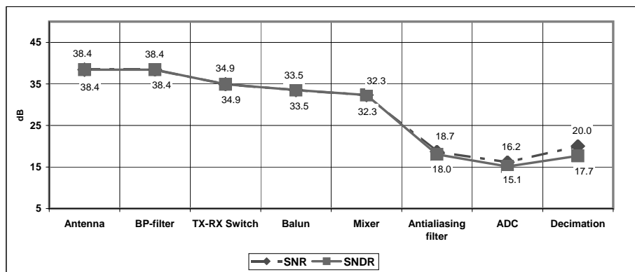
Figure 5.24 SNDR and SNR along the receiver chain with the input signal at the sensitivity level
