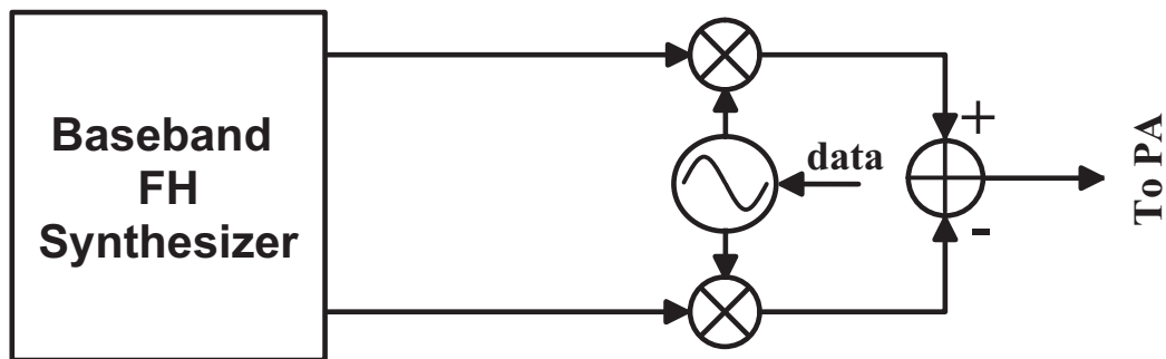
Figure 5.1 Transmitter architecture employing SSB direct up-conversion scheme
