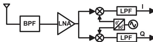
Figure 2.13 Zero-IF architecture
