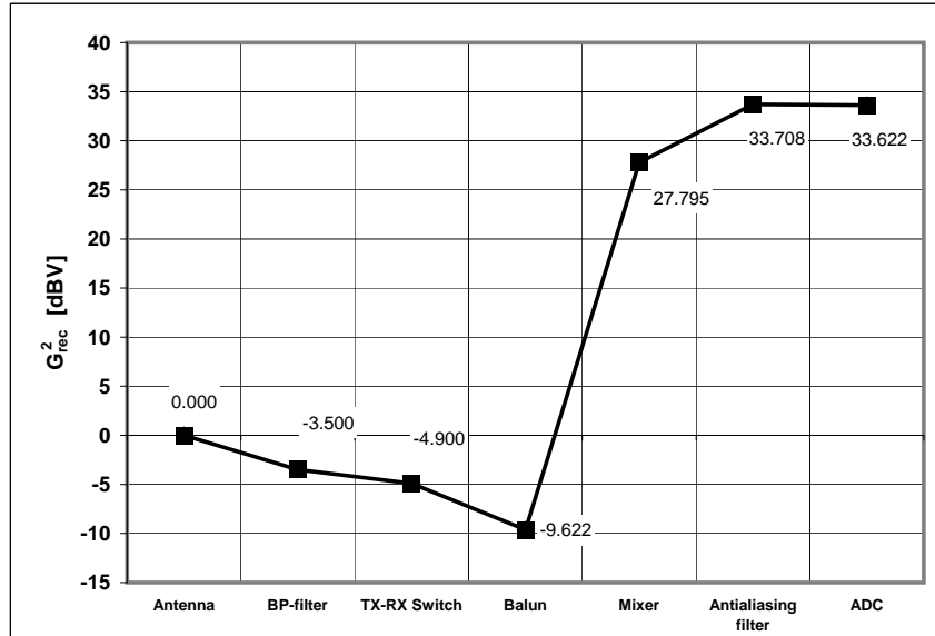
Figure 5.21 Gain distribution through the receiver chain
