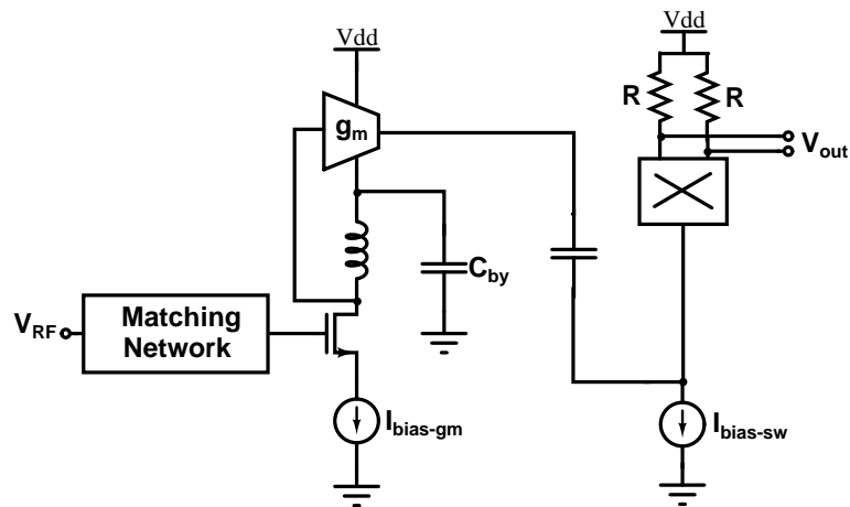
Figure 5.25 Current-reused folded-cascode LNA-mixer (from [126])
