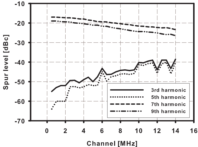
Figure 5.31 3 rd , 5 th , 7 th and 9 th harmonic levels below the fundamental versus synthesized frequency (prior to LP-notch filter)
