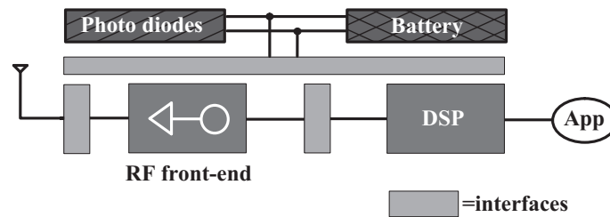
Figure 4.49 High level block diagram of the TX-only demonstrator
