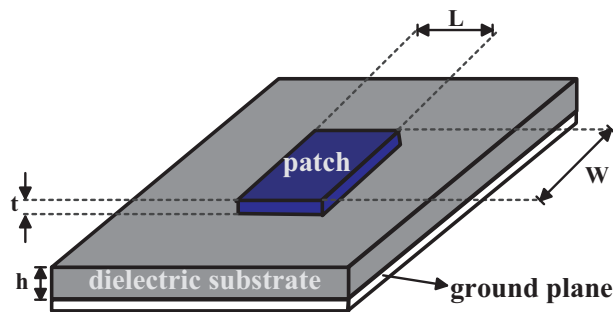
Figure 4.56 Structure of a microstrip patch antenna
