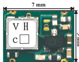
Figure 1.4 On Shine 433 MHz transmitter.
