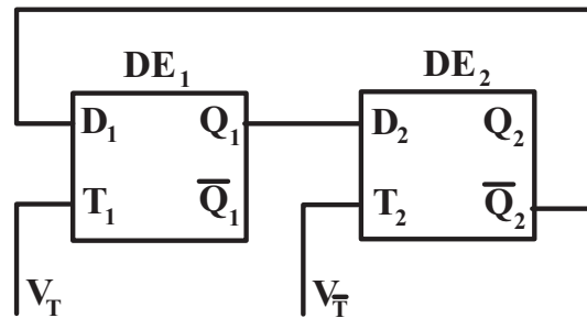
Figure 4.26 Block diagram of a binary divide-by-two frequency divider using the master-slave principle
