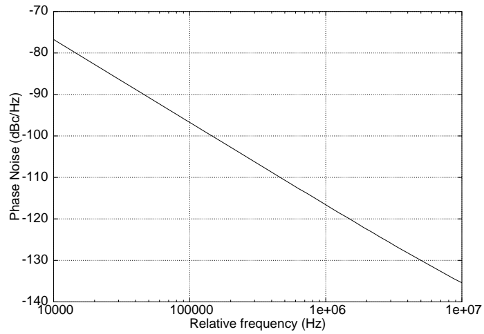
Figure 4.23 Phase noise plot for the topology with AC coupled cross-coupled pair
