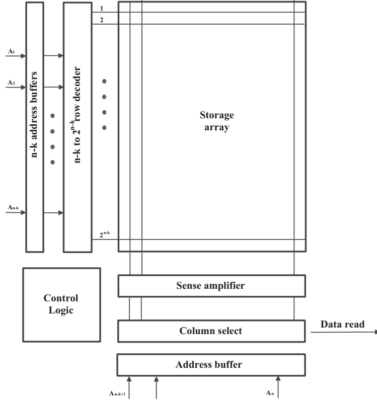
Figure 3.16 General memory structure
