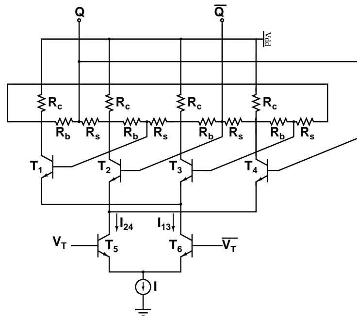
Figure 4.27 Travelling-wave divider schematic
