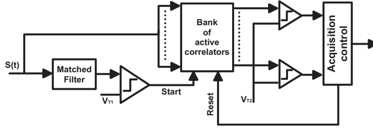
Figure 3.3 Two-step acquisition scheme adapted from [34]
