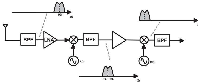
Figure 2.14 Super-heterodyne architecture
