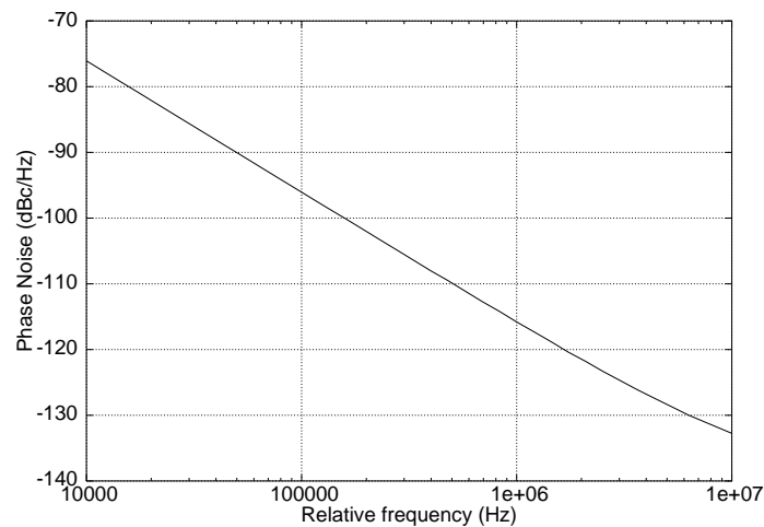
Figure 4.25 Phase noise plot of the topology biased via a current mirror
