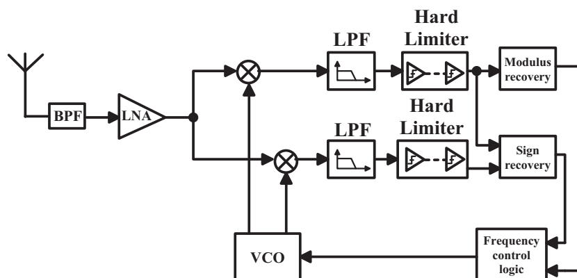
Figure 4.36 Direct-conversion architecture with frequency offset recovery circuitry
