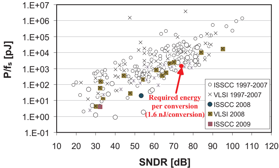
Figure 5.22 ADC performance survey 1997-2009 [125]
