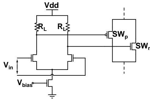
Figure 3.18 Switch driver schematic
