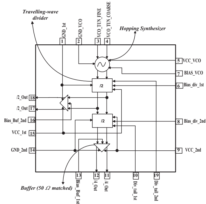
Figure 4.50 Block diagram of the 1 st IC prototype
