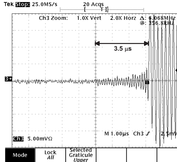
Figure 4.62 Oscillator start-up time for the power VCO based architecture
