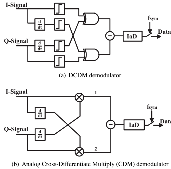
Figure 4.45 Cross-differentiate-multiplier demodulator
