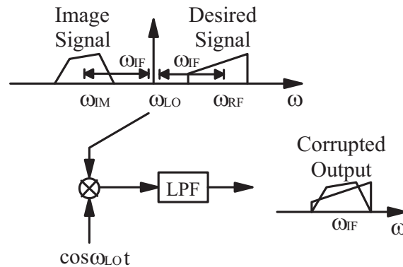
Figure 2.15 Image frequency problem
