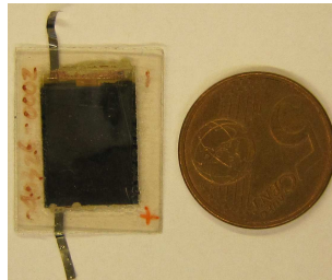
Figure 1.5 NanoEnergy battery from FrontEdge Technology, Inc.
