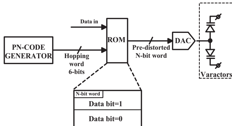
Figure 4.3 Frequency pre-distortion conceptual block diagram
