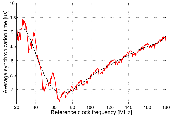
Figure 4.40 Average acquisition time vs. reference clock frequency
