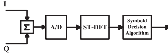
Figure 4.46 ST-DFT demodulator
