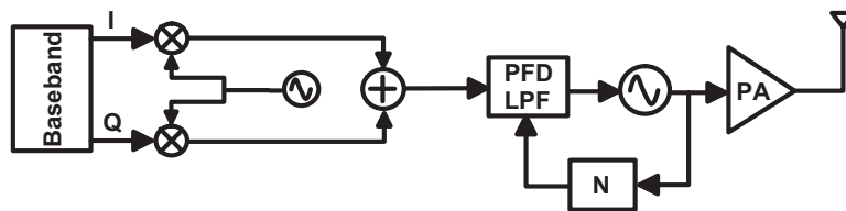
Figure 2.12 Offset PLL architecture
