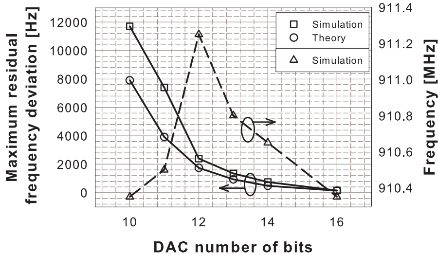
Figure 4.6 Maximum uncorrected frequency error and its position in the frequency band versus DAC number of bits
