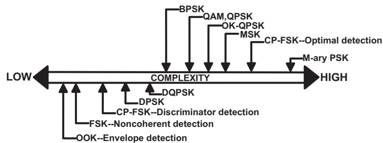
Figure 2.6 Relative complexity of various modulation scheme (adapted from [29])
