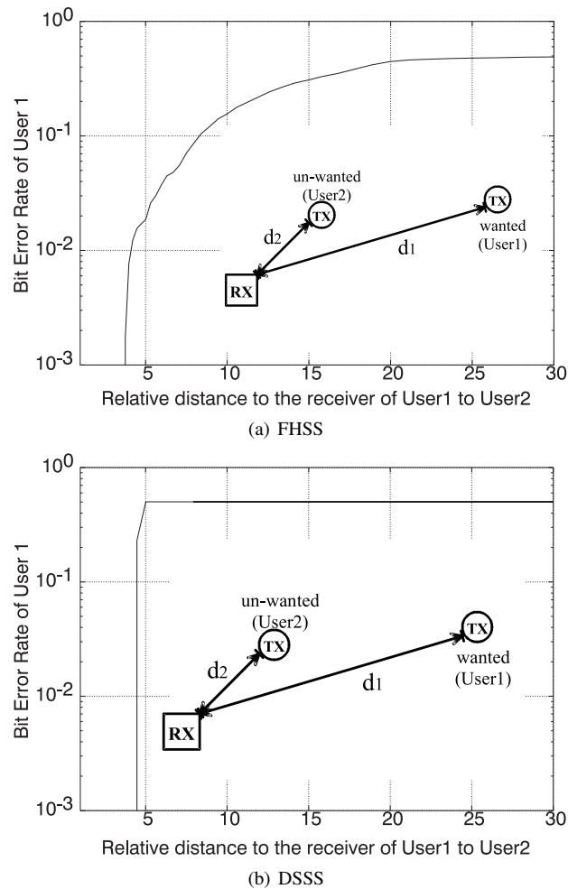
Figure 2.4 Near-far sensitivity comparison between FHSS and DSSS.
