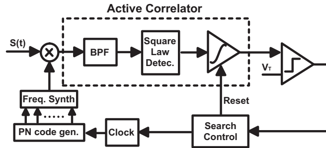
Figure 3.1 Stepped serial search scheme adapted from [34]
