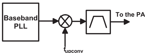
Figure 3.14 Modified transmitter architecture using a baseband PLL followed by an up-conversion mixer
