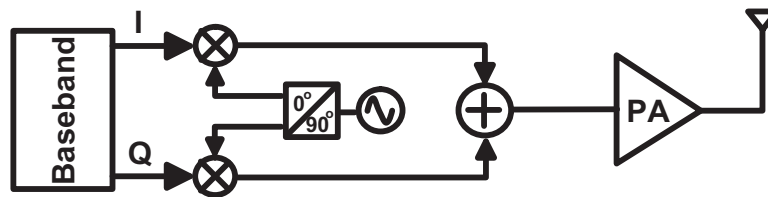
Figure 2.10 Direct conversion transmitter
