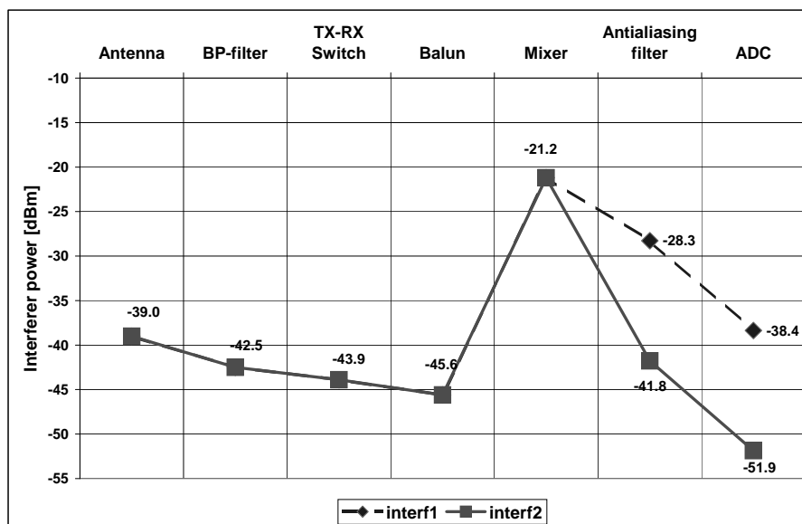
Figure 5.23 Adjacent and alternate channel interferer levels through the receiver chain
