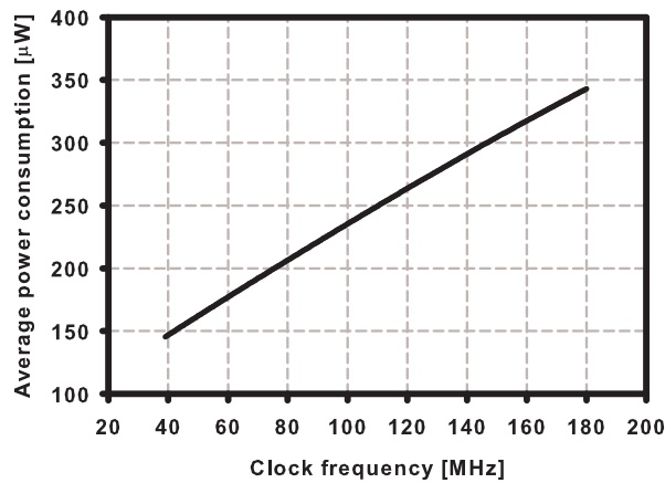
Figure 3.19 Digital back-end power consumption versus reference clock frequency
