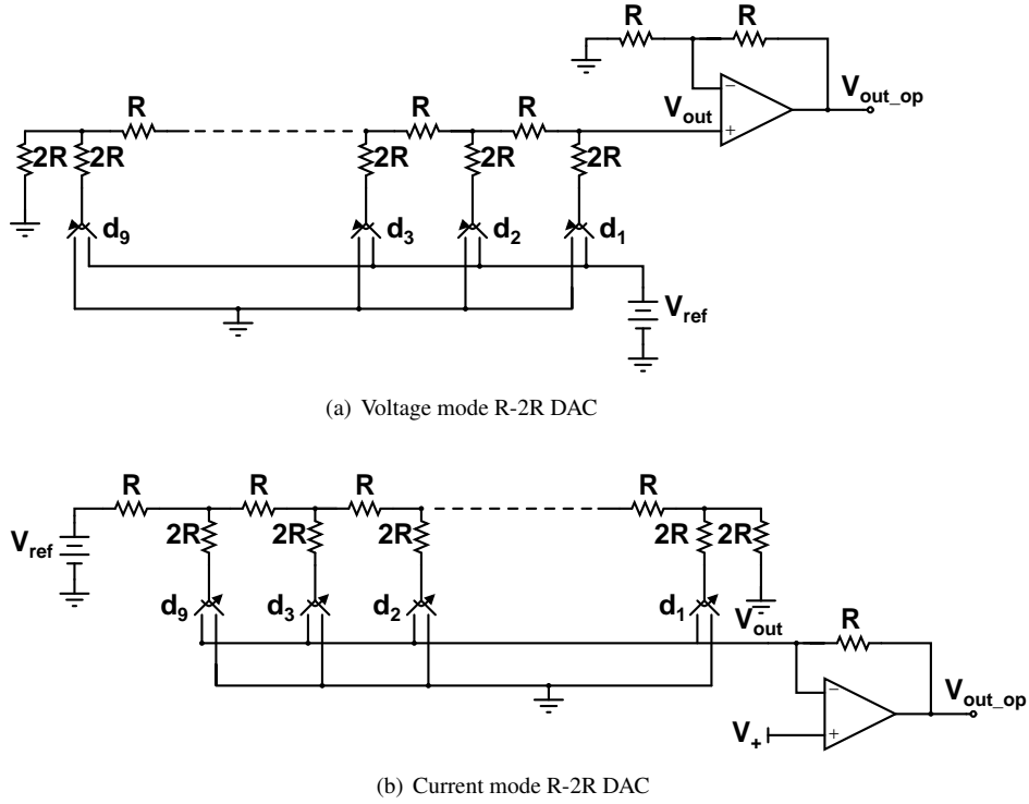
Figure 3.17 R-2R DAC topologies
