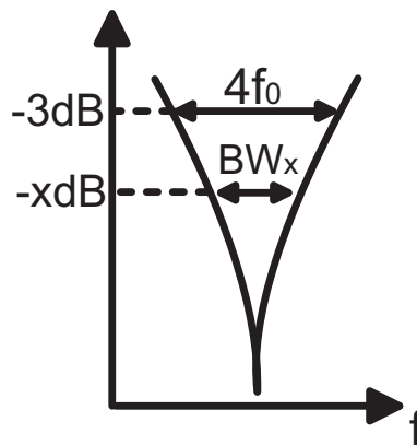
Figure 5.15 Bode plot of the twin-T notch filter
