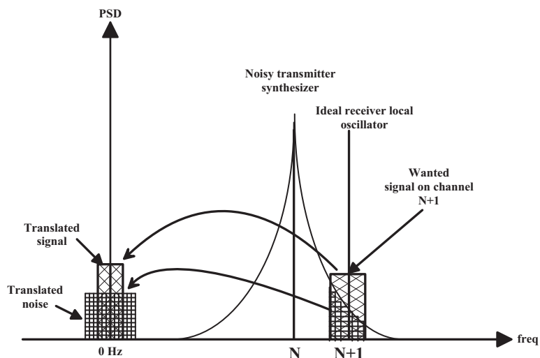
Figure 4.13 Effect of phase noise produced by an unwanted communication on the reception of the wanted signal
