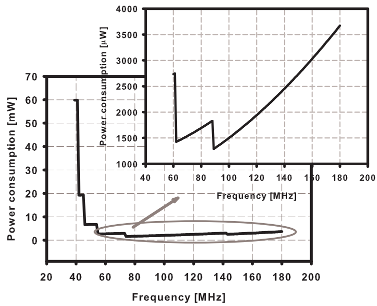
Figure 3.22 DDFS power consumption
