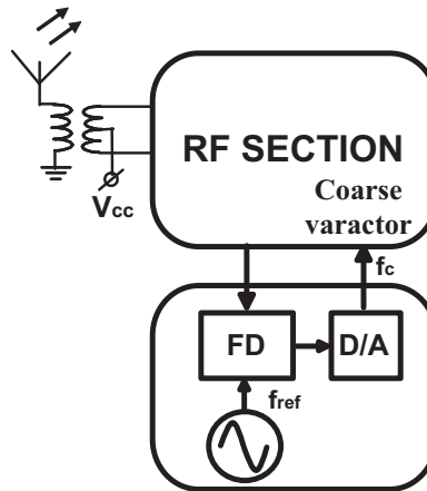
Figure 4.2 Initial calibration loop (FLL)
