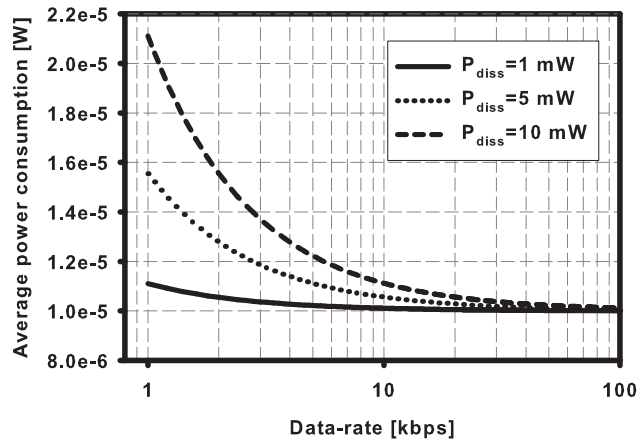
(b) P_{idle} = 10 \mu\text{W}
