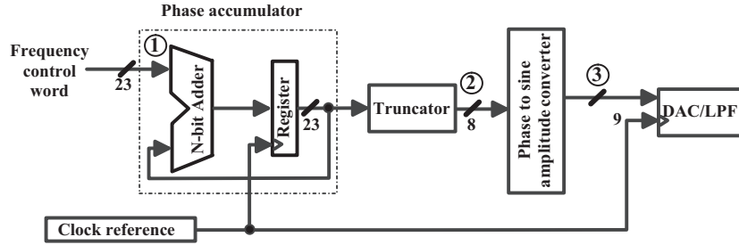
Figure 3.7 Basic direct digital frequency synthesizer, with bits required in the various stages
