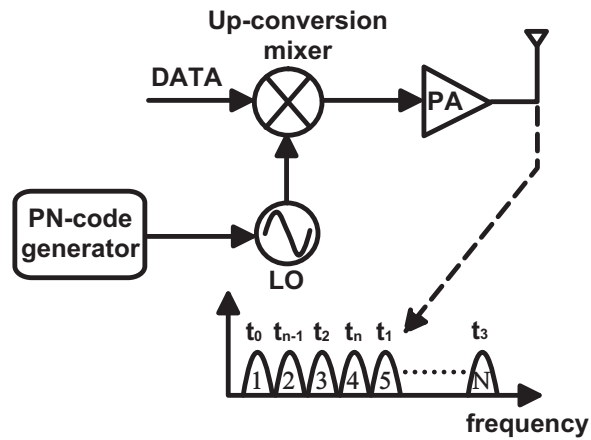
Figure 2.3 Schematic block diagram of an FHSS transmitter
