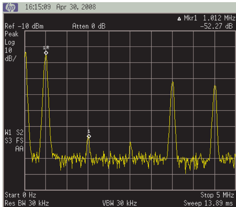
Figure 5.30 Spectrum of the 0.5 MHz synthesized waveform
