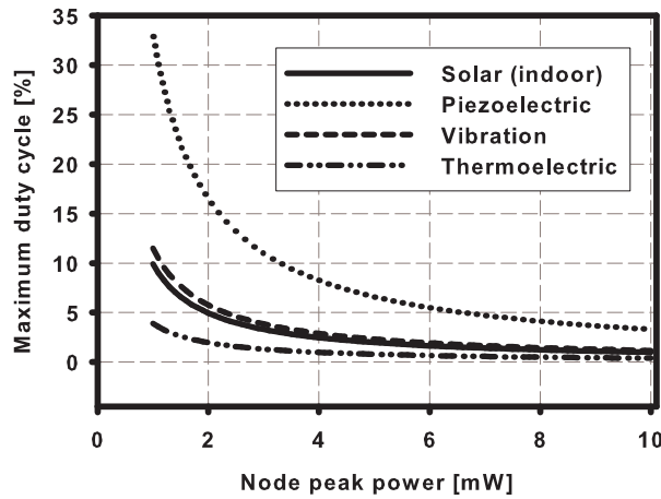
Figure 1.7 Maximum duty-cycle versus node peak power consumption for different harvesting technologies
