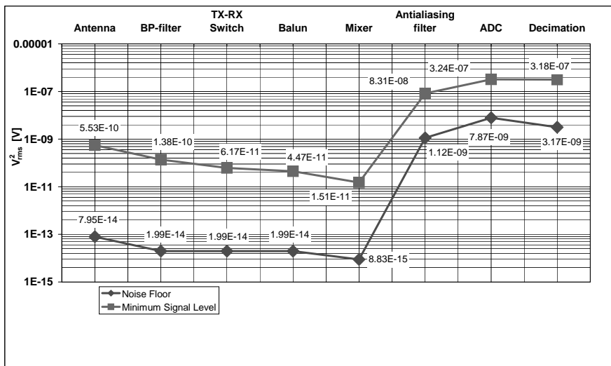
Figure 5.18 Signal and noise levels along the receiver chain referred to the input of each block
