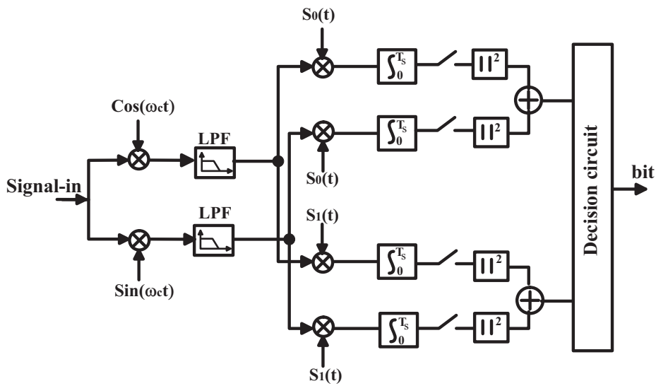
Figure 4.44 Non-coherent correlator receiver
