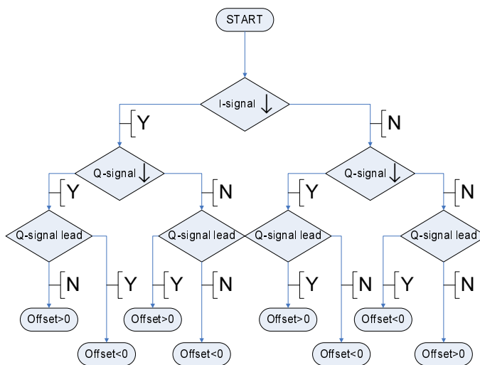
Figure 4.41 Frequency offset sign recovery method flowchart
