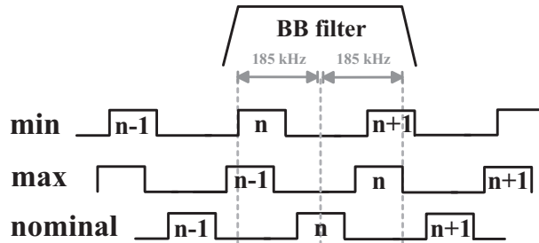
Figure 4.11 Effect of residual frequency errors on the choice of the RG base-band filter bandwidth
