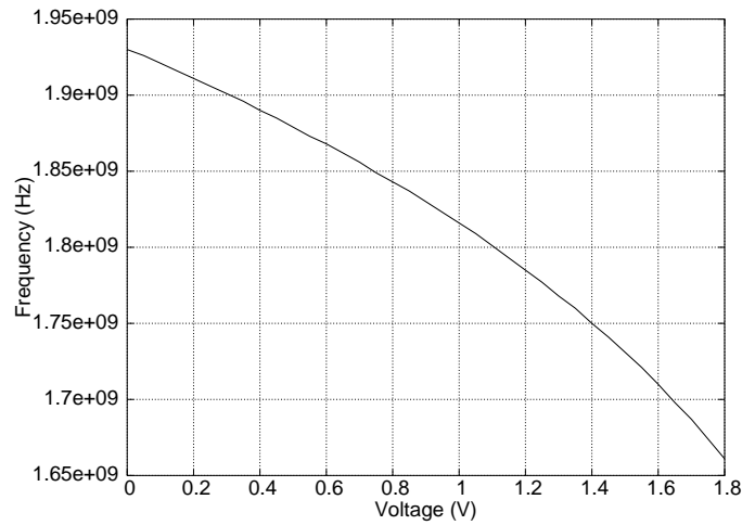
Figure 4.22 Varactor coarse tuning curve
