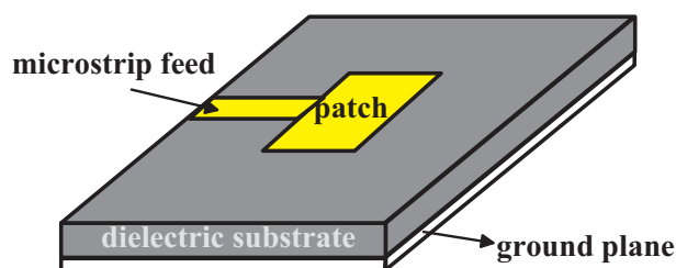
Figure 4.57 Microstrip line feed
