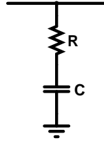
Figure 3.10 Simple first-order PLL loop filter
