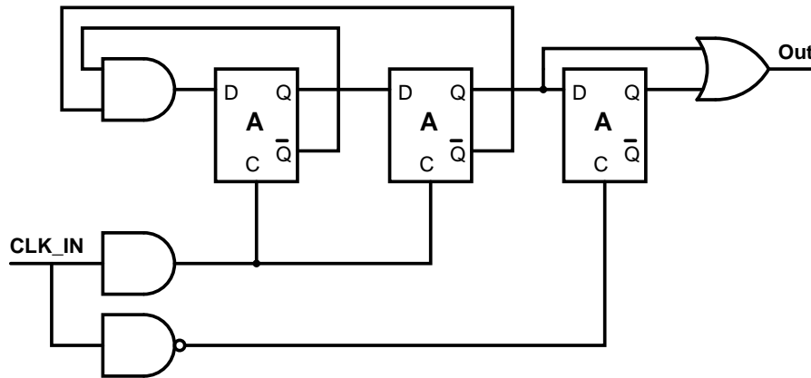
Figure 5.10 Divide-by-three frequency divider
