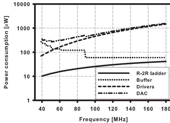
Figure 3.20 DAC power consumption
