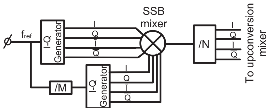
Figure 5.3 Simplified block diagram of the proposed baseband frequency hopping synthesizer
