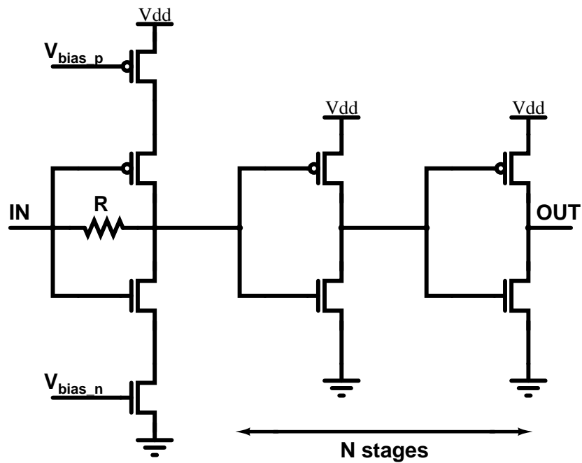
Figure 5.8 Schematic of the hard limiters in Fig. 5.6: N is equal to 3 for the path A and to 4 for the path B
