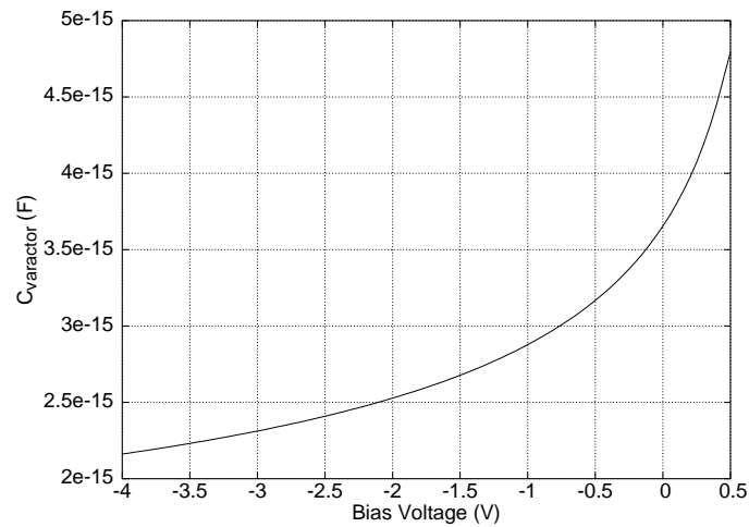
Figure 4.19 Simulated varactor capacitance curve
