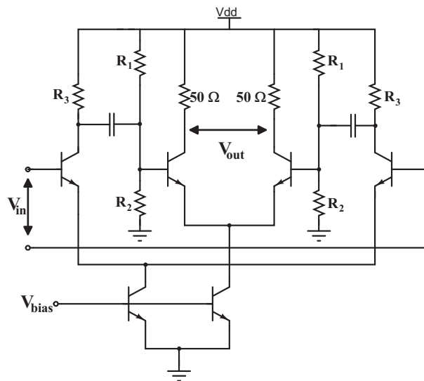
Figure 4.30 Output buffer
