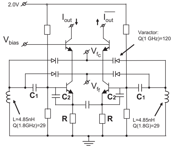
Figure 4.32 Circuit schematic of the differential cascoded Colpitts power-VCO
