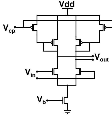
Figure 3.9 Schematic of a differential cell used in differential ring oscillators
