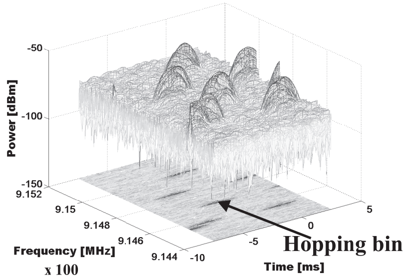
Figure 4.64 Received power spectrum (8 meters distance, NLOS condition, and -25 dBm transmitted power)
