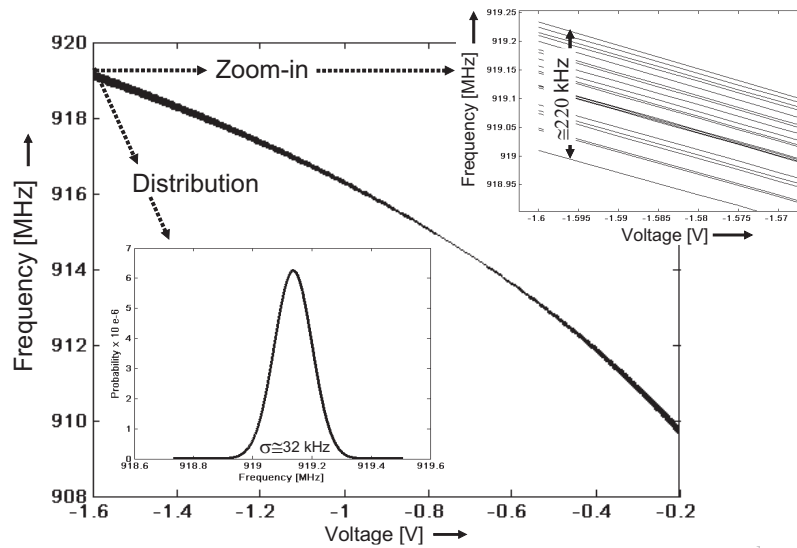
Figure 4.8 Measured fine tuning characteristic for 20 IC samples (same DAC)
