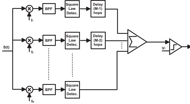
Figure 3.2 Passive correlator adapted from [34]
