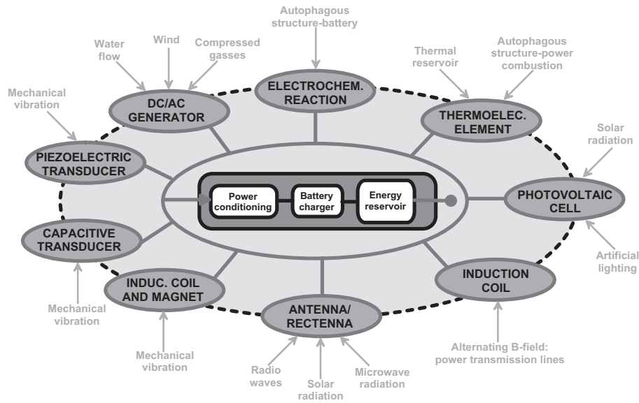
Figure 1.6 Various scavengable energies that can be used for portable systems (from [7]).
