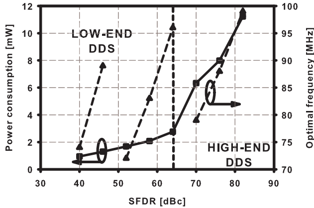
Figure 3.24 Minimum power consumption and optimal reference clock versus SFDR
