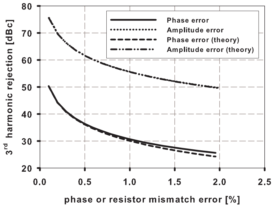
Figure 5.13 Effect of the resistor mismatch or phase mismatch on the 3 rd harmonic rejection
