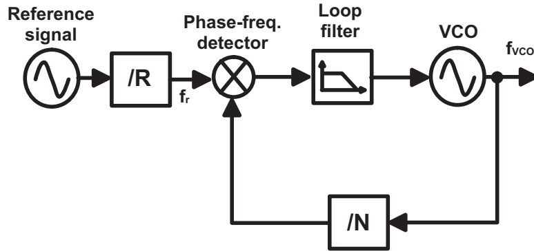
Figure 3.5 Integer-N PLL block diagram
