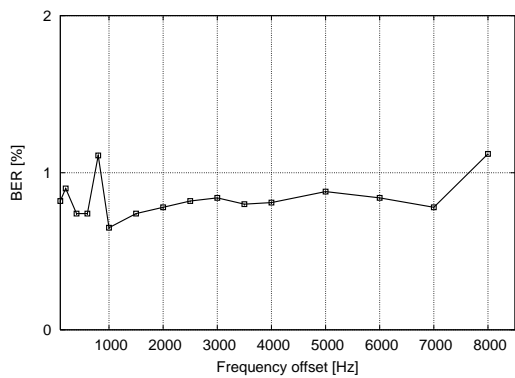
(c) ST-DFT
