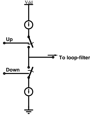
Figure 3.11 Simplified block diagram of a charge pump
