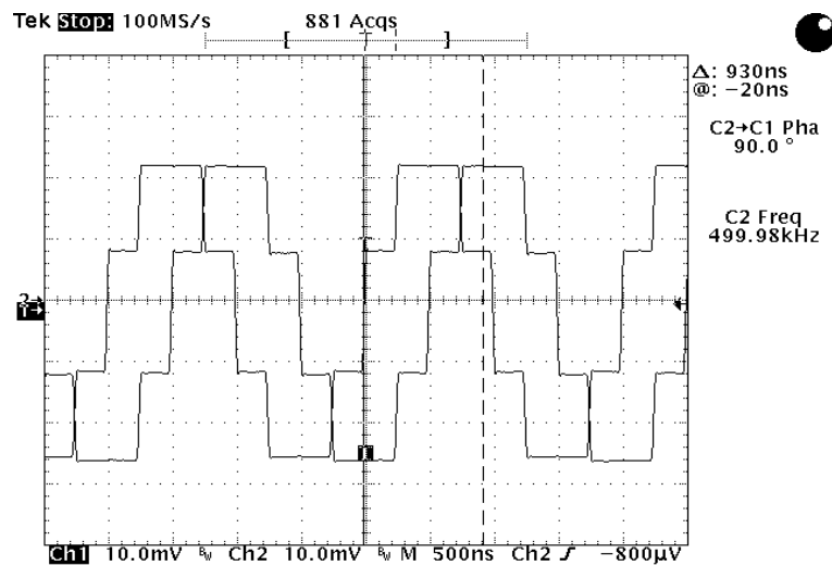
Figure 5.29 Time waveform of the 0.5 MHz synthesized frequency
