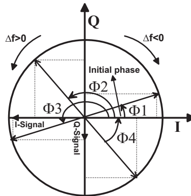
Figure 4.37 I-Q plane representation of the frequency offset component with different initial phases
