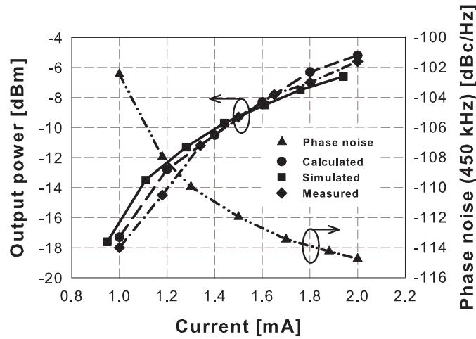
Figure 4.61 Output power and phase noise at 450 kHz offset versus bias current for the power-VCO based RF front-end
