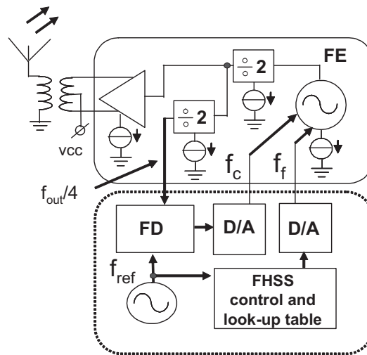
Figure 4.14 Proposed VCO-divider based frequency hopping transmitter architecture
