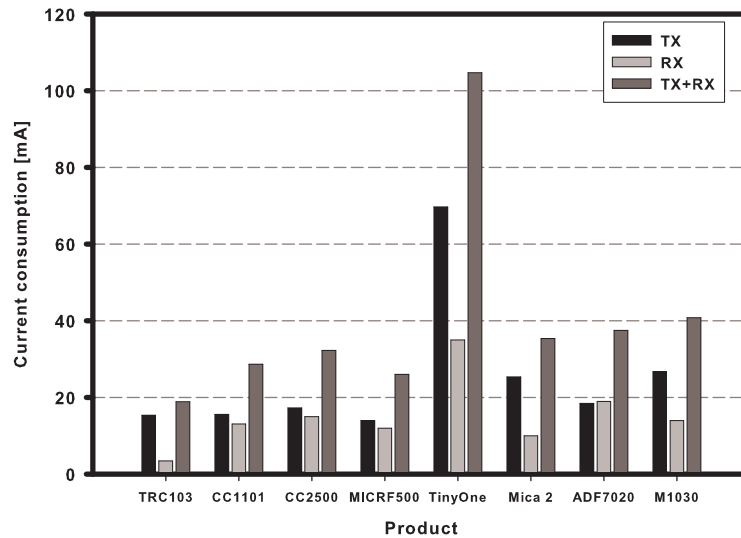
Figure 3.4 Power consumption of some commercial FHSS products normalized to -6 dBm output power
