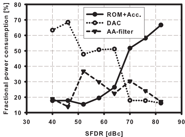
Figure 3.25 Power consumption break-down versus SFDR
