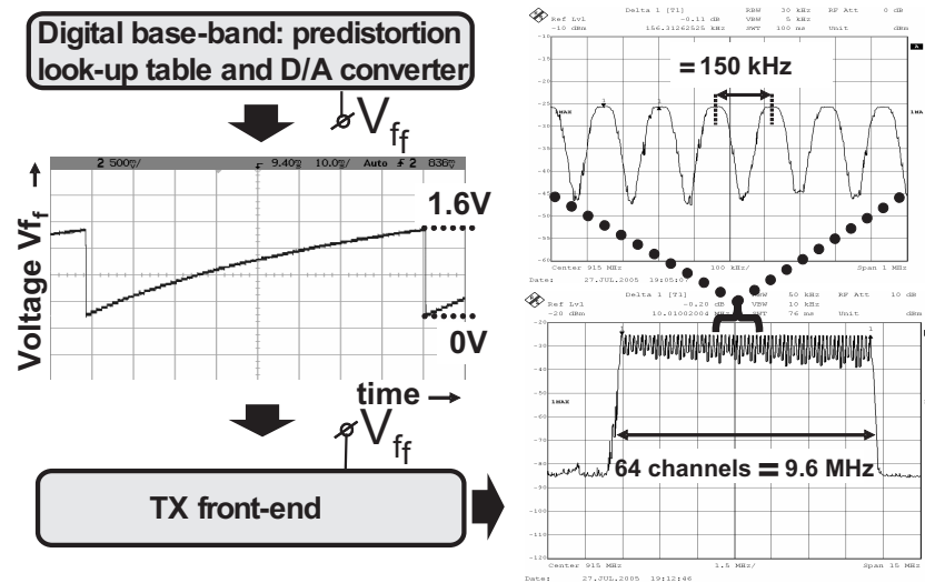
Figure 4.63 Pre-distortion chain with measured DAC pre-distorted output voltage and output spectrum of TX front-end
