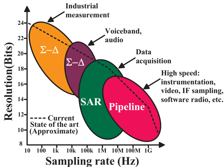
Figure 5.26 ADC architectures, application, resolution and sampling rates(from [128])
