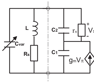
Figure 4.33 Common collector Colpitts small signal AC equivalent
