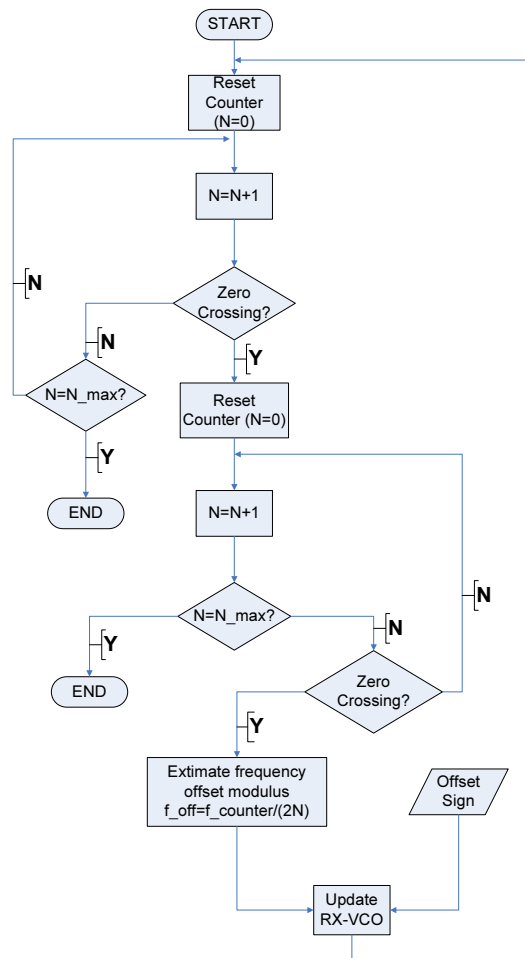
Figure 4.38 Frequency offset recovery algorithm flowchart
