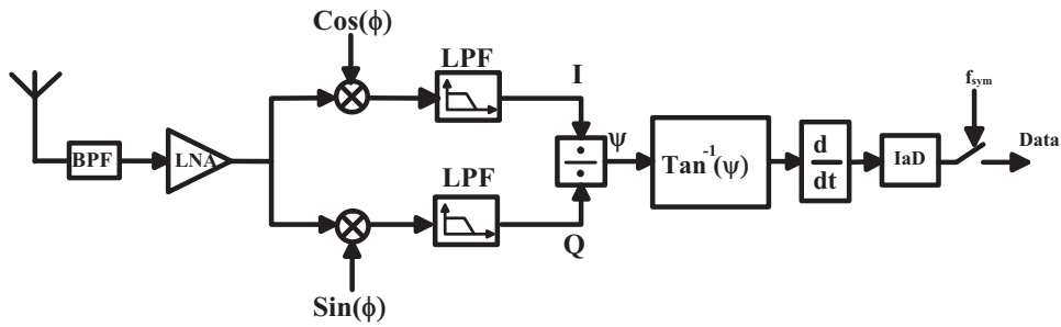
Figure 4.43 Conventional Arctangent receiver
