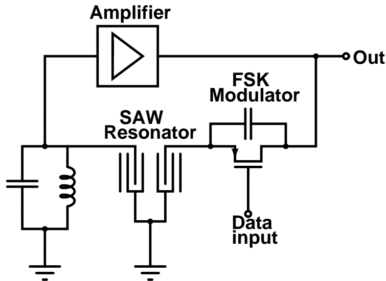
Figure 5.2 Block diagram of the Surface Acoustic Wave (SAW) stabilized LO with embedded FSK modulation functionality
