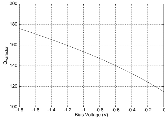
Figure 4.17 Varactor Q factor versus forward bias voltage
