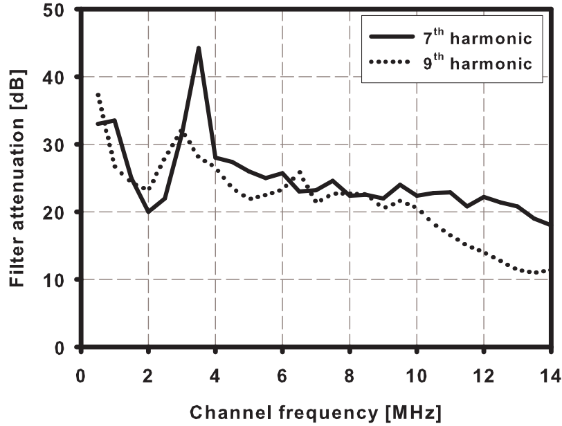
Figure 5.34 Measurement results of the stand alone LP-notch filter
