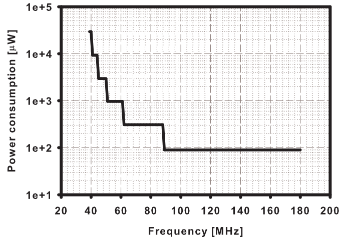
Figure 3.21 AA-filter power consumption
