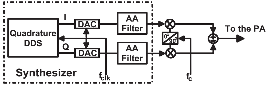
Figure 3.8 Complete DDFS based hopping synthesizer including the up-conversion stage
