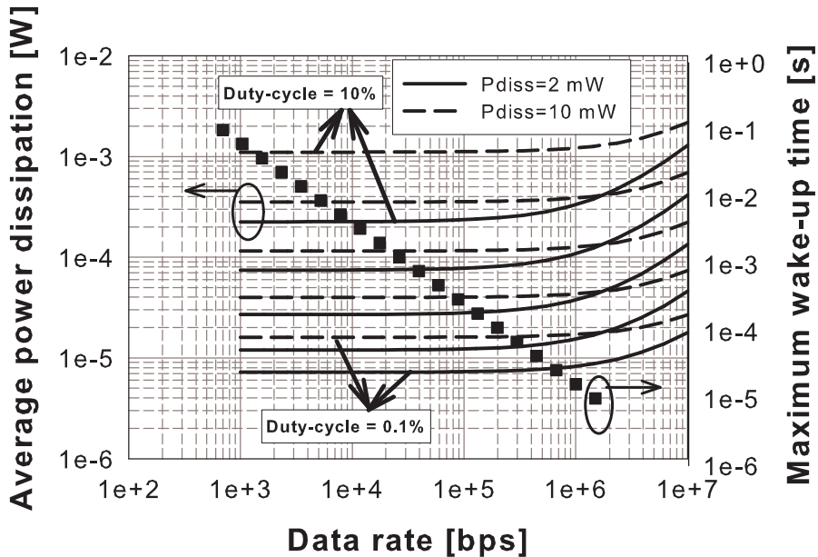
Figure 2.8 Average transmitter power consumption and maximum wake up time for different value of duty cycle, as a function of the data rate ( L_{pack}=1000 bits, NF=10 dB, \frac{E_b}{N_0}=20 dB, carrier frequency=915 MHz, P_{idle}=10 \mu W ) [30]
