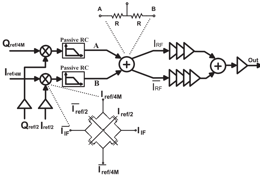
Figure 5.6 SSB mixer block diagram and partial circuit level implementation
