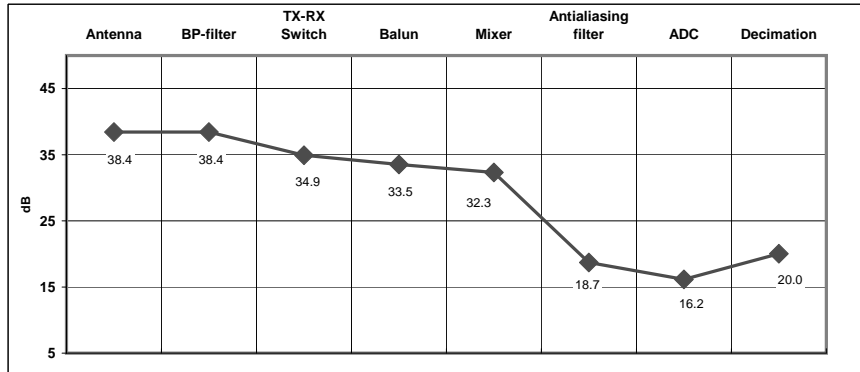
Figure 5.19 SNR along the receiver chain referred to the input of each block
