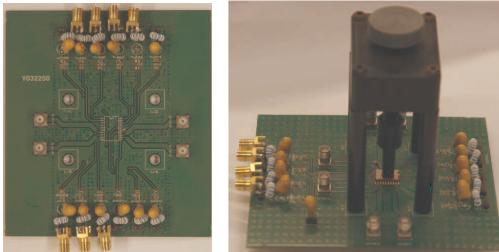
(a) PCB layout for the power-VCO based IC prototype
