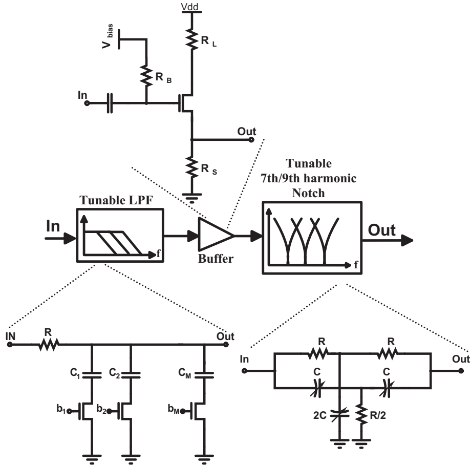
Figure 5.14 Schematic block diagram of the LP-Notch filter and its circuit level implementation
