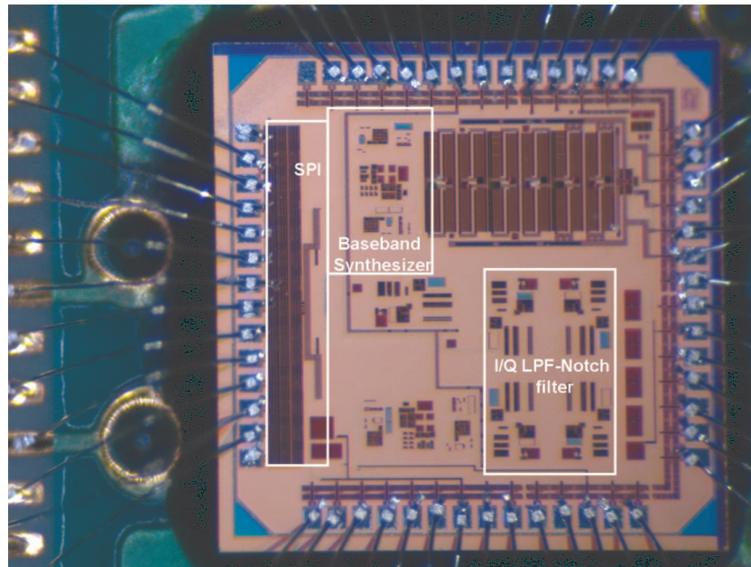
Figure 5.28 Microphotograph of the FHSS synthesizer in 90nm CMOS. The not highlighted parts contain a test structure for the baseband synthesizer without the LPF-notch, a single LPF-notch test structure and test-structures of a different system.
