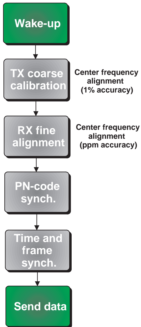
Figure 4.1 TX operation flowchart
