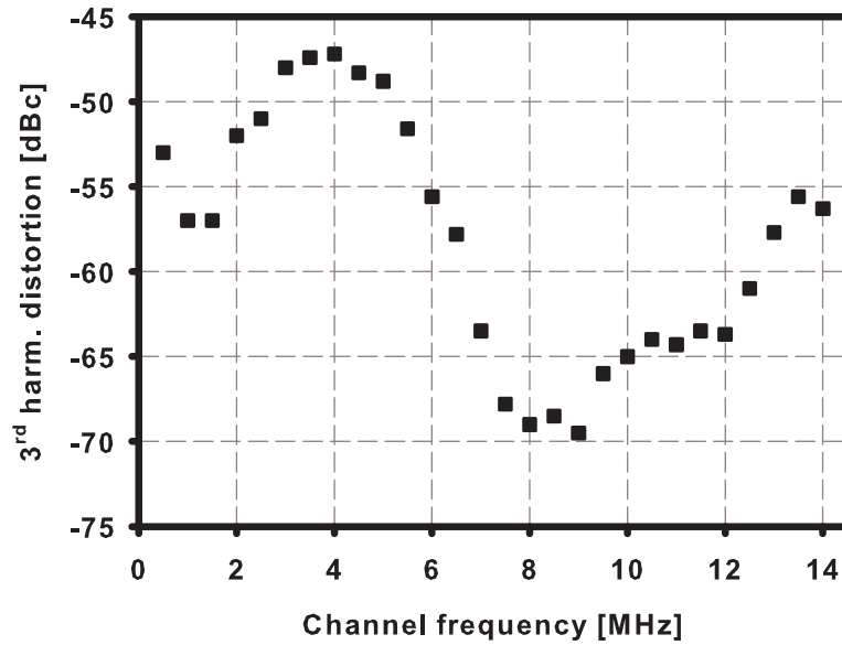
Figure 5.35 3 rd order LP-notch filter harmonic distortion
