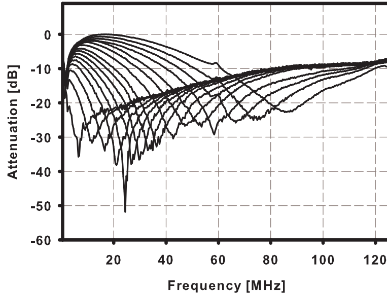
Figure 5.33 LP-notch filter transfer characteristics
