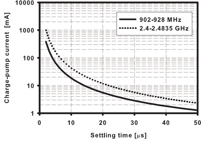
Figure 3.12 Charge pump current consumption versus the required settling time
