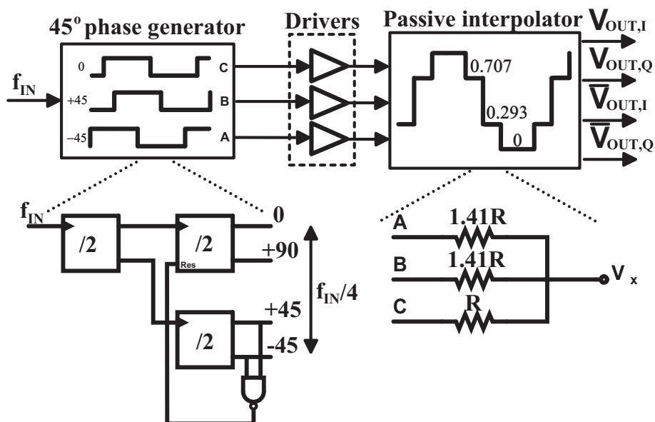
Figure 5.12 Walsh function harmonic rejection block
