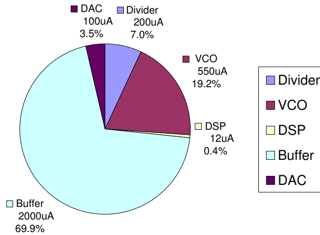
Figure 4.65 Power consumption breakdown by block for the LC-VCO-divider front-end (buffer not optimized for low-power)
