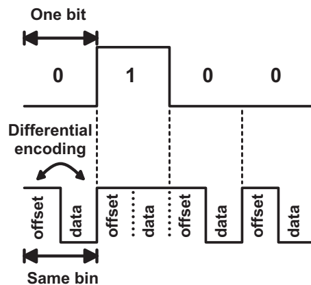
Figure 4.48 Residual offset cancellation technique
