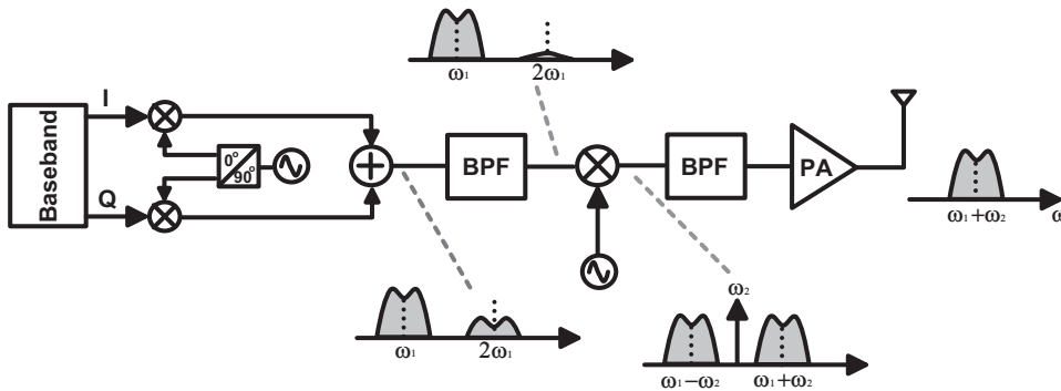
Figure 2.11 Two-step conversion transmitter (adapted from [32])
