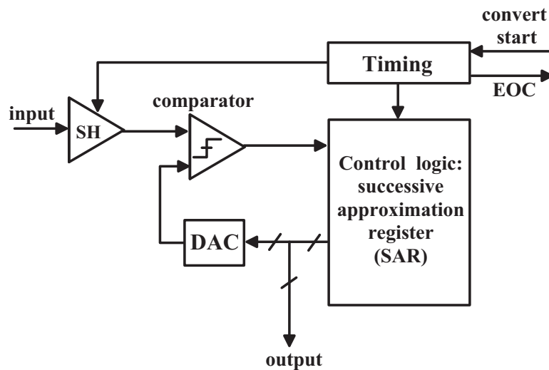
Figure 5.27 SAR ADC architecture(from [128])
