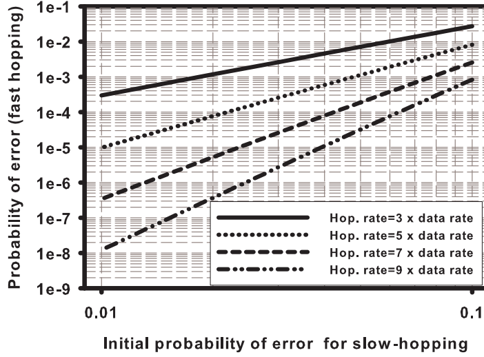
Figure 2.5 Probability of error at variable hopping rate using a majority decision criteria.
