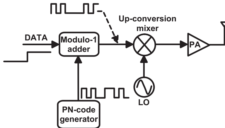
Figure 2.2 Schematic block diagram of a DSSS transmitter
