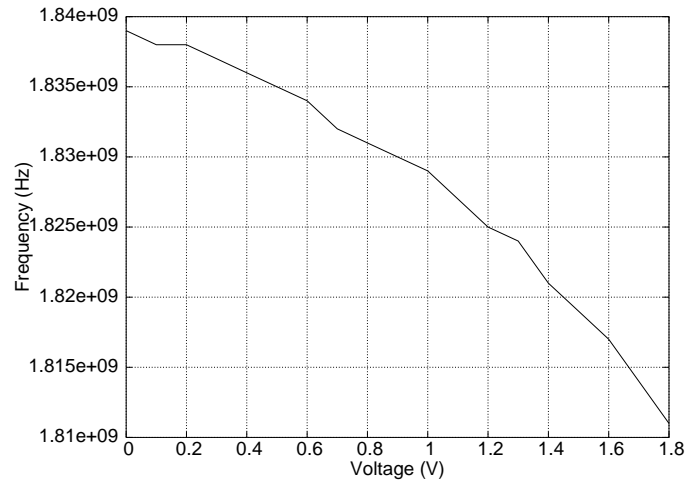
Figure 4.20 Fine tuning curve of a single varactor cell in the SOA technology
