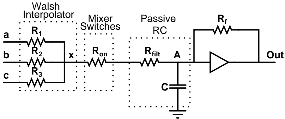
Figure 5.7 Mixer working principle, single ended signals, no SSB operation and single pole RC LPF
