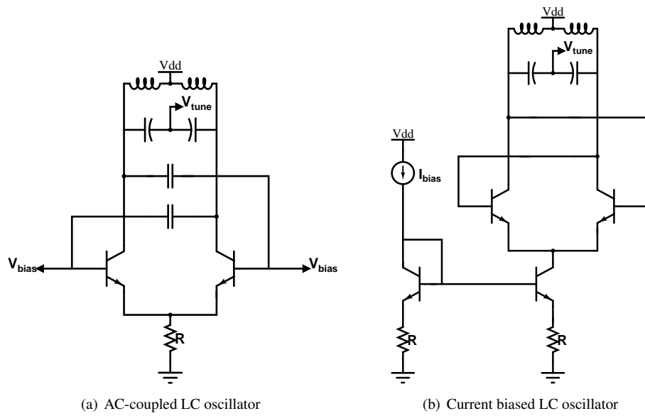
Figure 4.18 Two possible biasing techniques for an LC cross-coupled oscillator
