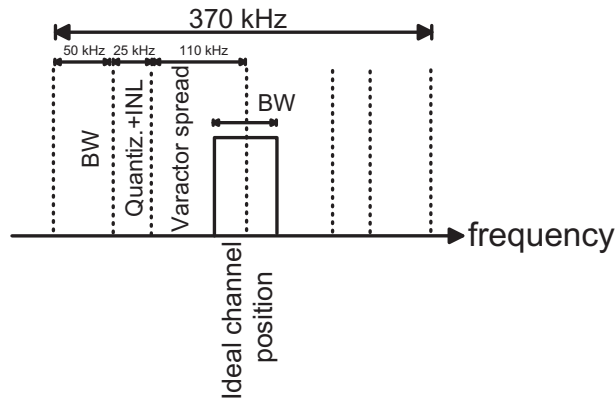
Figure 4.10 Minimum inter-channel spacing when varactor spread is considered
