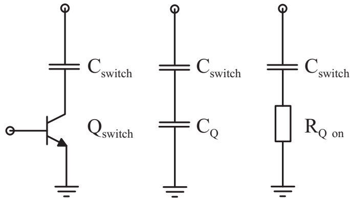
Figure 4.21 Typical switched capacitor circuit implementation and a simplified model for off-state and on-state respectively.
