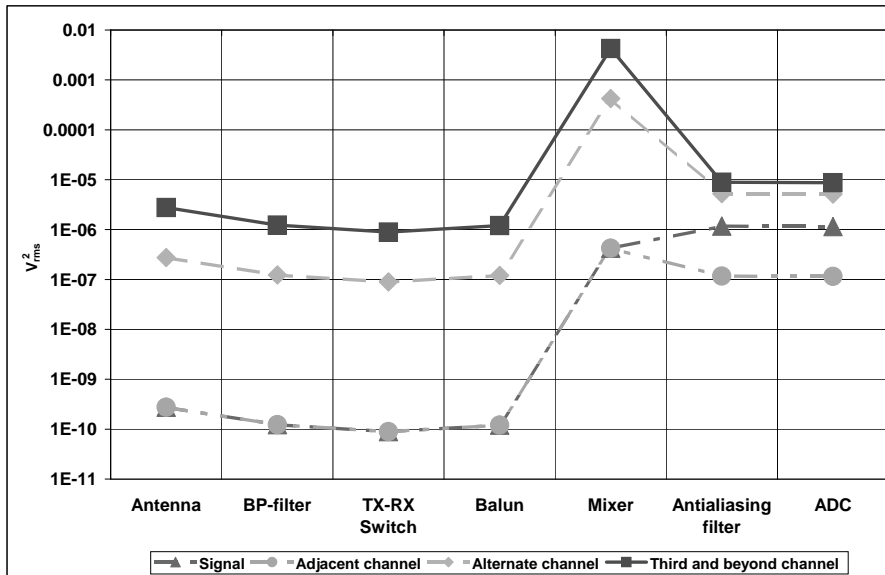
Figure 5.20 Signal and blockers levels along the receiver chain
