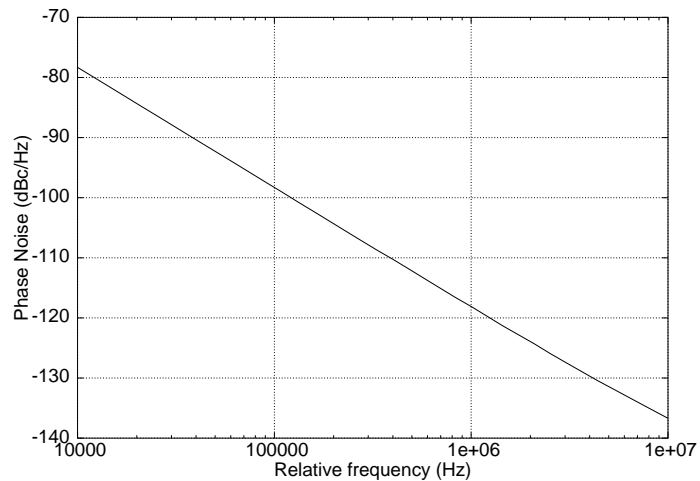
Figure 4.24 Phase noise plot for the topology with AC coupled cross-coupled pair and 20 feedback transistors in parallel
