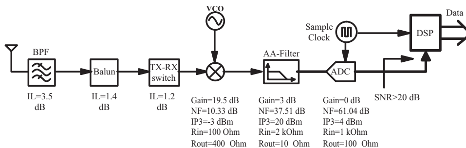
Figure 5.17 Receiver front-end blocks specifications
