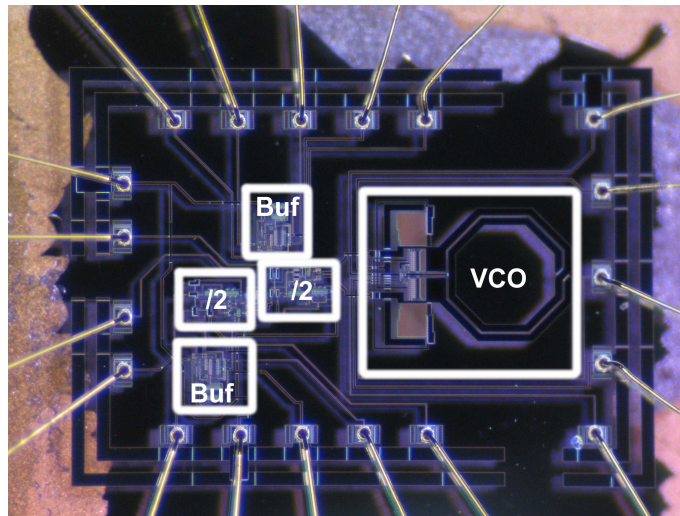
Figure 4.51 1 st IC prototype silicon implementation
