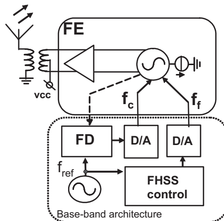
Figure 4.31 Power-VCO based frequency hopping transmitter architecture
