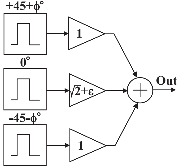
Figure A.1 Simplified model to evaluate the harmonic rejection sensitivity to resistor mismatches and signal phase unbalances
