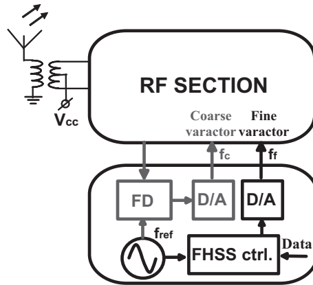
Figure 4.5 FHSS synthesizer block diagram: the frequency pre-distortion path is included
