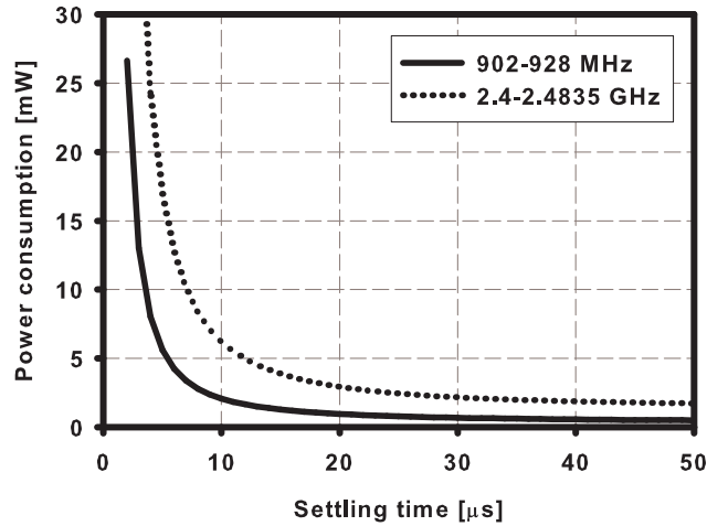
Figure 3.13 PLL power consumption estimation versus the required settling time
