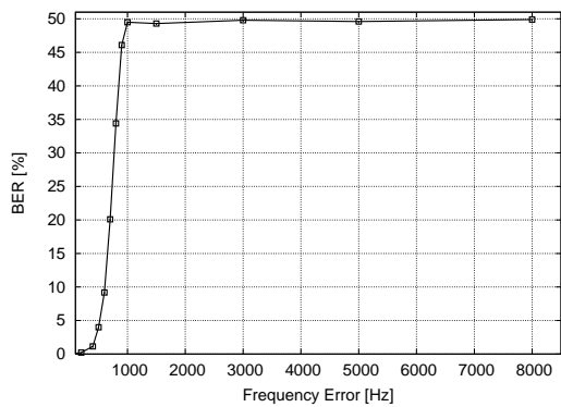
(b) Correlation
