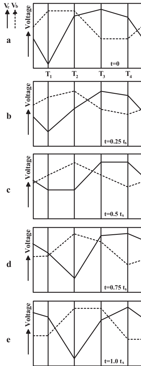
Figure 4.28 The collector voltage V_c and the base voltage V_b of the transistors T_1 to T_4 during one step of the switching process. After four steps the starting position is reached again.
