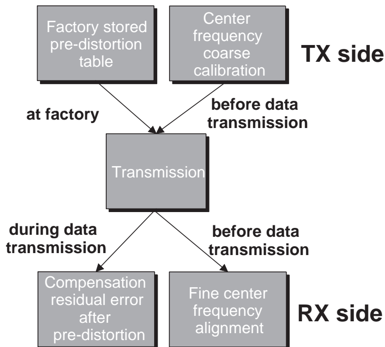
Figure 4.4 Center frequency alignment and frequency bin synthesis flowchart
