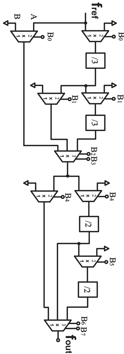
Figure 5.9 Schematic block diagram of the programmable divide-by-M frequency divider; the divide-by-N frequency divider is designed using the same architecture
