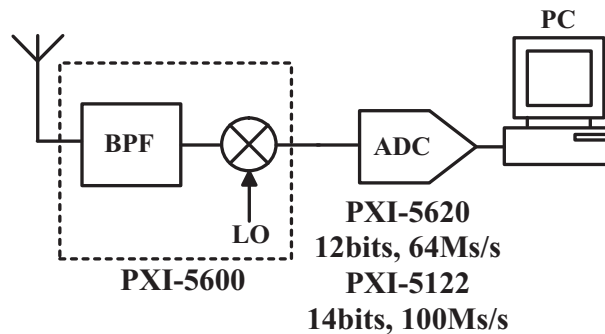
Figure 4.60 RG receiver implemented using a PC and measurement instruments
