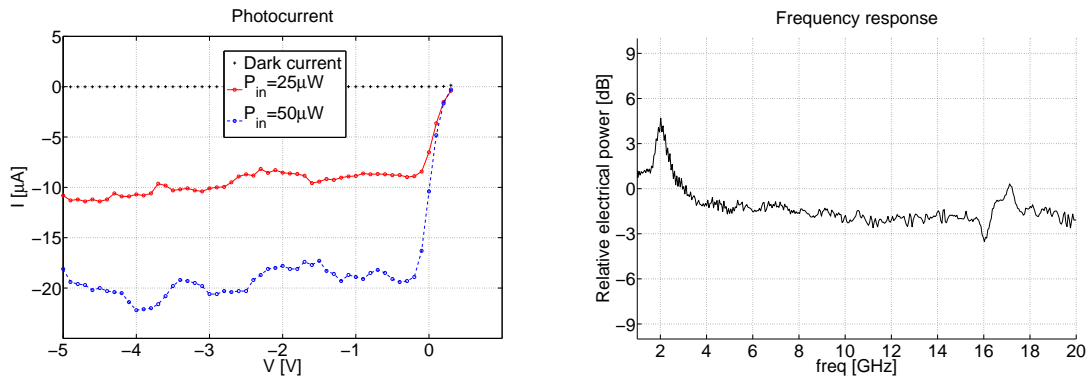
Figure 4: Left: Measured photocurrent for 0, 25 and 50 \mu\text{W} optical input power as a function of the detector applied bias voltage. Right: Detector frequency response.
