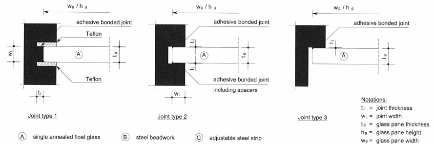
Figure 1 Joint type 1 to 3
