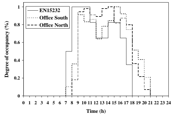
Figure 4 Degree of occupancy for offices, Comparison of EN15232 and observations, Beta-Building, Floor 4, Wing A
