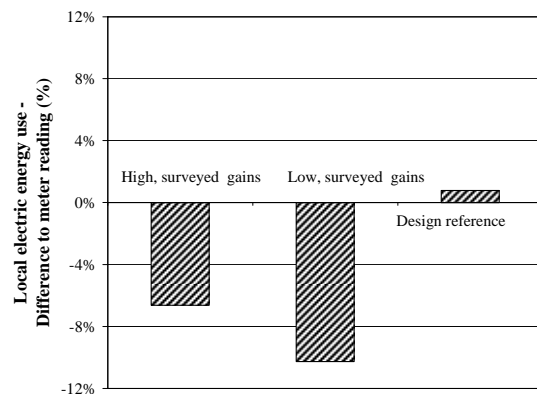
Figure 6 Comparison of local electric energy use from estimations and meter reading, Wing A, 4 th floor, Metered electricity use 7585kWh
