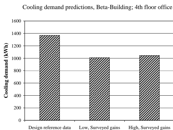
Figure 7 Cooling demand predictions for 4 th floor offices; Beta-Building
