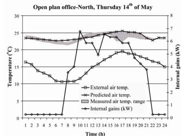
Figure 3 Measured and predicted air temperatures for north-facing open plan office on the 4 th floor. Grey area indicates air measurement range by sensor 1 &. The internal gains represent sensible gains from electrical equipment, lighting and people.
