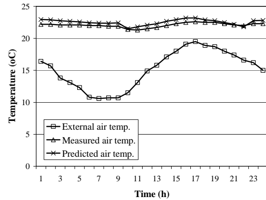
Figure 2 Predicted and measured air temperatures for an unoccupied office unit on the 3 rd Floor of Wing A on the 14 th of May.
