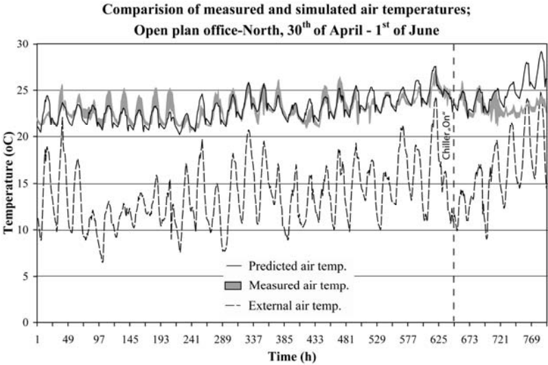
Figure A1 Comparison of measured and simulated air temperatures for the North-facing open plan office space on Floor 4 of Wing A.
