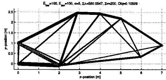
Figure 8: Optimal control/top/geo, displacement under load
