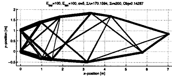
Figure 7: Optimal topology/geometry, displacement under load
