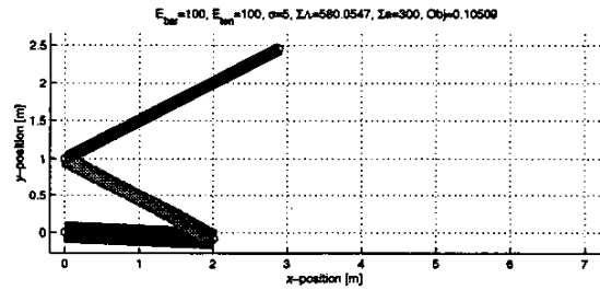
Figure 9: Optimal control/top/geo, controlled tendons
