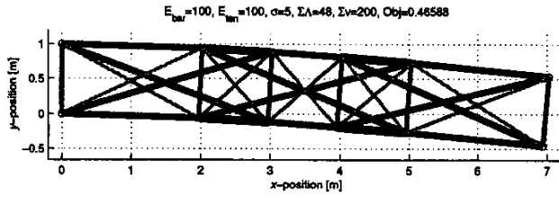
Figure 1: Basic tensegrity beam system (not optimized)
