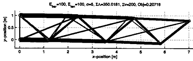
Figure 2: Optimal topology/geometry, displacement under load
