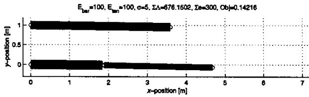
Figure 4: Optimal control/top/geo, controlled tendons
