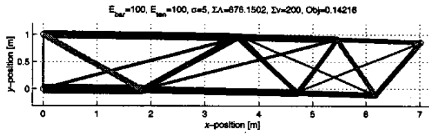
Figure 3: Optimal control/top/geo, displacement under load
