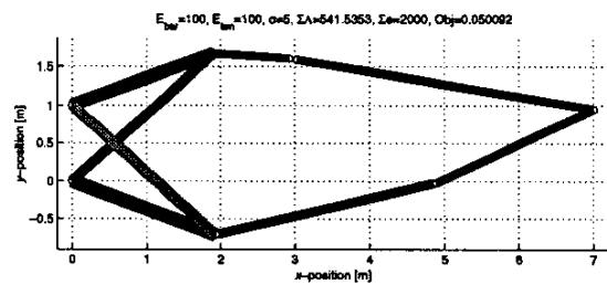
Figure 11: Optimal control/top/geo, controlled tendons
