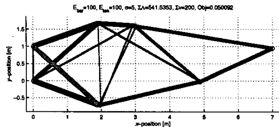
Figure 10: Optimal control/top/geo, displacement under load
