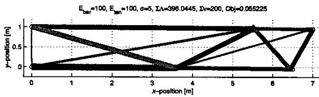
Figure 5: Optimal control/top/geo, displacement under load
