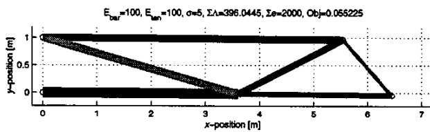
Figure 6: Optimal control/top/geo, controlled tendons
