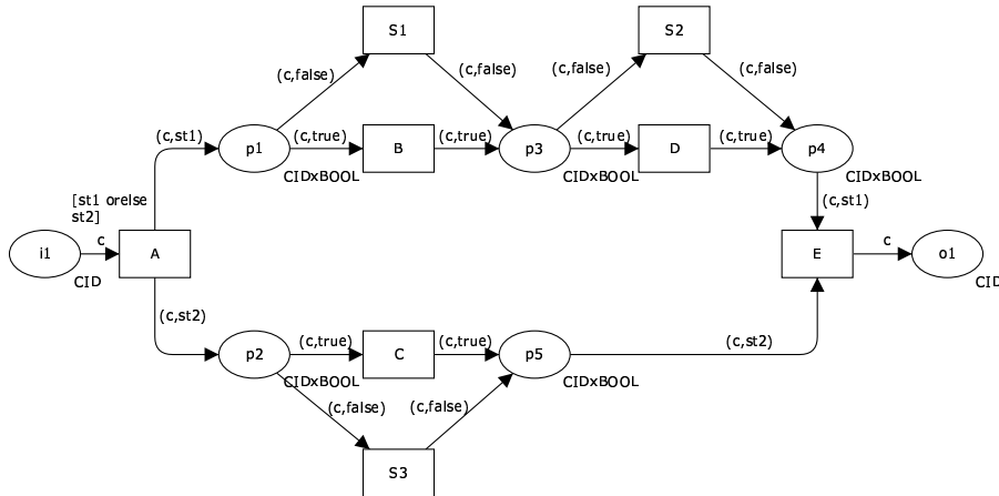
Figure 8: Acyclic synchronizing merge pattern
