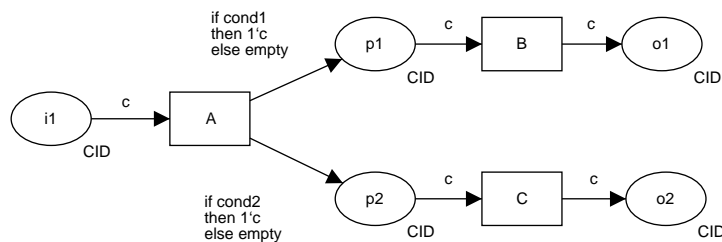
Figure 6: Multi-choice pattern
