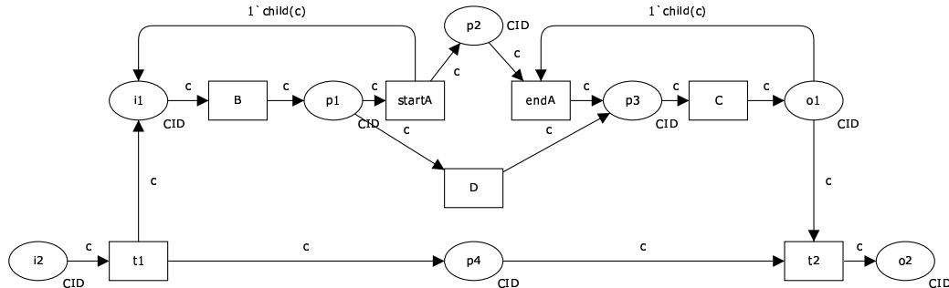
Figure 34: Recursion implementation
