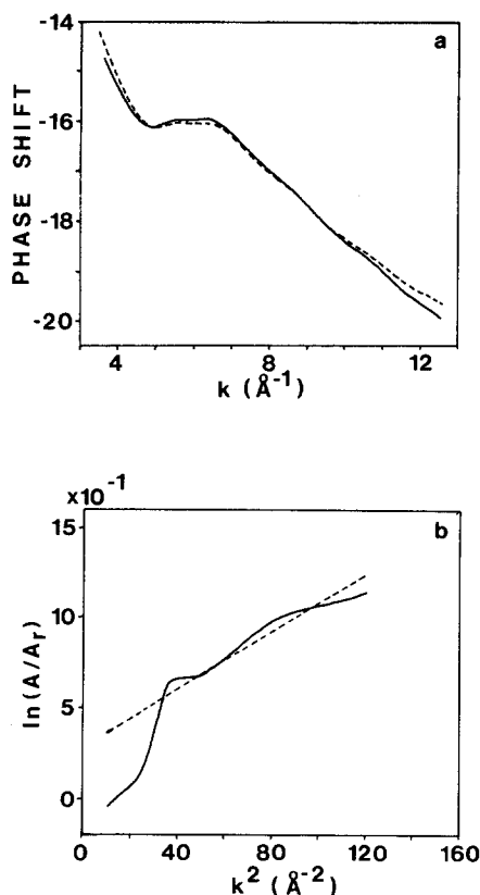
FIG. 6. (a) Phase shift function \varphi(k) of the reference compound (dotted line) and catalyst (B) (solid line), (b) log plot of A/A_r vs k^2 (solid line). The dotted line represents the best fit straight line.
