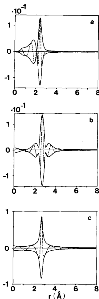
FIG. 1. Imaginary part (dotted line) and magnitude (solid line) of the Fourier transform ( k^{-1} -weighted, \Delta k = 2.68\text{--}24.4 \text{ \AA}^{-1} ) of a single shell Rh-Rh EXAFS ( N = 6 , R = 2.687 , \Delta\sigma^2 = 0.005 ): (a) normal, (b) Rh-Rh phase corr., (c) Rh-Rh phase and amplitude corr.
