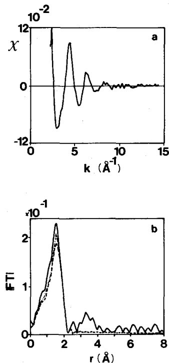
FIG. 3. Impregnated and dried 0.57 wt. % Rh/Al 2 O 3 catalyst: (a) EXAFS spectrum, (b) normal Fourier transform ( k^{-1} -weighted, \Delta k = 2.58\text{--}10 \text{ \AA}^{-1} ) of experimental data (solid line), of calculated EXAFS: (---) ( N_{\text{Rh-O}} = 3 , N_{\text{Rh-Cl}} = 3 ), (-----) ( N_{\text{Rh-O}} = 3.8 , N_{\text{Rh-Cl}} = 3 ).
