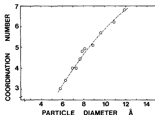
FIG. 11. First shell Rh–Rh coordination number as a function of the diameter of a half-spherical rhodium particle, having an fcc structure.
