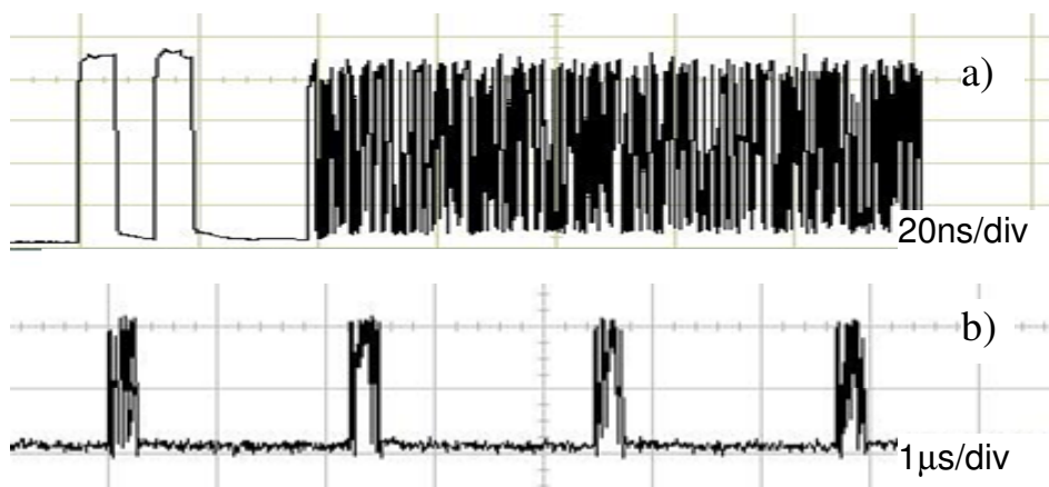
Figure 7.7 a) Fixed length packets with 155Mb/s 4-bit headers and 102.4ns 10Gb/s payloads are transmitted every second timeslot, b) which are 1.107μs long. Fixed length synchronous packets were used to demonstrate contention resolution.
