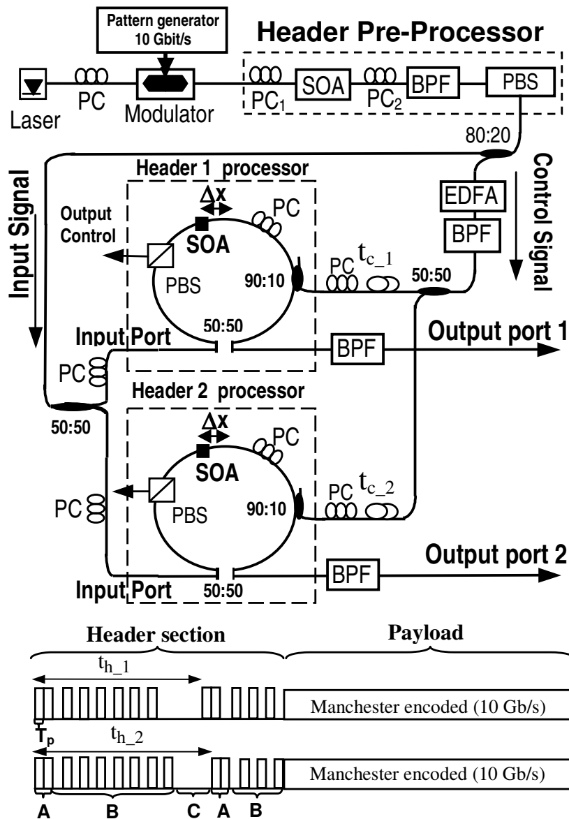
Figure 2.2 Experimental setup to demonstrate the header processing system and packet structure. PC : polarisation controller, EDFA : erbium doped fibre amplifier, BPF : band pass filter, PBS : polarisation beam splitter.
