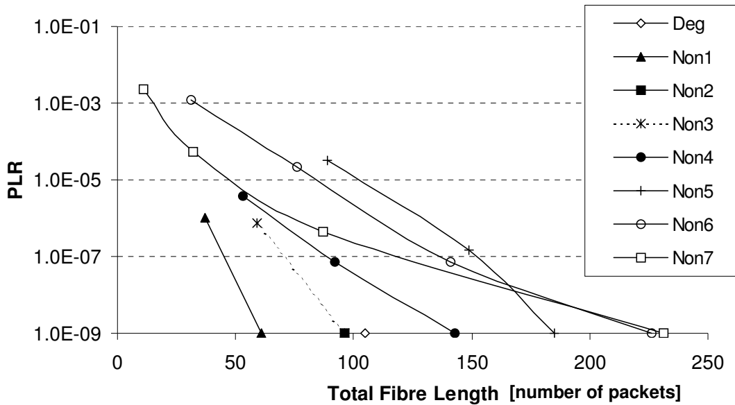
Figure 3.5 Figures a) and b) show the packet loss ratio for an output travelling buffer and a recirculating buffer, respectively. The performance is measured versus the total amount of fibre required for buffering, measured in the number of packets buffered in the fibre. It is clear that recirculating buffers outperform travelling buffers. For both, nondegenerate configurations outperform a degenerate buffer configuration.
