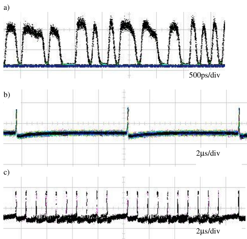
Figure 6.7 a) A close up of the 10Gbit/s 2^7-1 payload after 10 recirculations. The pattern is clear with little signal quality degradation. b) Packets are buffered 10 times, so there are 10 793ns time slots in between output packets from the CrossPoint switch, ( 8.7\mu\text{s} between payloads). c) 10 unbuffered packets are directly switched to an alternative output.
