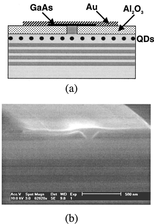
FIG. 1. (a) Schematics of the fabricated LED structure. (b) Cross-sectional SEM image of a 70 nm aperture obtained by lateral oxidation from a 1- \mu\text{m} -wide stripe.
