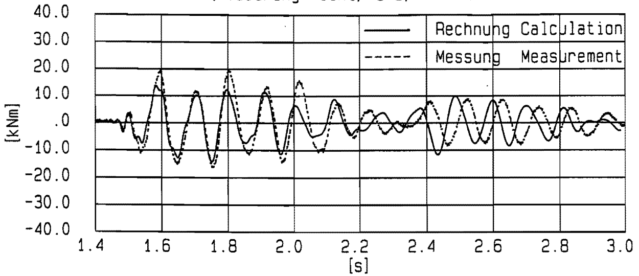
Mess-Stelle (Measuring Point) 34B; Mx: Torsionsmoment
