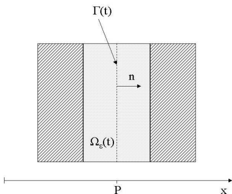
Figure 7: Geometry in model (P_\Gamma) and (P_{\Gamma\epsilon}) .
