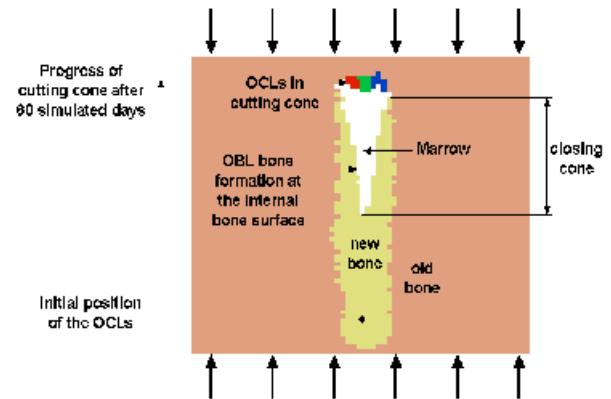
Figure 1: Depiction of the computed morphology after 60 simulated days. Mechanically induced osteocyte signals are capable of directing osteoclast resorption in the external loading direction. They also explain subsequent coupling of osteoblast bone formation to resorption.
