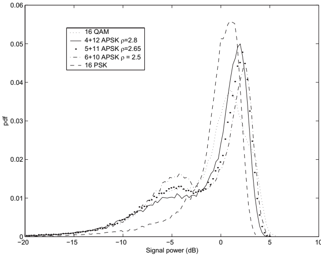
Fig. 4. Simulated histogram of the transmitted signal envelope power for 16-ary constellations.
