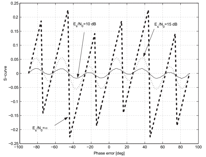
Fig. 8. Simulated APSK phase error detector S-curve for E_s/N_0 = \infty, 15, 10 dB; 4+12-APSK 4Q-DD scheme.
