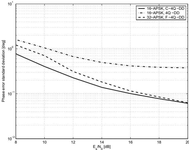
Fig. 11. APSK simulated phase jitter for: 16-APSK 4Q-DD, 16-APSK C-4Q-DD and 32-APSK F-4Q-DD estimators: [B_L \cdot T_s]_{\infty} = 10^{-4} .
