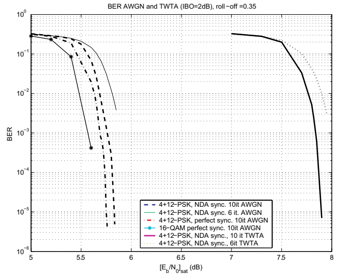
Fig. 14. Rate r=3/4 turbo coded simulated BER of 16-QAM and 16-APSK in the AWGN channel and the nonlinear channel with IBO= 2 dB, roll-off factor=0.35, clock timing and carrier phase recovery.
