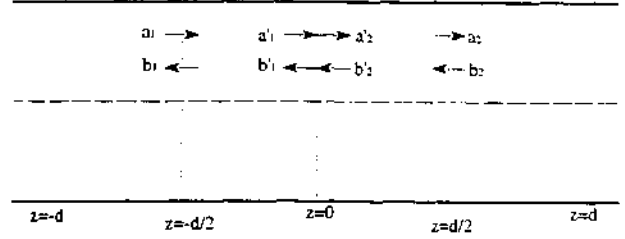
Figure 3: A section of the infinitely long periodic structure.
