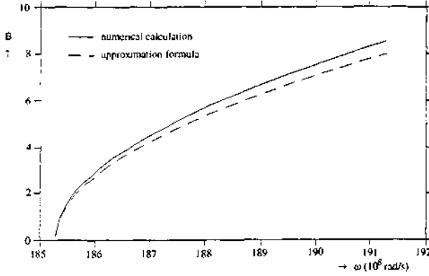
Figure 2: The susceptance as a function of the frequency, using b = 39 mm and a = 10 mm.
