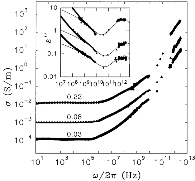
FIG. 2. \sigma'(\omega) between 5 Hz and 3 THz at 300 K for three doping levels 0.03 < c < 0.22 . In the inset the loss function \epsilon''(\omega) = \sigma'(\omega)/\epsilon_0 \omega is plotted for the same three samples. Drawn lines are fits to Eqs. (2) and (3). Data are corrected for the relatively small dipolar response of the alkoxy side chain (the maximal value of \epsilon'' = 0.1 is centered around 0.5 GHz), most clearly visible in the undoped polymer.
