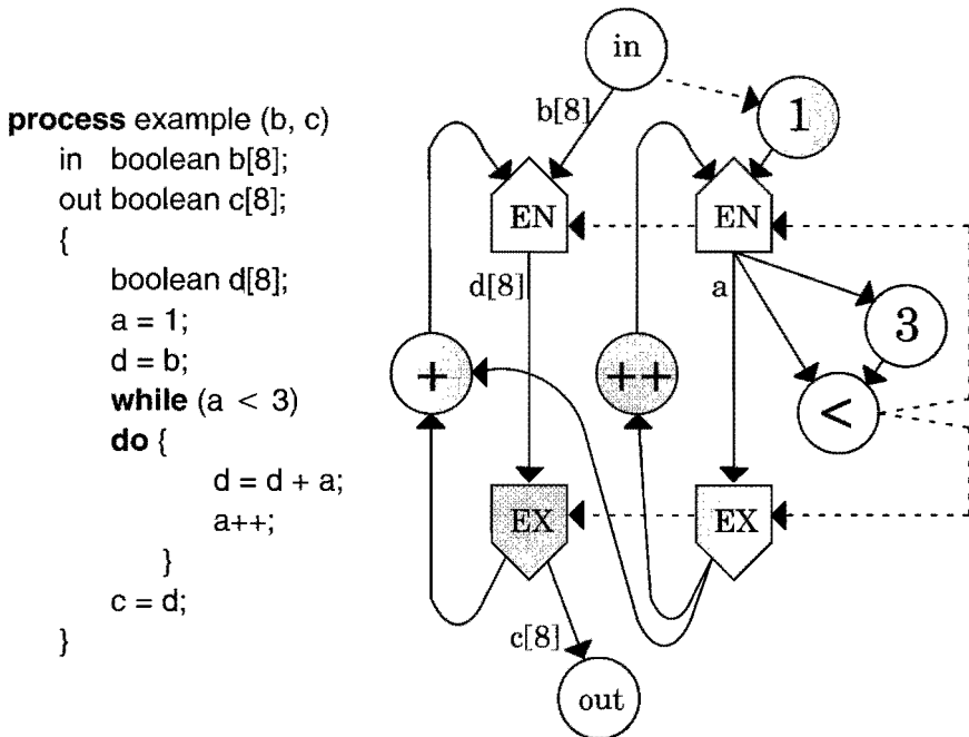
FIGURE 1.4. Example of a data flow graph.
