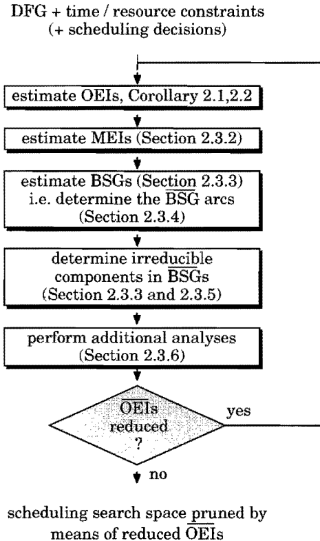
FIGURE 2.2. Flow of the execution interval analysis of Section 2.3.
