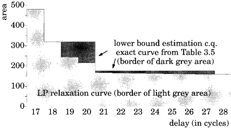
FIGURE 4.4. LP relaxation results for WDELF.
