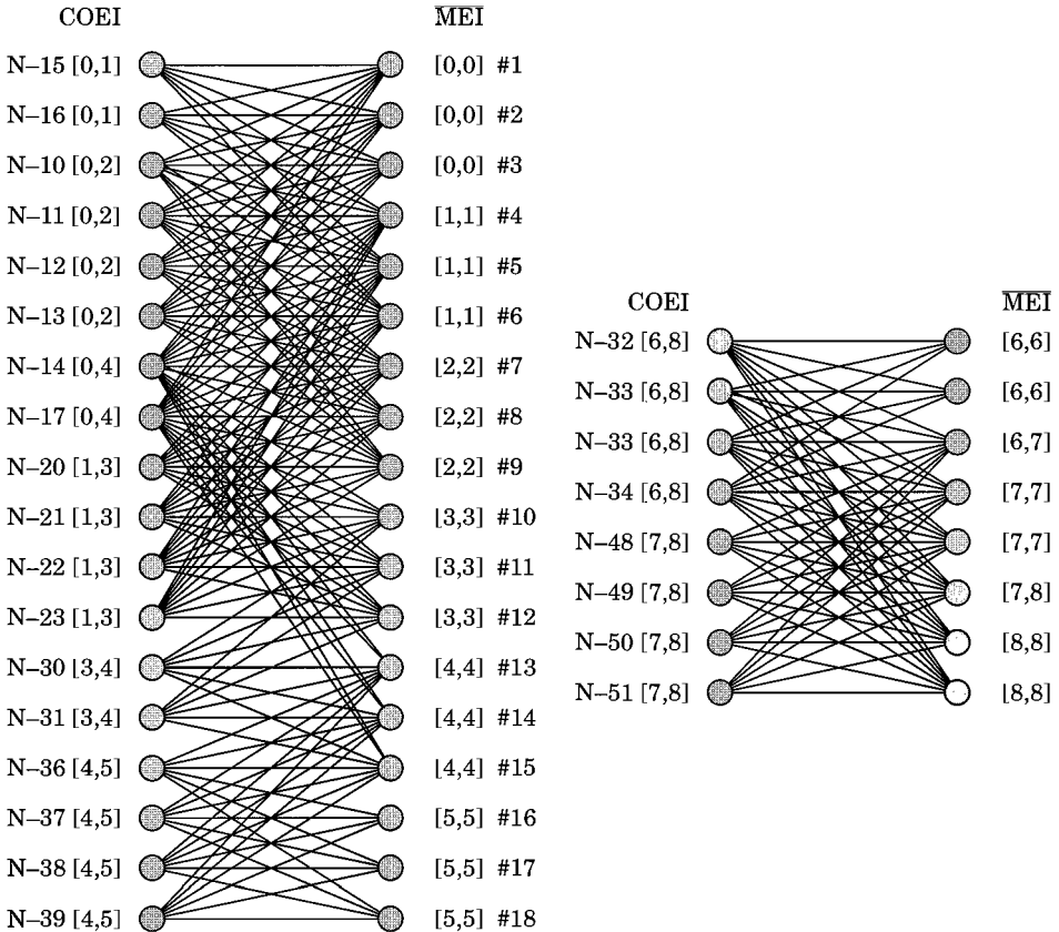
FIGURE 4.2. \overline{\text{BSG}} for additions/subtractions of FDCT in Figure 2.3.
