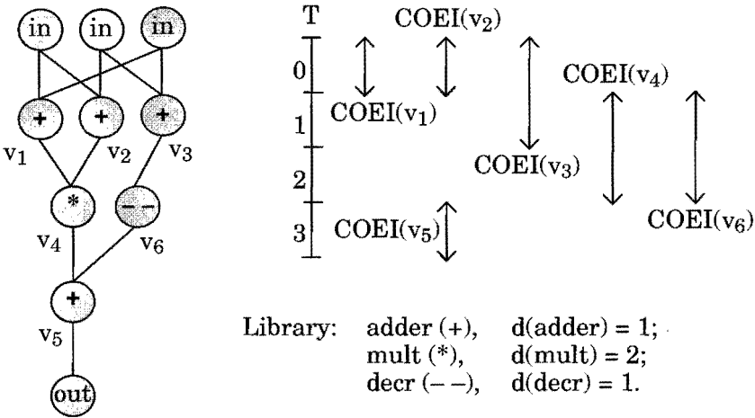
FIGURE 3.1. Example DFG, module library and COEIs.
