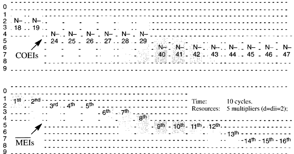
FIGURE 2.4. COEIs & MEIs for the sixteen multiplications of FDCT given in Figure 2.3.
