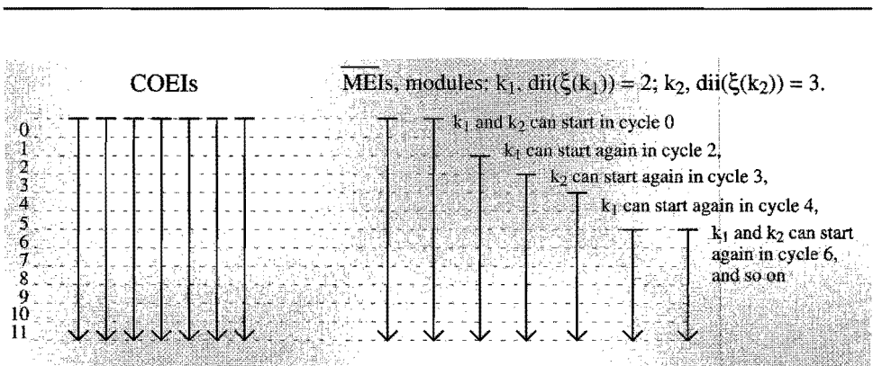
FIGURE 2.9. 1 st example of \overline{\text{MEI}} s with an unrestricted module set.
