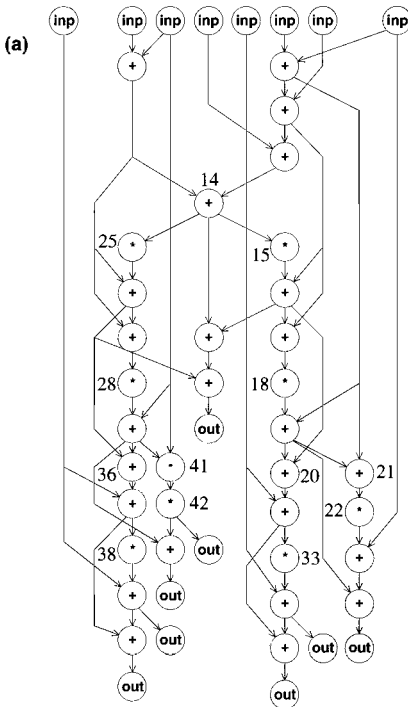
FIGURE 2.5. Fifth order wave digital filter, WDELDF, from [DeWi85].
