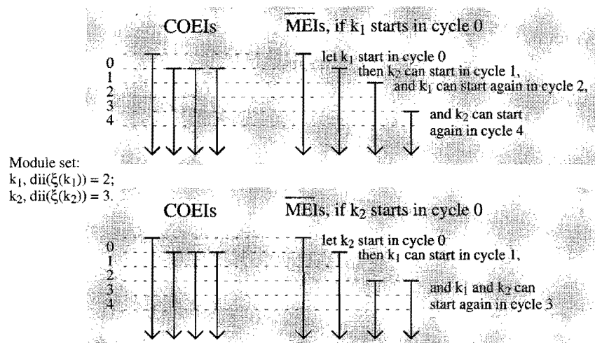
FIGURE 2.10. 2 nd example of \overline{MEI} s with an unrestricted module set.
