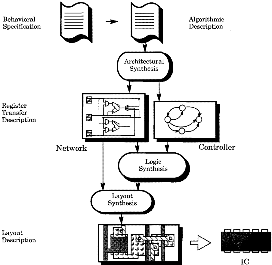
FIGURE 1.1. Computer-aided VLSI design flow, taken from [Stok91].
