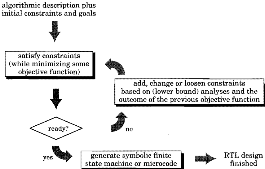
FIGURE 1.2. Design methodology for architectural synthesis.
