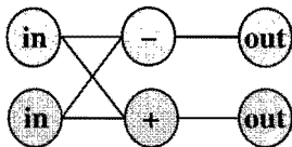
FIGURE 3.3. Example DFG with library.
