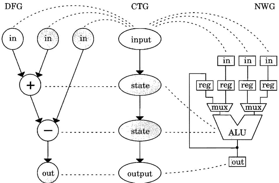
FIGURE 1.5. Simplified example of inter-domain relations.
