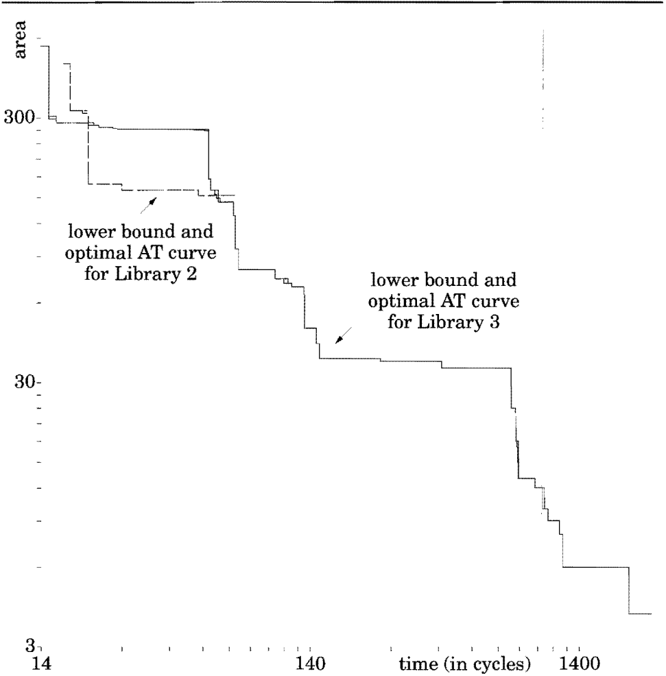
FIGURE 3.6. WDELFF results, Library 2 and 3.
