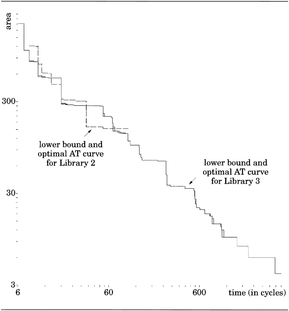
FIGURE 3.7. FDCT results, Library 2 and 3.
