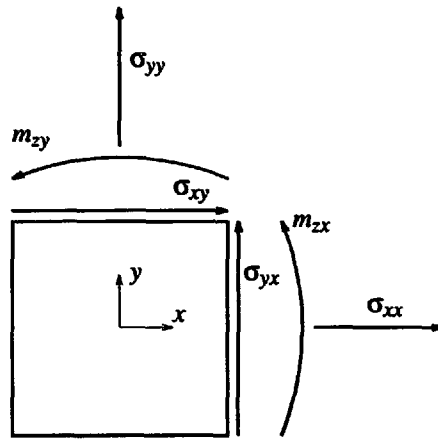
Fig. 1. Stress and couple-stress in a two-dimensional configuration.
