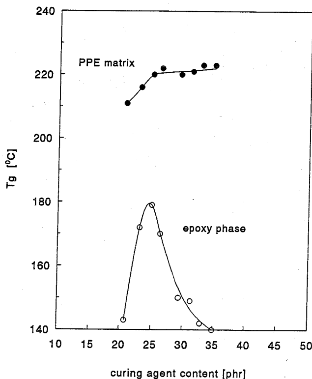
Figure 6 Glass transition temperature versus curing agent concentration of the epoxy and PPE phase, as determined using d.m.t.a. (heating rate = 3^\circ\text{C min}^{-1} , frequency = 1 Hz) for cured blends containing 65 wt% PPE ( 30 \text{ kg mol}^{-1} )
