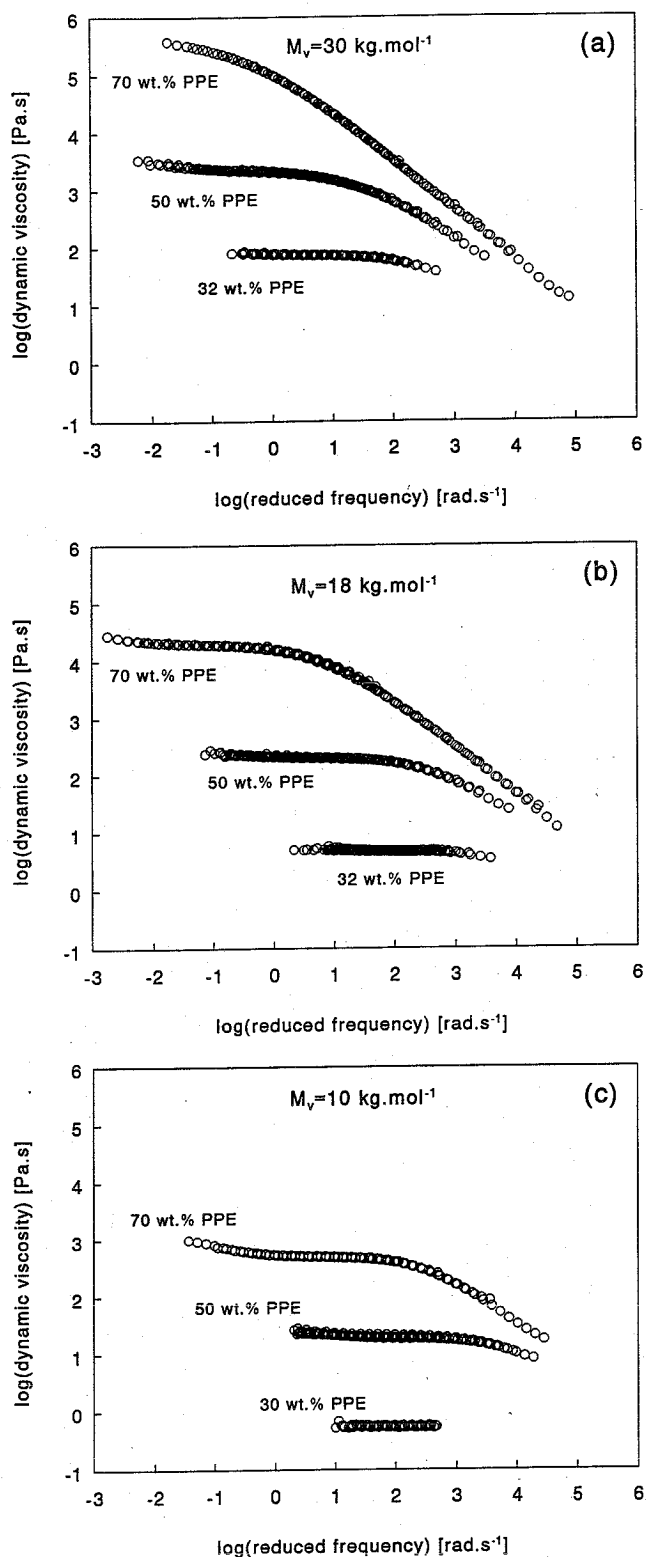
Figure 3 Flow curves of epoxy/PPE solutions varying in PPE content for PPE with different molecular weights: (a) 30 \text{ kg mol}^{-1} ; (b) 18 \text{ kg mol}^{-1} ; (c) 10 \text{ kg mol}^{-1} (reference temperature is 170^\circ\text{C} )
