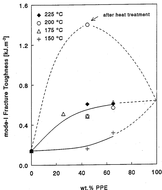
Figure 10 Mode-I fracture toughness ( G_{1c} ) of cured epoxy/PPE blends as a function of PPE content and initial curing temperature for PPE with a molecular weight of 20 \text{ kg mol}^{-1} . The fracture toughness value of a blend containing 45 wt% PPE, which has been heated for 24 h at 200^\circ\text{C} before adding curing agent and curing, is also shown
