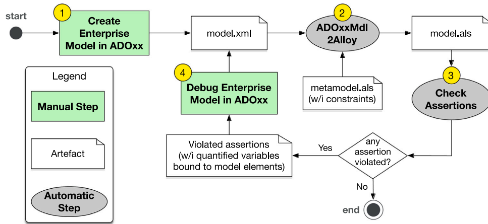
Fig. 4. Chaining ADOxx with Alloy for enterprise models consistency checking.
