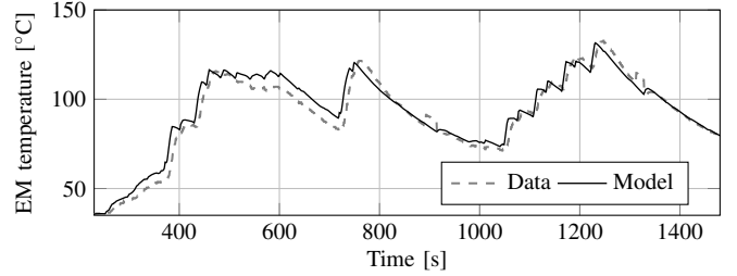
Fig. 8. Comparison between the thermal model and one of the vehicle telemetry data samples. In total, three data sets were used to fit the model parameters, of which the average normalized RMSE was 4.12% w.r.t. the maximum temperature of each data set.
