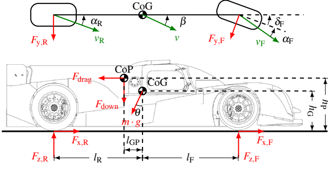
Fig. 4. Top and side view of the single-track vehicle model. The forces acting on the vehicle are shown in red and the velocity vectors are shown in green. The center of gravity (CoG) is shown in both figures, whereas the center of pressure is only shown in the side view. The arrows indicate positive directions, angles or forces.
