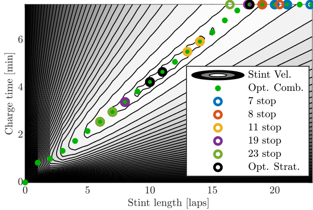
Fig. 18. The average stint velocity for a combination of stint lengths and charge times together with the optimal combinations and actual numerical solutions. The optimal combinations of stint length and charge time show a clear (linear) correlation, to which the numerical solutions are aligned.
