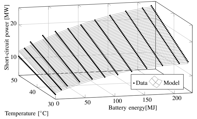
Fig. 9. A temperature- and energy-dependent battery model. The normalized RMSE of the model is 2.23% w.r.t. the maximum short-circuit power.
