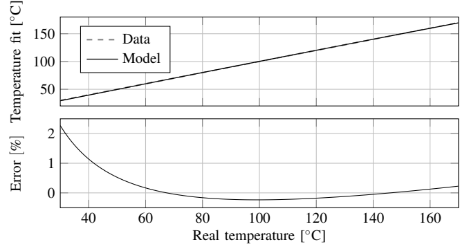
Fig. 7. Semi-definite fit of the EM temperature together with the relative error. The normalized RMSE is 0.15% w.r.t. the maximum temperature.
