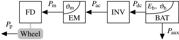
Fig. 5. Schematic layout of the electric race car powertrain topology consisting of a battery (BAT), inverter (INV), electric machine (EM) and final drive (FD). The arrows indicate positive power flows of the auxiliary power P_{aux} , the electrical inverter power P_{dc} , the electrical EM input power P_{ac} and mechanical output power P_m , and the propulsion power P_p .
