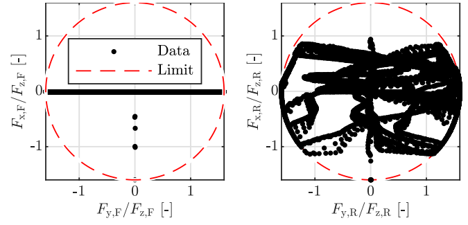
Fig. 15. The friction circles per axle showing the normalized longitudinal and lateral forces. The vehicle is rear-wheel driven and braking is done mostly using the EM. Therefore, the front axle (left figure) mostly generates lateral forces, whereas the rear axle (right figure) shows more combined forces.
