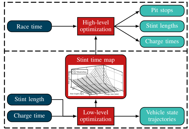
Fig. 3. Block diagram overview of the general approach to optimize the race strategy. The low-level framework provides the state trajectories and minimum stint time for several combinations of stint length and charge time. The high-level framework optimizes the race strategy for a given race time, using the stint time data.
