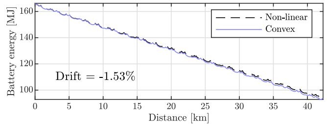
Fig. 19. Battery energy calculated through the non-linear and convex models, using the optimized inputs for the globally optimal stint of 10 laps and 4.2 min charging. The small drift in battery energy between the non-linear and convex models indicate that the convex models accurately capture the dynamics of the powertrain components.
