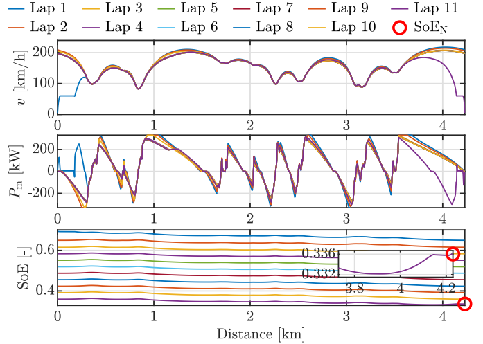
Fig. 13. Velocity, EM power and battery SoE trajectories per lap for an 11 lap stint. The battery energy is an active constraint, thus the stint is energy-limited. The EM power shows a gradual decrease at high velocities, thus indicating energy management. The zoom window corresponds to the final 500 m of the stint.
