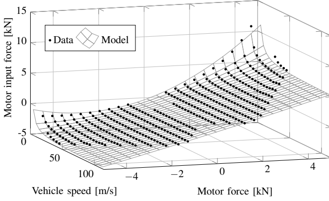
Fig. 6. A speed- and torque-dependent model of the EM. The normalized root-mean-square error (RMSE) of the model is 1.49% w.r.t. the maximum motor input force F_{ac} .
