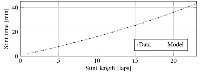
Fig. 12. Fit of the final stint times for a range of stint lengths. The normalized RMSE of the fit is 0.58% w.r.t. the maximum stint time.
