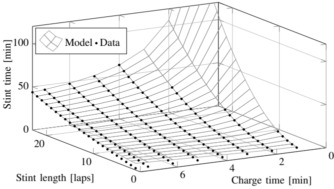
Fig. 11. Fit of optimization results for a combination of stint lengths and charge times. The normalized RMSE of the fit is 2.2% w.r.t. the maximum stint time.
