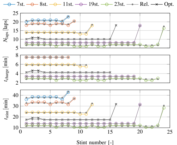
Fig. 17. Optimal race strategy (black) in terms of stint length, charge time and stint time with t_{\text{charge,max}} = 7.5 min. For comparison, we show other optimal fixed pit stops strategies together with the relaxed solution in gray. Stint length, charge- and stint time are related and the optimal integer solution minimizes the differences to the relaxed solution.
