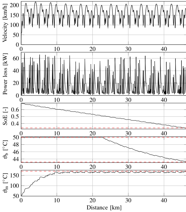
Fig. 14. Velocity, powertrain losses, battery SoE, battery temperature and EM temperature trajectories for an 11 lap stint. The battery energy is an active constraint, thus the stint is energy-limited and energy management is needed. Furthermore, the maximum EM temperature is reached multiple times throughout the stint. Therefore, the velocity profile decreases when the maximum EM temperature is reached.
