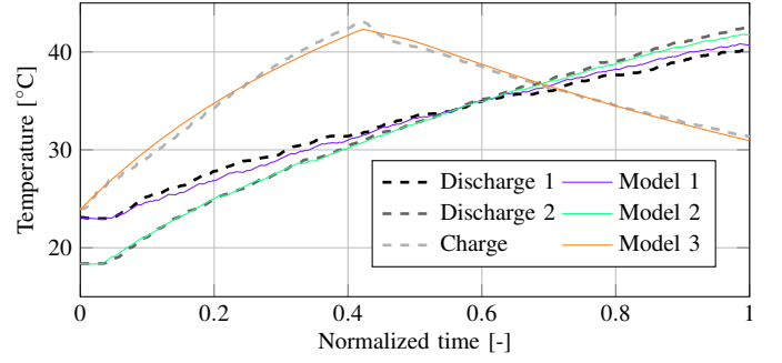
Fig. 10. Comparison between the thermal model and three data sets, of which two represent a dynamic discharge (violet and green) and one represents a constant current charge profile followed by a cooldown period (orange). The average normalized RMSE is 0.87% w.r.t. the maximum temperature of each data set.
