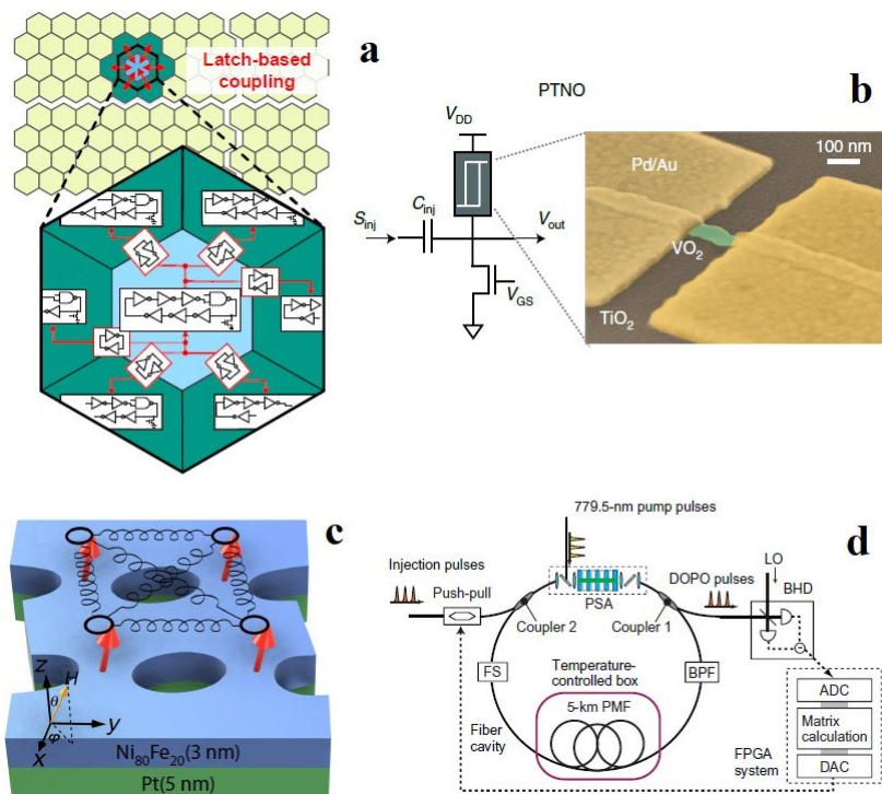
Figure 1. Sketches of different implementations for Ising Machines realized through coupled oscillators of different types: a) Exagonal ring-oscillators [8] b) phase-transition oscillators based on \text{VO}_2 [10] c) nanoconstriction-based spin-Hall nano-oscillators [12] d) optical parametric oscillators [19].
