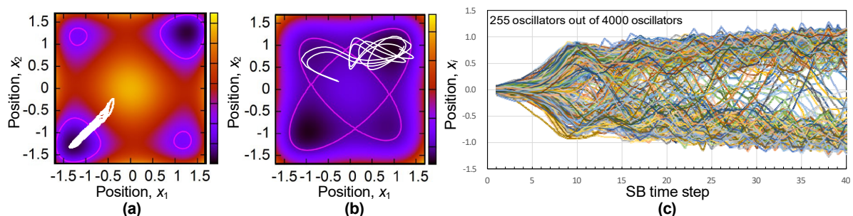
Figure 1. Dynamics in simulated bifurcation. (a) and (b) show trajectories indicating adiabatic and ergodic searches, respectively, for a two-spin problem ( N=2 ) [1]. (c) Time evolution of oscillators exhibiting bifurcations ( N=4000 ) [8].
