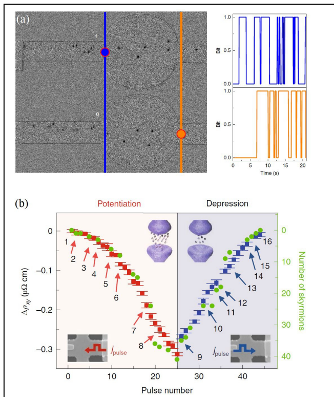
Figure 1. (a) example of a skyrmion reshuffler. Reproduced with permission from Ref. [13]. (b) memristive behavior of skyrmions for synapses applications. Reproduced with permission from Ref. [15].
