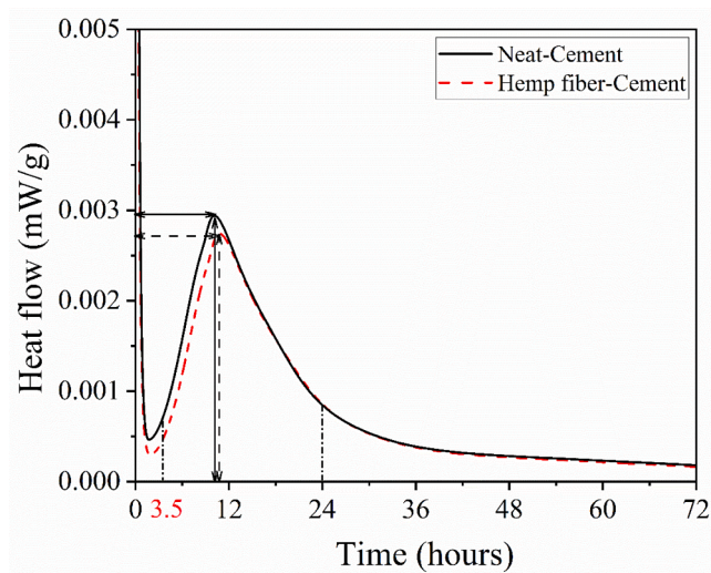
Fig. 9. Heat flow versus time for a typical hemp fiber-cement (dashed curve) and neat-cement (solid curve).
