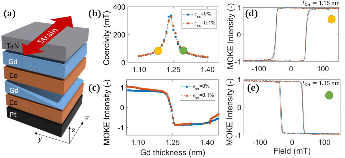
FIG. 3: (a) Layerstack consisting of a Co/Gd quadlayer used to obtain magnetization compensation. (b) Coercivity and (c) remanent pMOKE intensity scan as a function of t_{Gd} . Measurements before (blue) and after (orange) application of in-plane strain are reported. (d) Hysteresis loops in the Co dominated and (e) Gd dominated state. Both curves with (orange) and without (blue) in-plane strain applied are shown.
