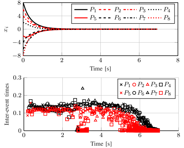
Fig. 3: Evolution of the states (top) and inter-event times (bottom) of the MAS using the dynamic trigger obtained by applying Corollary 1 to Proposition 3 with c_i = 0 and initial condition x(0, 0) = (8, 6, 4, 2, -2, -4, -6, -8) .
