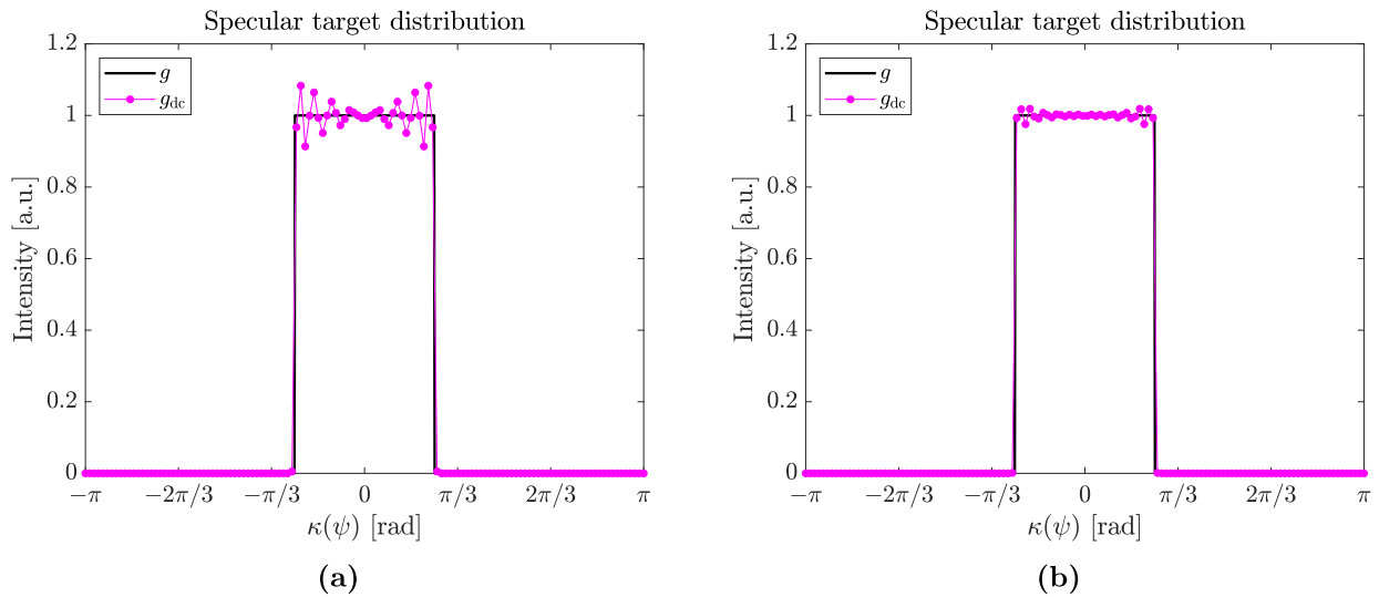
Figure 12. Example #2; deconvolucy deconvolution with 10^2 iterations (a), and 10^4 iterations (b).
