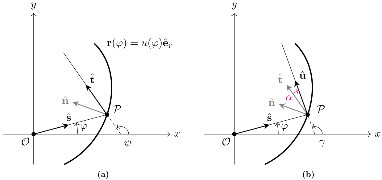
Figure 2. Reflectors exhibiting specular reflection (a), and light scattering (b); line-source along suppressed z -axis passing through \mathcal{O} .
