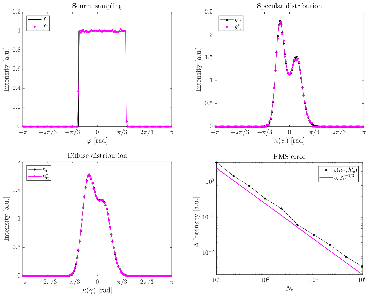
Figure 10. Example #1; raytraced distributions of m_{\text{conv}} reflector with g_{\text{dc}} ; 10^6 rays.
