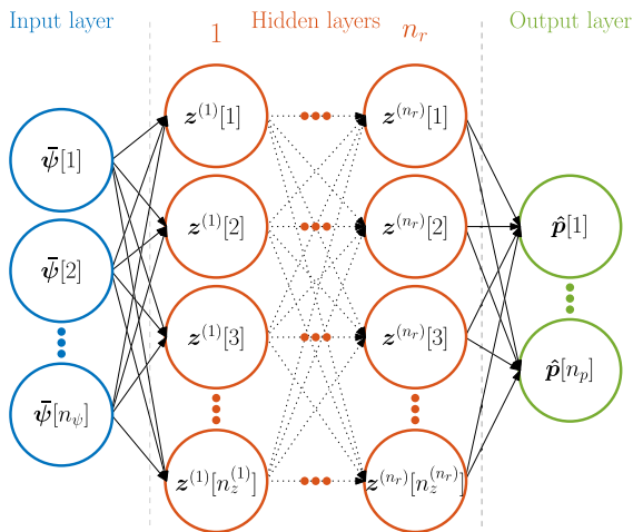
Fig. 1 Structure of a fully connected feed-forward ANN with n_r hidden layers
