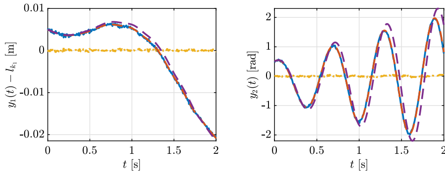
Fig. 14 Comparison of simulated measurement ( — ) and simulation of updated RDB model ( - - ), for different (simulated) experiment (harmonic excitation and deviating initial conditions) than used to update the model. Furthermore, the error
