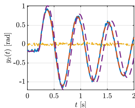
as initial conditions. Furthermore, the error of the updated model (---) is plotted and, for reference, the simulation is performed using the reference model with \mathbf{p} = \mathbf{p}_c (---)
