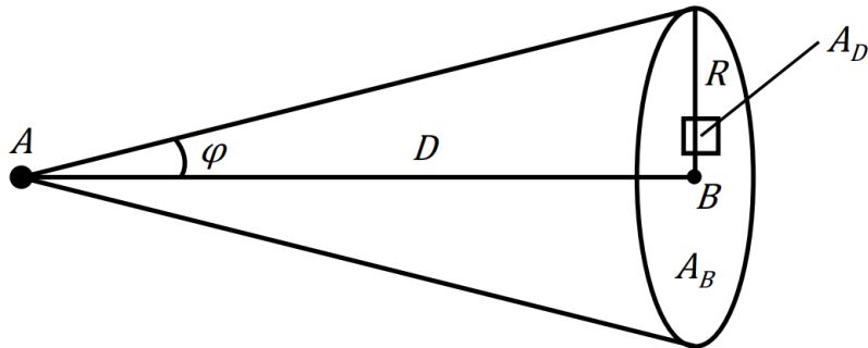
Figure 1. Illustration of propagation of the optical signal
