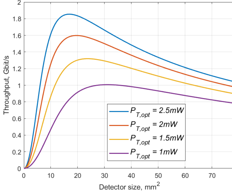
Figure 2. Bit rate of the system that uses the flat frequency response range of the PD as a function of photo-sensitive area
