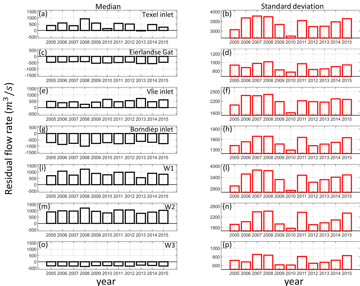
Fig. 6. Median (a, c, e, g, i, m, o) and standard deviation (b, d, f, h, l, n, p) of the residual volume flow in each transect for each year. The residual volume flow is considered positive if it corresponds to an inflow. For the watersheds 1 and 2, we consider these residual flows positive if they are directed towards the tidal basins 2 and 3.
