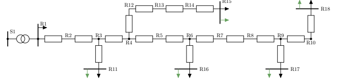
Fig. 2. Residential feeder of the European low voltage CIGRE benchmark grid. Arrows in black represent loads and the arrows in green represent inverters.
