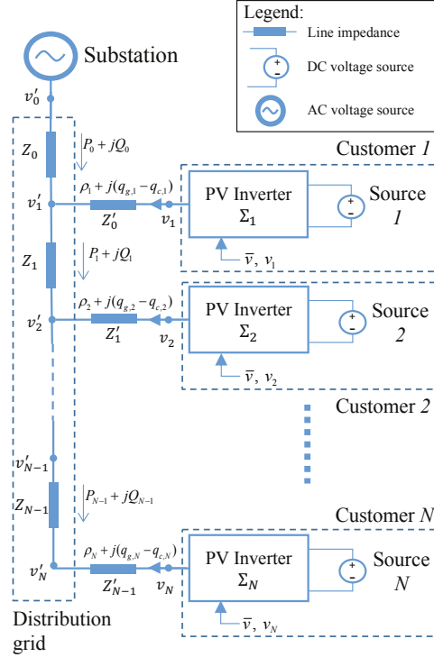
Fig. 1. Infrastructure of the low-voltage distribution grid.
