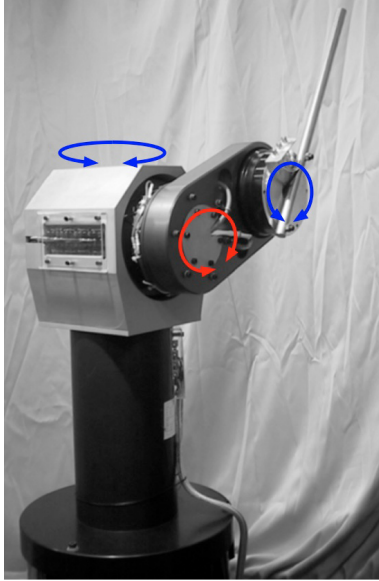
Fig. 4. RRR Robot - 3 rotational DOF robot present at the Department of Mechanical Engineering of the Technische Universiteit Eindhoven. Only the red rotational DOF is considered in this work. Picture from Kostić (2004).
