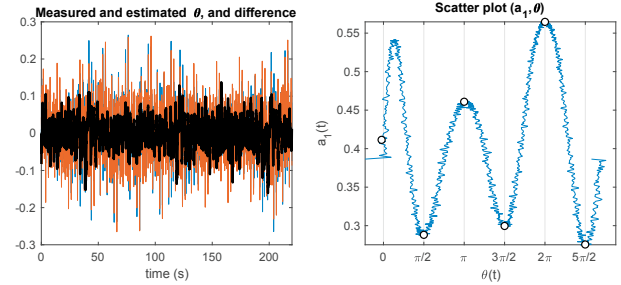
Fig. 5. Left: Measured (orange) and simulated (blue) detrended \theta , and difference (black). Right: Estimated a_1(t) against the measured \theta(t) . This gives an impression of the damping coefficient as a function of the angle.
