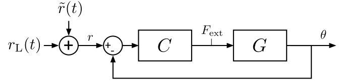
Fig. 2. Stabilising feedback configuration for the simulation example. G is the pendulum in (14), C is a PID controller, \tilde{r}(t) is a small amplitude multisine signal, and r_L(t) is a slowly varying angular setpoint change (ramp).
