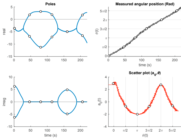
Fig. 6. Left: Time-varying pole-zero map, measurement example. Top-Right: measured angle \theta(t) (black), and estimated trend \theta_L(t) . Bottom-right: visualisation of the dependence of a_0 on the angle \theta . The black circles on all the plots correspond to the angular positions k\frac{\pi}{2} , with k = 0, 1, \dots, 5 .
