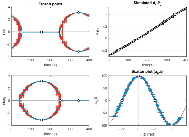
Fig. 3. Identification results on a simulation example. Left: Evolution of frozen poles (top: real part, bottom: imaginary part) (blue: estimated; red: true, locally linearised around \theta(t) ). Top right: Simulated \theta(t) (black) and trend \theta_L(t) . Bottom right: blue: (\hat{a}_0(t), \theta(t)) , red: mg \cos(\theta) . The black circles indicate corresponding points of interest in the four plots.
