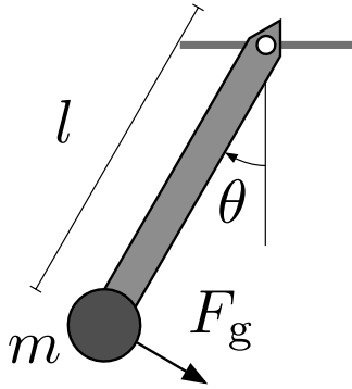
Fig. 1. Simulated pendulum, with massless stiff rod to the extremity of which a mass m is fixed, instantaneous angle \theta , and F_g the component of the gravitational force mg which is perpendicular to the rod.
